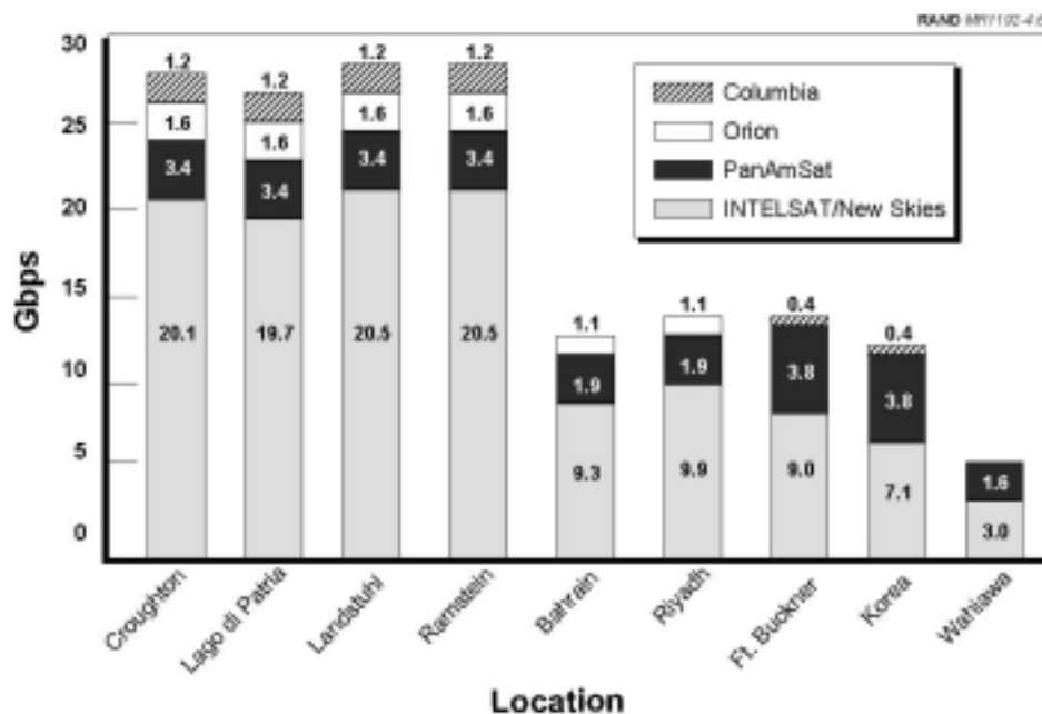
Figure 3 - Maximum International Satellite System Capacity Over DoD STEP Sites 6
