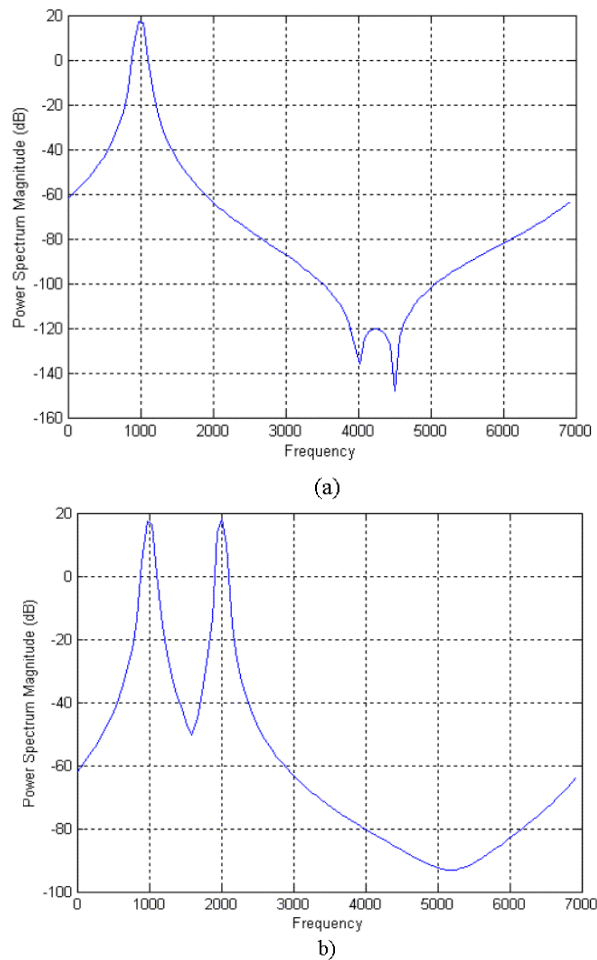
Figure 41 PSD plots for both Test signals: a) 1000Hz single carrier and b) 1 and 2000Hz double carrier, no modulation.
