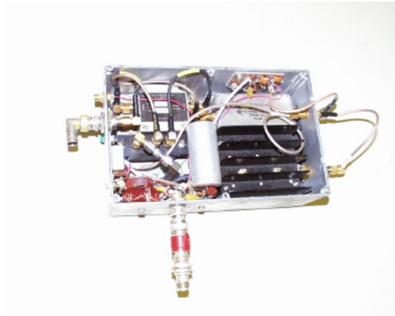
Figure 3.6 Mixer Box
