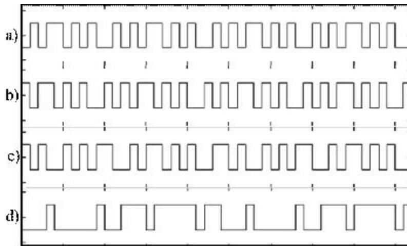
Figure 12. Incorrect Demodulation of Data Signal
