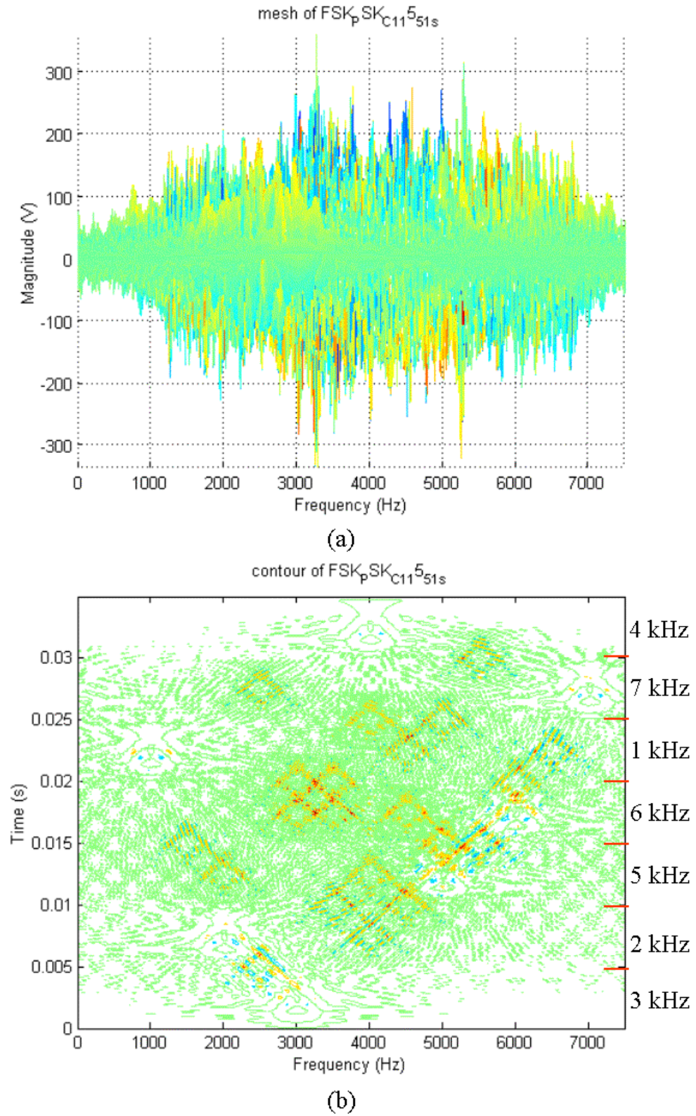
Figure 61. WD for FSK/PSK COSTAS with 5 bit Barker Code, CPP = 1, Signal Only, (No.99) (a) 2D Mesh in Frequency Domain. (b) Contour.
