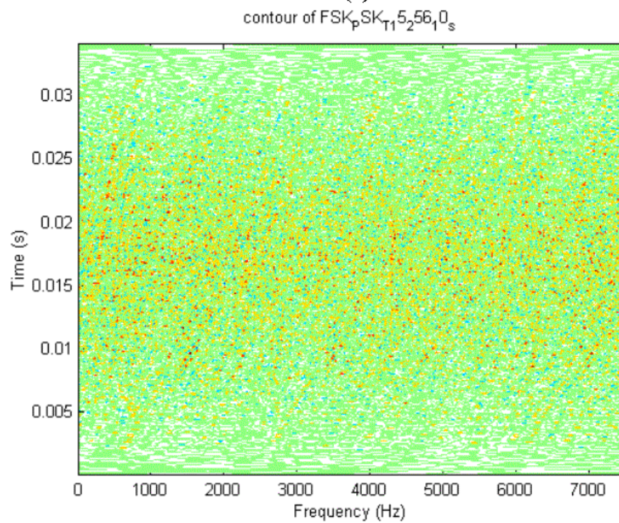
Figure 67. WD for FSK/PSK Target with 256 Random Hops, CPP = 10, Signal Only, (No.111) (a) 2D Mesh in Frequency Domain. (b) Contour.
