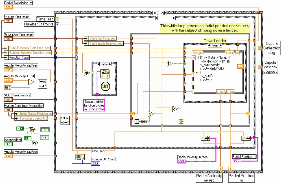
Figure 33: Determination of Subject Radial Velocity when Climbing Down a Ladder
