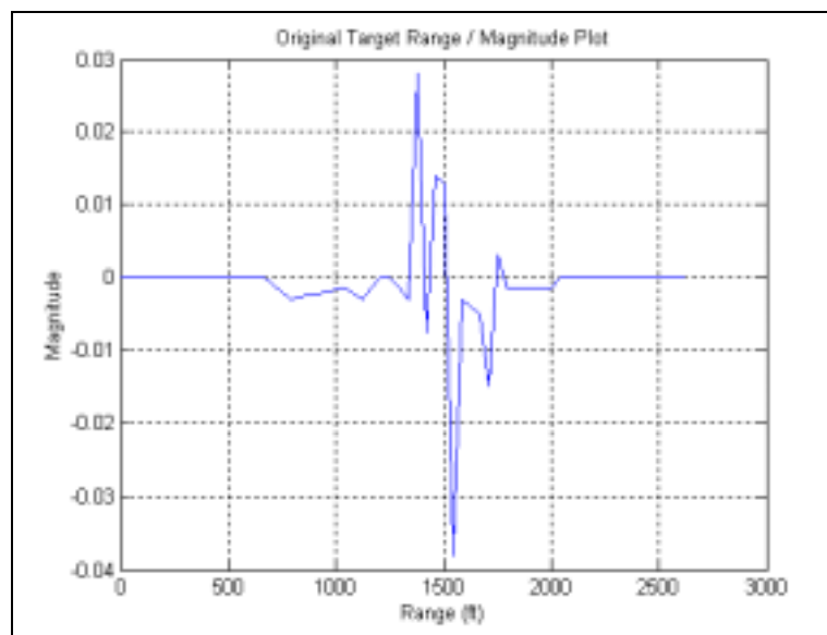
Figure 81 FSK/PSK Target simulated response.
