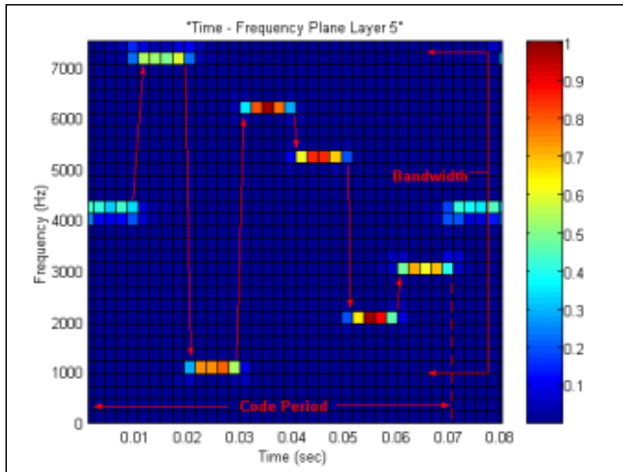
Figure 66 Zoom of output matrix from layer 5 of C_1_15_10_s (colorplot).
