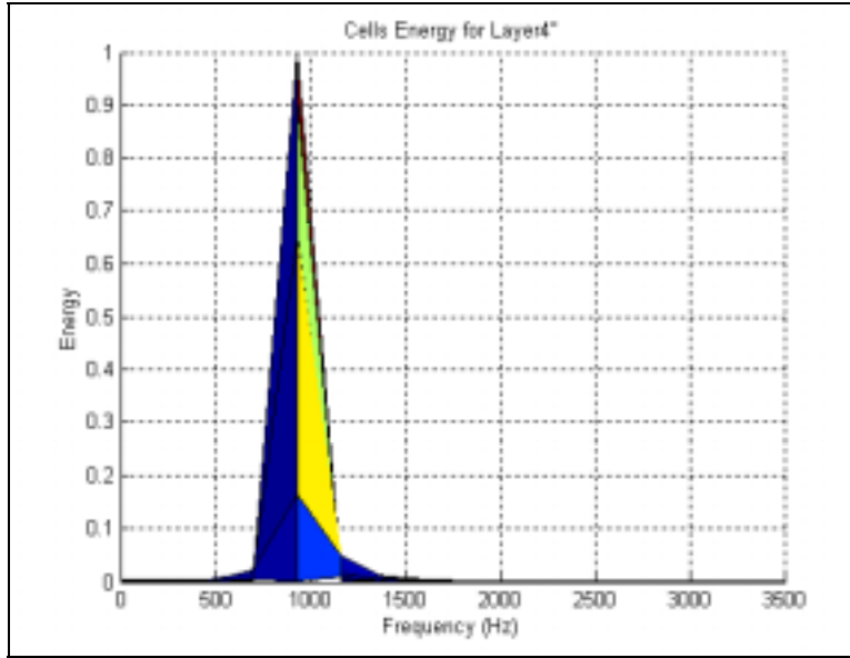
Figure 21 Frequency-energy plot from layer 4 for T_1_7_1_s.
