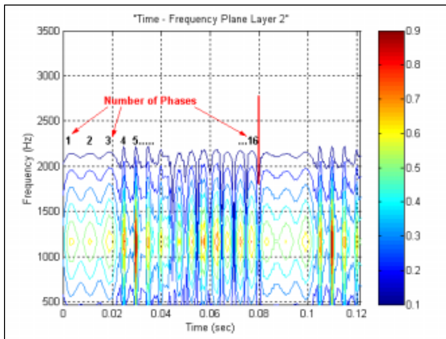
Figure 44 Zoom on output matrix from layer 2 of FR_1_7_4_5_s (contourplot).
