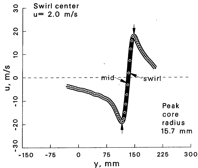
Figure 81: Vortex statistics at \psi = 280^\circ for the +10° vortex generator case.
