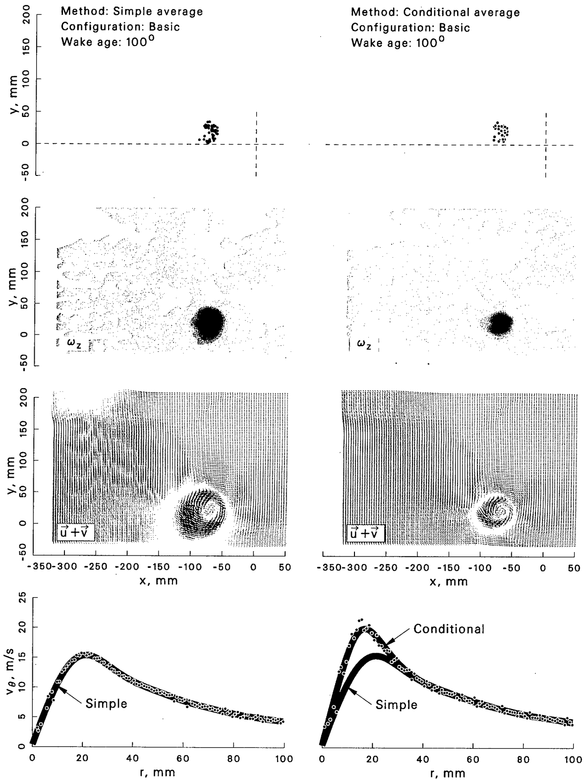
Figure 15: Conditional ensemble average compared to simple average.
