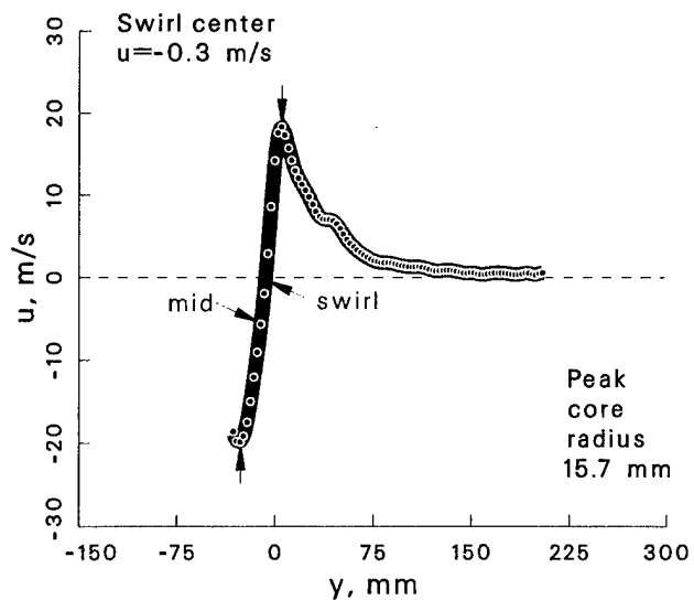
Figure 58: Vortex statistics at \psi = 30^\circ for the +5^\circ vortex generator case.
