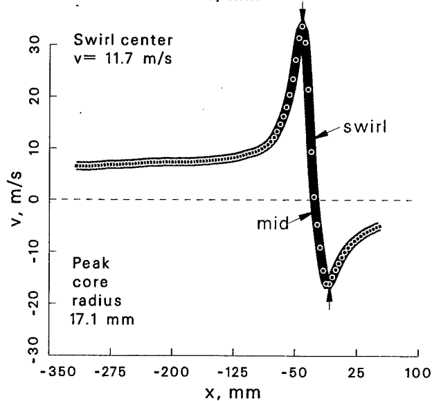
Figure 22: Vortex statistics at \psi = 30^\circ for the basic blade case.
