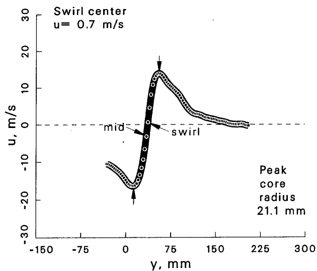
Figure 167: Vortex statistics at \psi = 150^\circ for the free vortex generator case.
