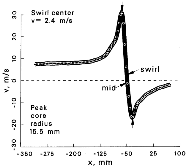
Figure 113: Vortex statistics at \psi = 60^\circ for the -5^\circ vortex generator case.
