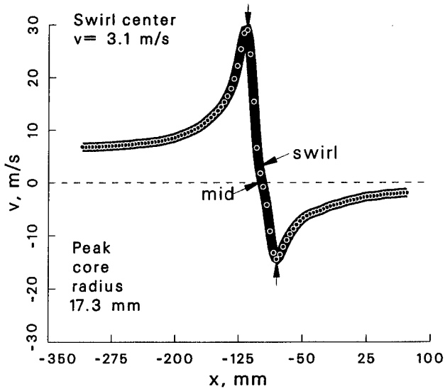
Figure 133: Vortex statistics at \psi = 150^\circ for the -10^\circ vortex generator case.
