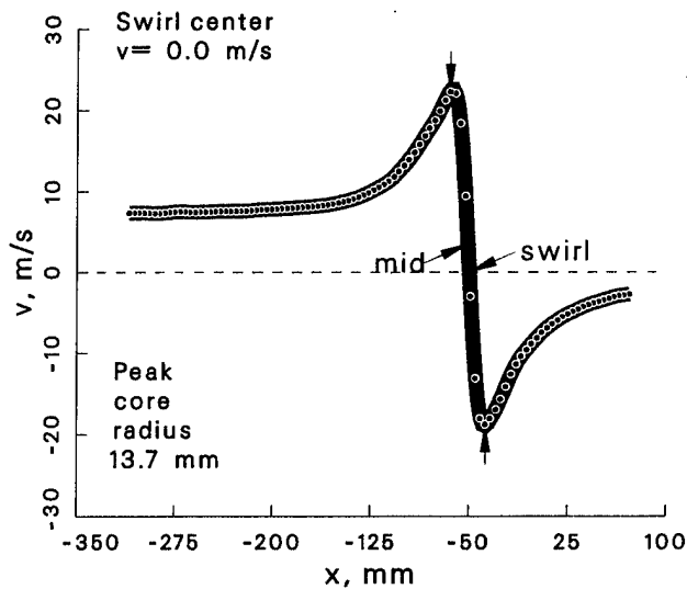
Figure 77: Vortex statistics at \psi = 60^\circ for the +10° vortex generator case.
