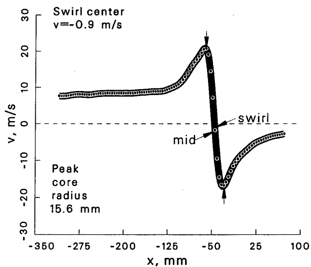
Figure 165: Vortex statistics at \psi = 60^\circ for the free vortex generator case.
