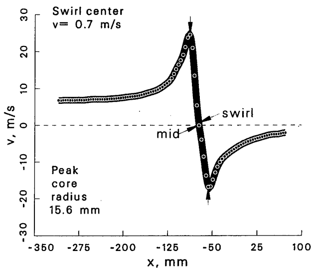
Figure 149: Vortex statistics at \psi = 100^\circ for the -15^\circ vortex generator case.
