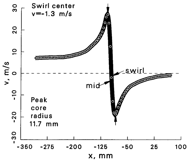
Figure 43: Vortex statistics at \psi = 150^\circ for the 0^\circ vortex generator case.
