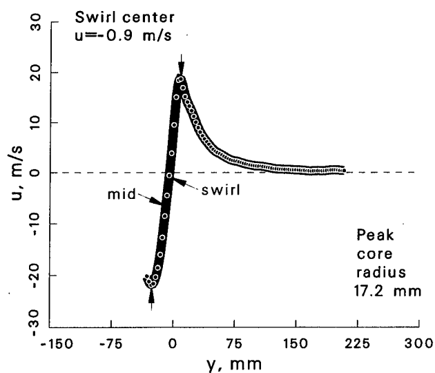
Figure 21: Vortex statistics at \psi = 10^\circ for the basic blade case.
