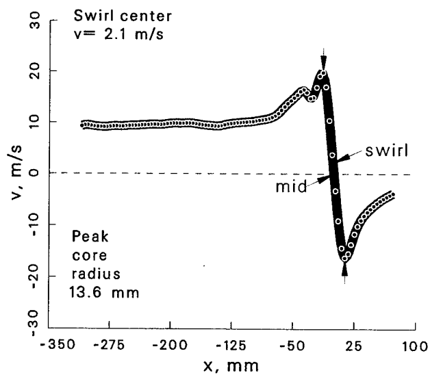
Figure 74: Vortex statistics at \psi = 2^\circ for the +10^\circ vortex generator case.
