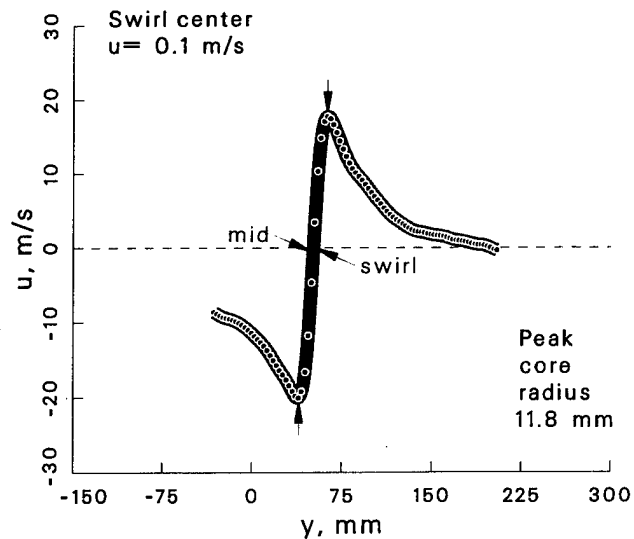
Figure 79: Vortex statistics at \psi = 150^\circ for the +10° vortex generator case.
