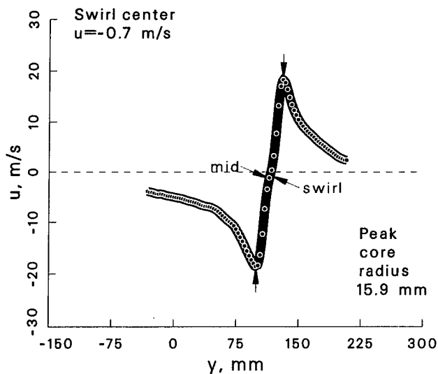
Figure 27: Vortex statistics at \psi = 280^\circ for the basic blade case.
