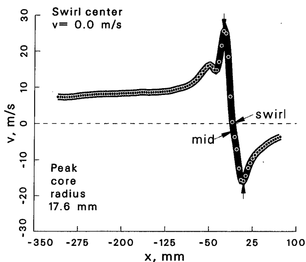
Figure 39: Vortex statistics at \psi = 10^\circ for the 0^\circ vortex generator case.
