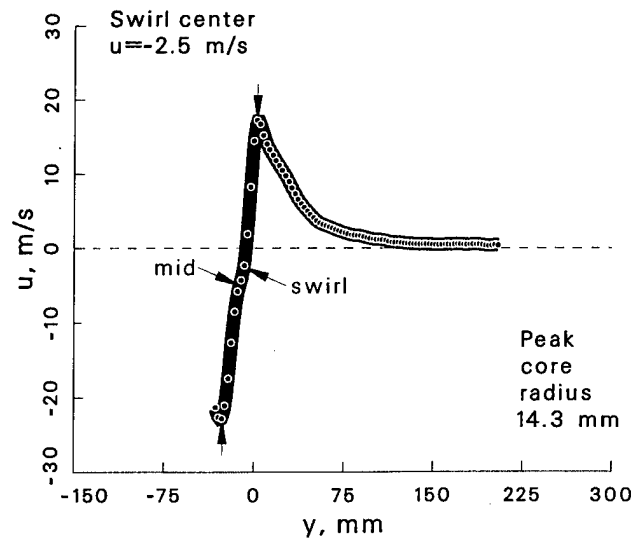
Figure 111: Vortex statistics at \psi = 10^\circ for the -5^\circ vortex generator case.
