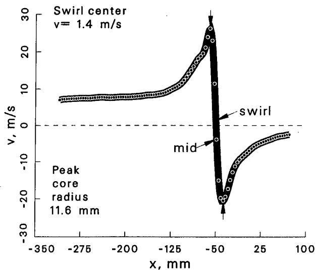
Figure 41: Vortex statistics at \psi = 60^\circ for the 0^\circ vortex generator case.
