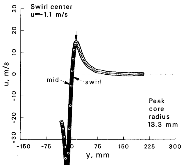
Figure 20: Vortex statistics at \psi = 2^\circ for the basic blade case.
