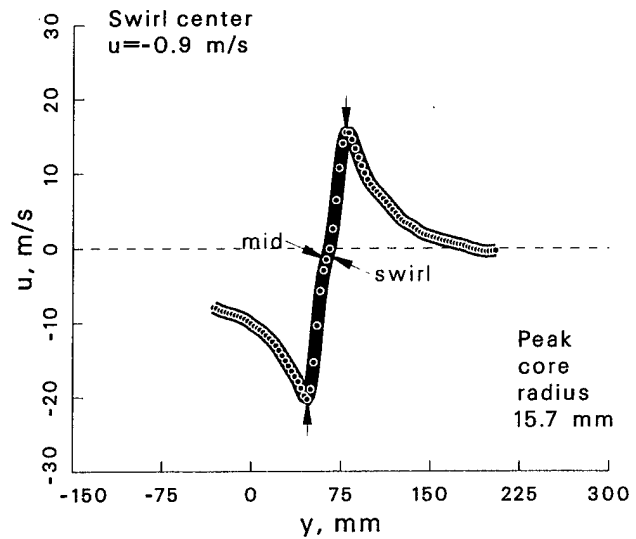
Figure 151: Vortex statistics at \psi = 210^\circ for the -15^\circ vortex generator case.
