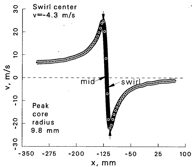
Figure 62: Vortex statistics at \psi = 210^\circ for the +5^\circ vortex generator case.
