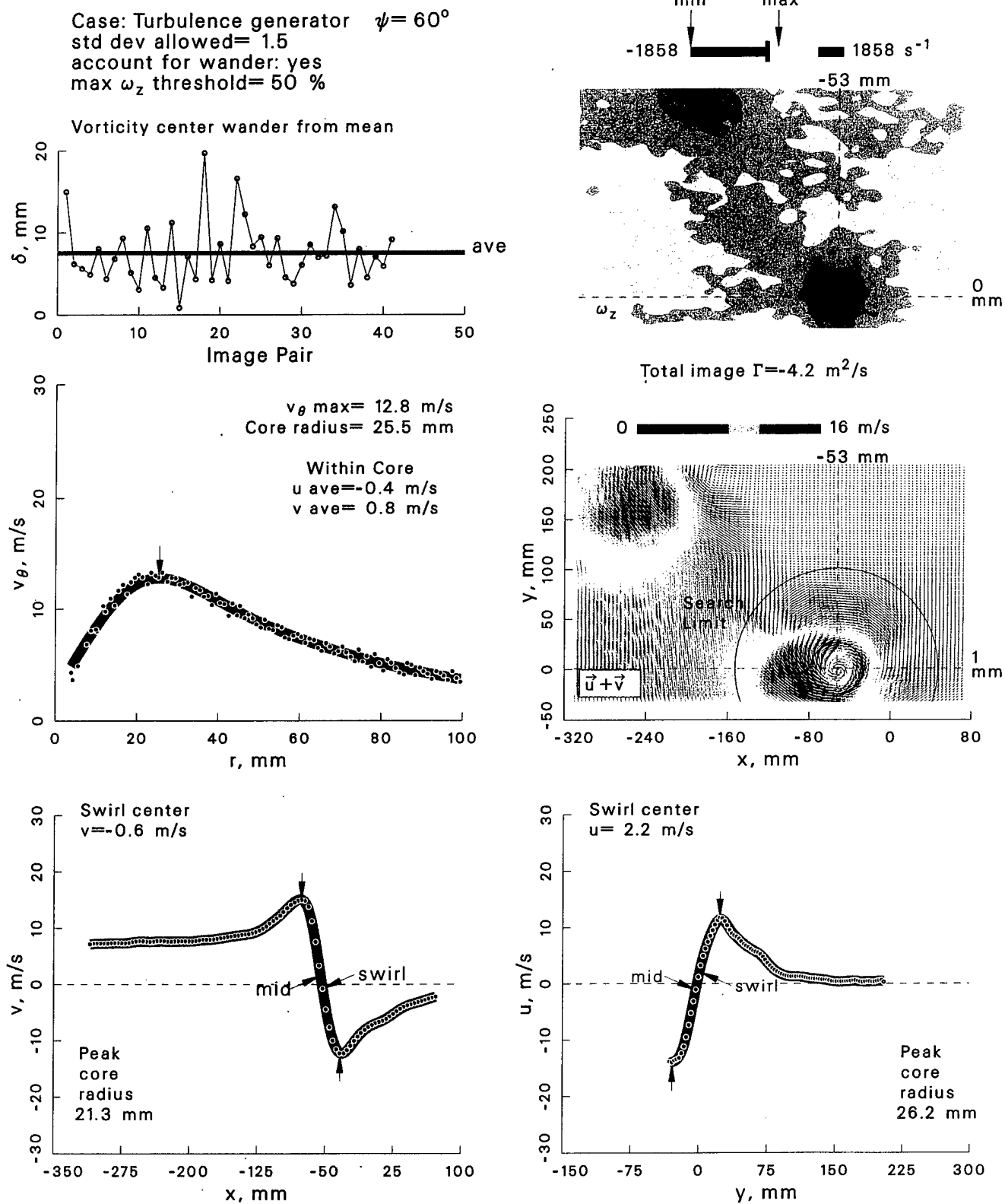
Figure 183: Vortex statistics at \psi = 60^\circ for the turbulence generator case.
