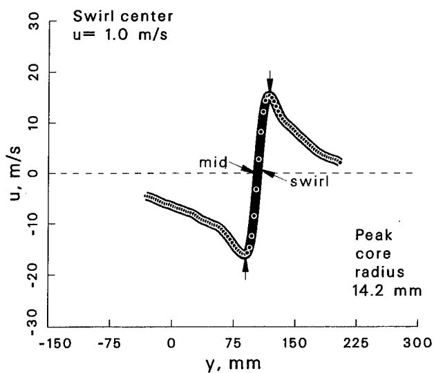
Figure 169: Vortex statistics at \psi = 280^\circ for the free vortex generator case.
