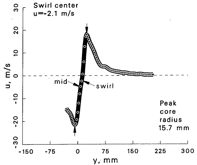
Figure 113: Vortex statistics at \psi = 60^\circ for the -5^\circ vortex generator case.
