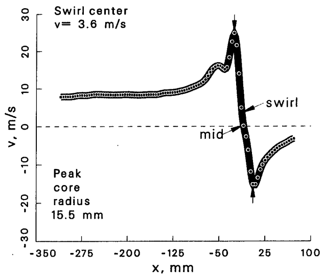
Figure 57: Vortex statistics at \psi = 10^\circ for the +5^\circ vortex generator case.
