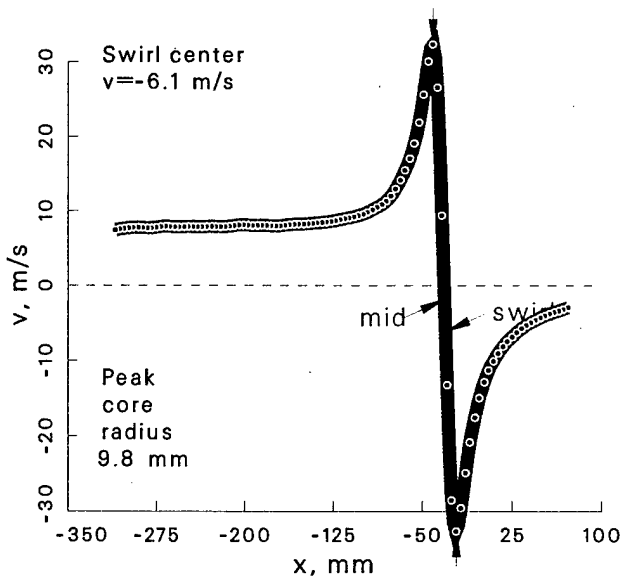
Figure 148: Vortex statistics at \psi = 30^\circ for the -15^\circ vortex generator case.
