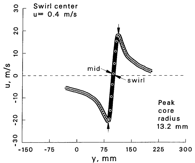
Figure 45: Vortex statistics at \psi = 280^\circ for the 0^\circ vortex generator case.
