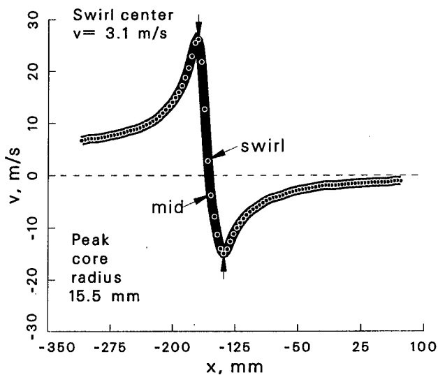
Figure 135: Vortex statistics at \psi = 280^\circ for the -10^\circ vortex generator case.
