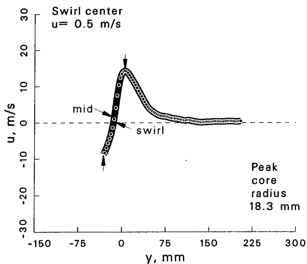
Figure 163: Vortex statistics at \psi = 10^\circ for the free vortex generator case.
