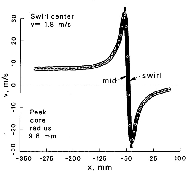
Figure 131: Vortex statistics at \psi = 60^\circ for the -10^\circ vortex generator case.
