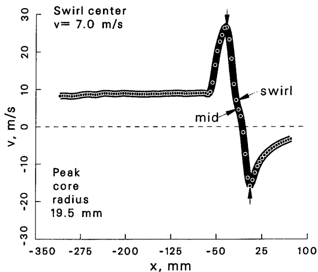
Figure 147: Vortex statistics at \psi = 10^\circ for the -15^\circ vortex generator case.
