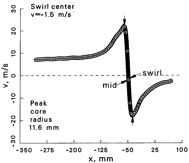
Figure 95: Vortex statistics at \psi = 60^\circ for the +15° vortex generator case.
