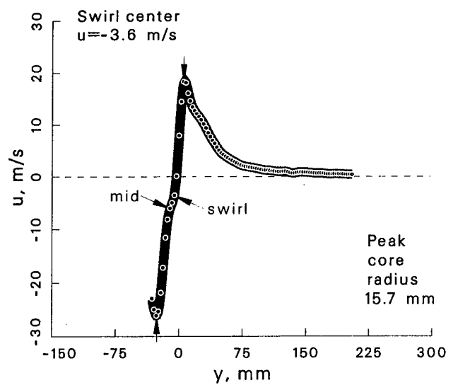
Figure 129: Vortex statistics at \psi = 10^\circ for the -10^\circ vortex generator case.
