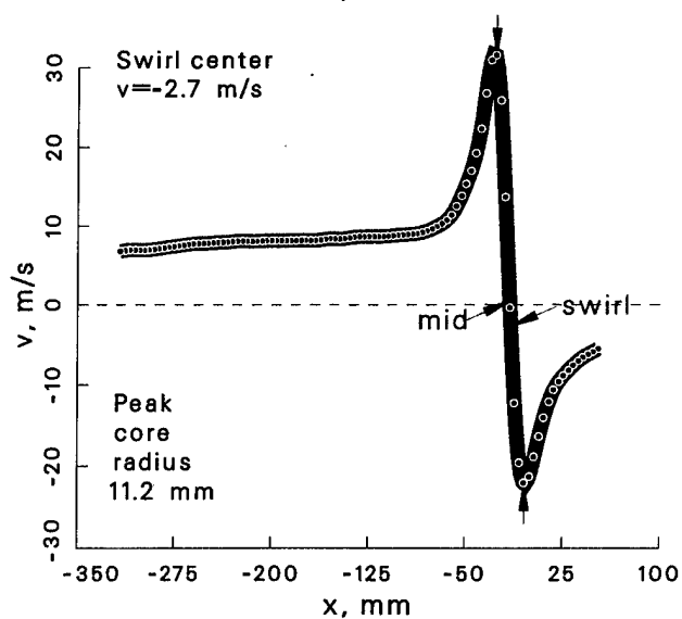
Figure 21: Vortex statistics at \psi = 10^\circ for the basic blade case.
