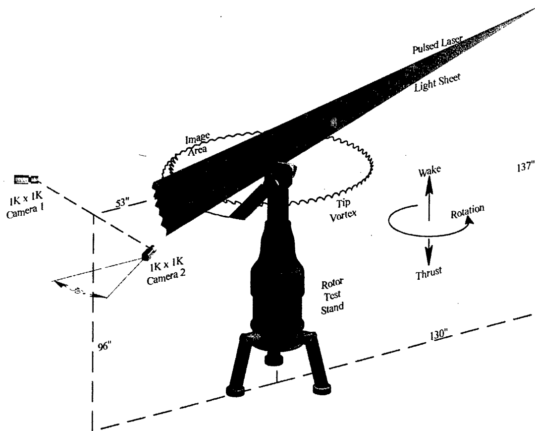
Figure 6: Setup of light sheet and cameras relative to rotor.
