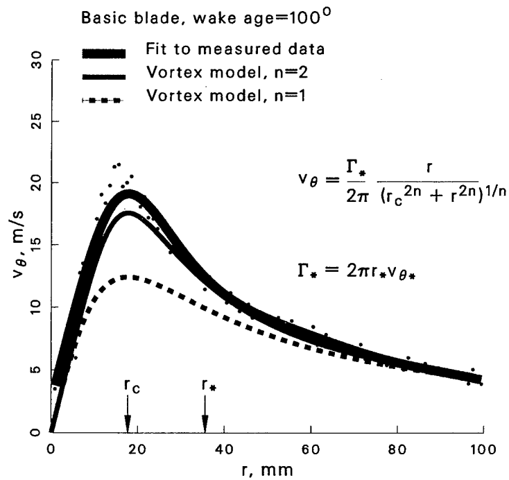
Figure 18: Comparison with algebraic models of vortex.
