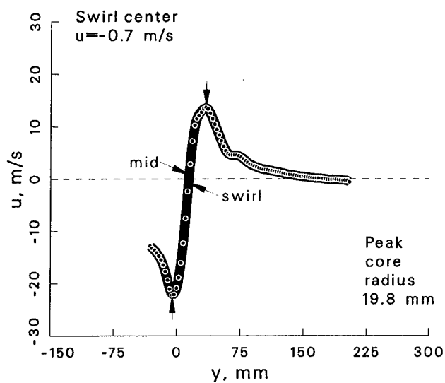
Figure 131: Vortex statistics at \psi = 60^\circ for the -10^\circ vortex generator case.
