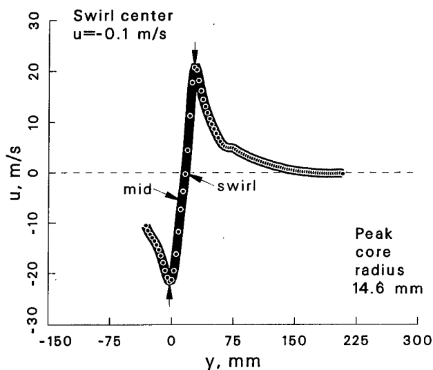
Figure 23: Vortex statistics at \psi = 60^\circ for the basic blade case.
