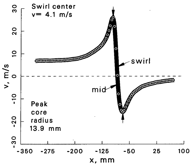
Figure 61: Vortex statistics at \psi = 150^\circ for the +5^\circ vortex generator case.
