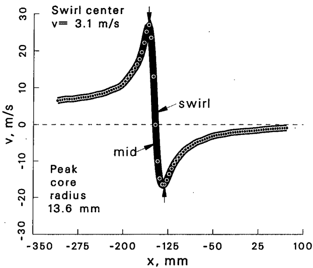
Figure 45: Vortex statistics at \psi = 280^\circ for the 0^\circ vortex generator case.
