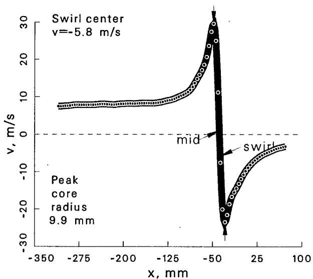
Figure 40: Vortex statistics at \psi = 30^\circ for the 0^\circ vortex generator case.
