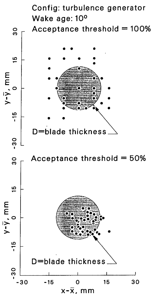
Figure 12: Effect of vorticity acceptance threshold on apparent vortex wander.
