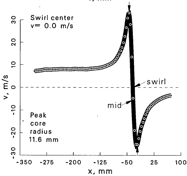
Figure 130: Vortex statistics at \psi = 30^\circ for the -10^\circ vortex generator case.
