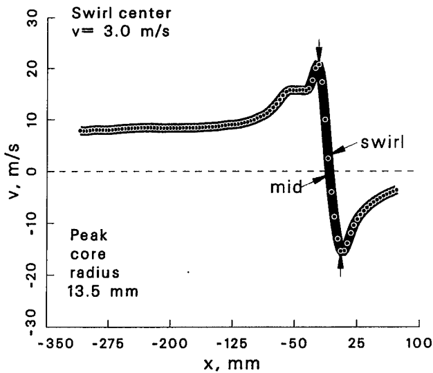
Figure 75: Vortex statistics at \psi = 10^\circ for the +10^\circ vortex generator case.
