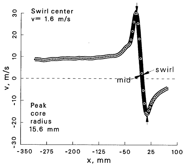
Figure 110: Vortex statistics at \psi = 2^\circ for the -5^\circ vortex generator case.
