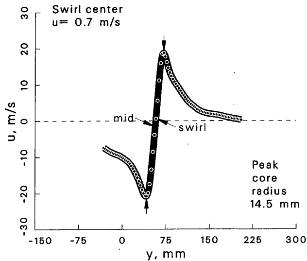
Figure 115: Vortex statistics at \psi = 150^\circ for the -5^\circ vortex generator case.
