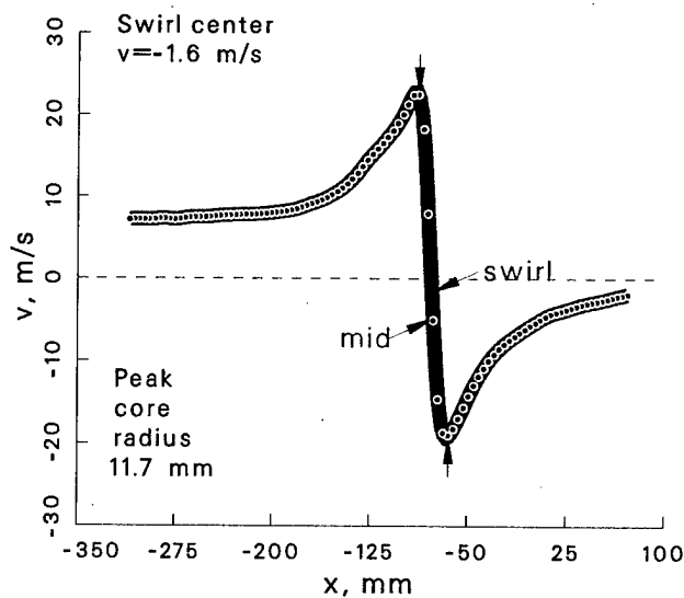
Figure 78: Vortex statistics at \psi = 100^\circ for the +10° vortex generator case.
