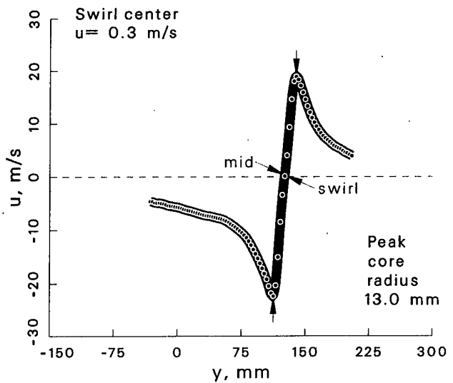
Figure 63: Vortex statistics at \psi = 280^\circ for the +5° vortex generator case.
