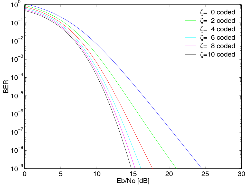
Figure 34. Performance of 16QAM with HDD ( r = 1/2 ) over Ricean Fading
