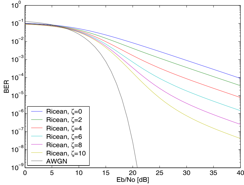
Figure 21. 64QAM performance in Ricean fading channels with 0 \leq \zeta \leq 10
