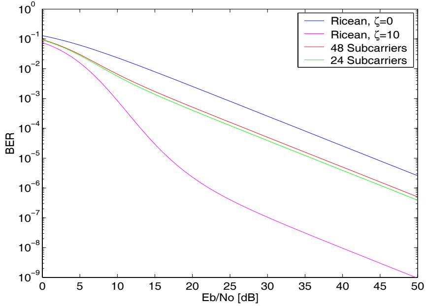
Figure 22. BPSK/QPSK modulated OFDM in composite Rayleigh/Ricean fading channels
