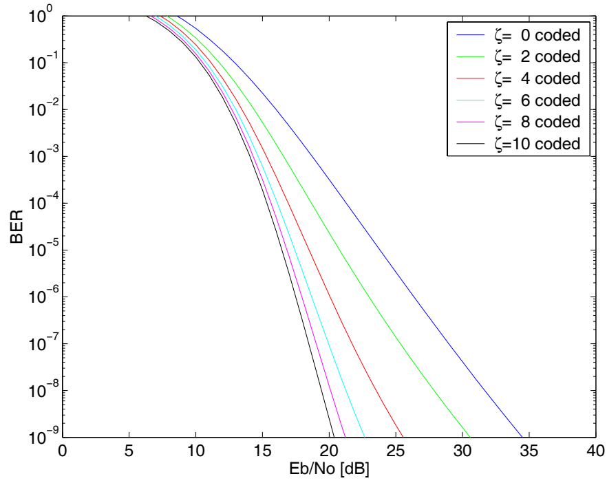
Figure 42. Performance of 64QAM with HDD ( r = 2/3 ) over Ricean Fading
