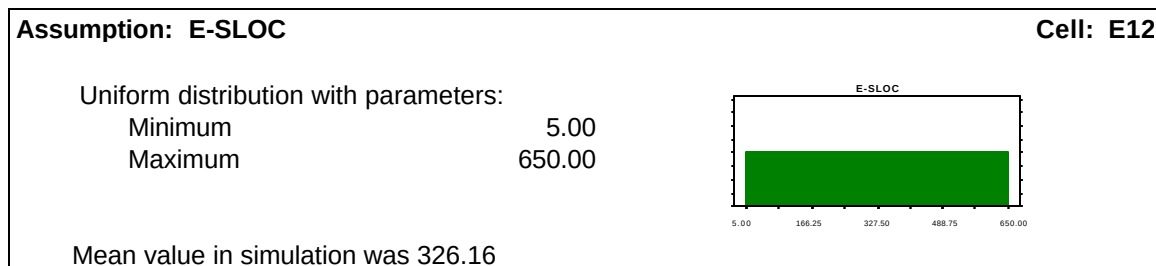
Figure 19 E-SLOC Distribution.
