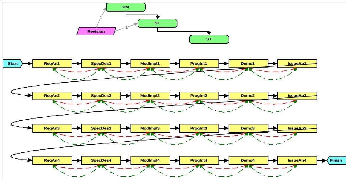
Figure 9 Organization Representation for VitéProject².
