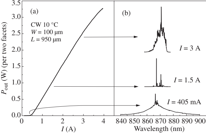
Fig. 2. (a) Light output power ( P_{out} ) dependence on continuous wave (CW) drive current per both facets at heat sink temperature of 10 °C; (b) lasing spectra recorded at corresponding current.
