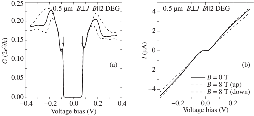
Fig. 3. Differential conductance of the samples with lithographic width 0.5 \mu m , solid curve—without magnetic field, dotted and dashed curve—in the magnetic field 8 T (a). Current-voltage characteristics for the samples with lithographic width 0.5 \mu m , solid curve—without magnetic field, dotted and dashed curve—in the magnetic field 8 T (b). For the dashed curves magnetic field is oriented in the 2DEG plane and normal to the wire, whereas for the dotted curves the direction of magnetic field was reversed.
