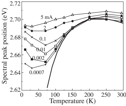
Fig. 2. EL spectral peak position of blue InGaN SQW LED at different current [13]. Thick curve is calculated according to Eq. (2). Fitting parameter s is 31.5 meV.
