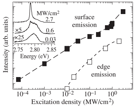
Fig. 4. Surface and edge emission of a stacked SML-CdSe structure with ZnMgSSe barriers as a function of the excitation density. The spectra are vertically displaced for clarity. The super-linear growth and the narrowing of the surface emission occurs, when edge emission saturates. The inset shows the surface emission.
