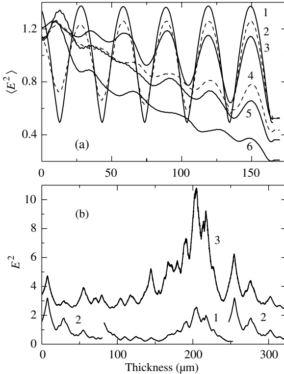
Fig. 1. Electric field intensity profiles for the frequency \nu_0 = 0.596 in the passband. (a) Averaged over 200 random configurations. The standard deviation \delta of the spheres diameter is 1—0%, 2—0.5%, 3—1%, 4—3%, 5—4%, 6—6%. (b) For a single configuration of disorder of \delta = 20\% . Curve 3 corresponds to the structure of 330 \mu\text{m} thickness combined from the structure 1 of 165 \mu\text{m} thickness at the center and two structures 2 of 82.5 \mu\text{m} stacked to it from both sides.
