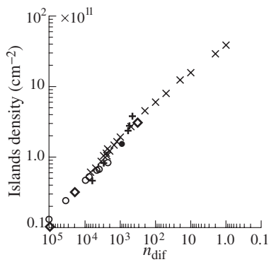
Fig. 1. Islands density dependence on model parameter n_{dif} ( \times \circ ) simulation results; ( \diamond ) experimental data from islands density dependence on temperature; ( + ) on flux intensity [5]; ( \bullet ) experimental point from work [6].
