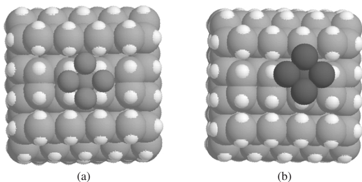
Fig. 1. Top view on the equilibrated supercluster simulating the Si(001)(2x1)-H surface. Tip in position (a) and (b) is placed 5 Å above the top silicon atoms.
