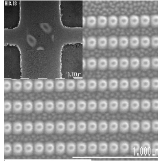
Fig. 1. SEM microphotography array of magnetic nanoparticles, top view. On an insert in the upper left corner of the figure array of magnetic nanoparticles with rectangular lattice on the Hall magnetometer (are seen Moiré patterns between a lattice and raster of SEM).
