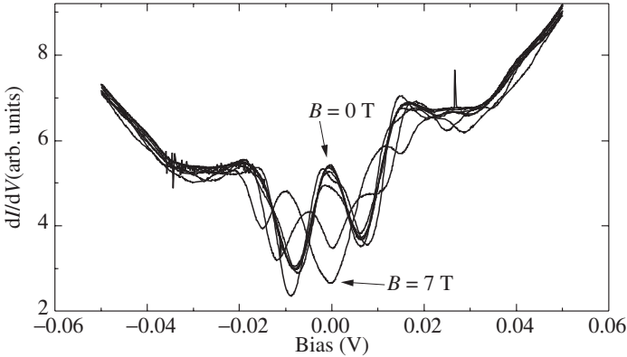
Fig. 2. The tunneling differential conductance as a function of external voltage in different magnetic fields up to 7 T. Magnetic field step between the curves is 1 T.
