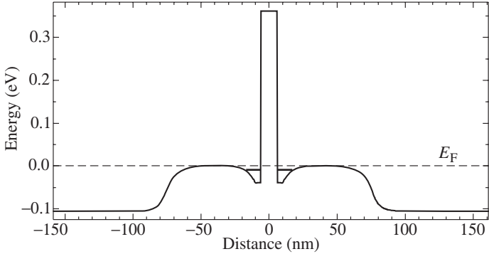
Fig. 1. Schematic band diagram of the structure at zero bias.
