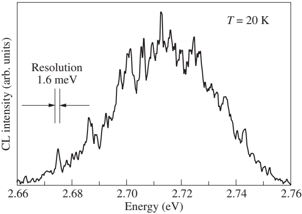
Fig. 2. Cathodoluminescence (CL) spectra of single 1 ML CdSe insertion in a ZnSSe at T = 20 K. The sharp luminescence lines in the spectra originate from single QDs.
