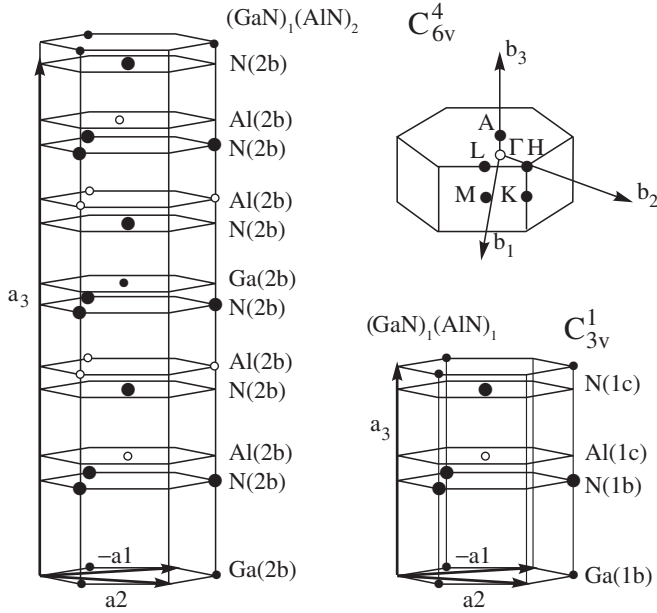
Fig. 1. The primitive unit cells of the (\text{GaN})_1(\text{AlN})_1 and (\text{GaN})_1(\text{AlN})_2 [0001] SLs and the corresponding BZ. The Wyckoff positions are given in parentheses together with the atoms.
