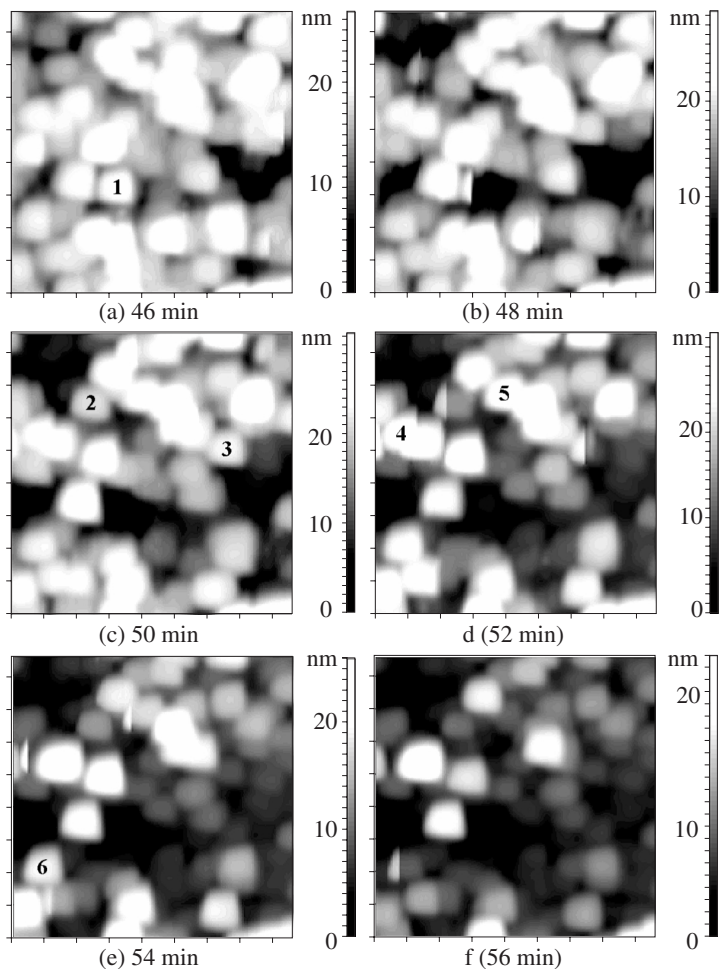
Fig. 1. The series of the AFM images shows the transformation of the same area (860×860 nm) of SiO 2 with αFe nanoparticles during the chemical etching, when the tip apex are pushing out some of the protrusions corresponding to the nanoparticles (with numbers 1–6). In brackets there was indicated the time from start of the chemical etching process.
