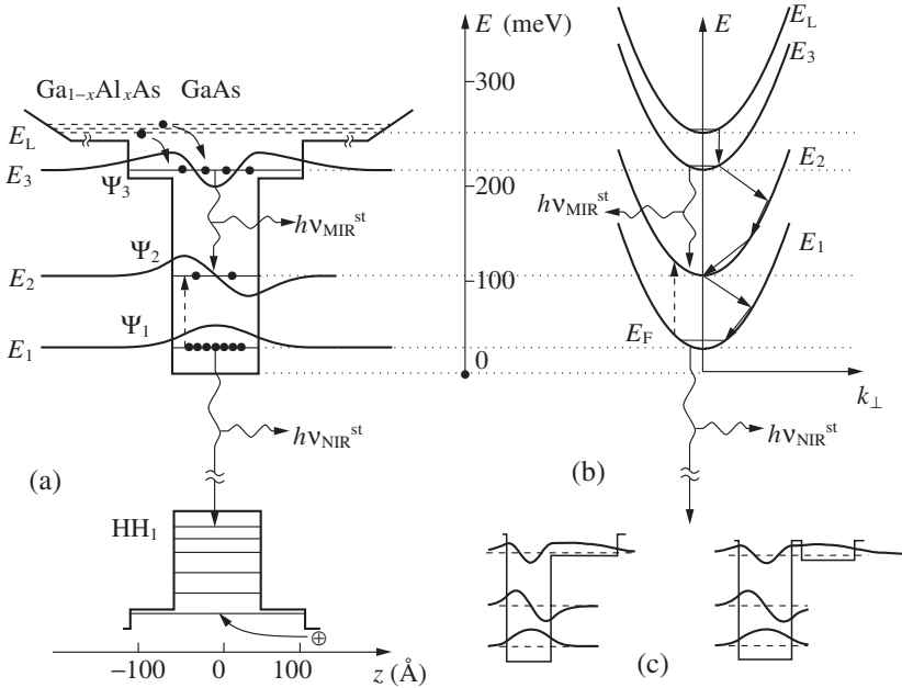
Fig. 1. (a) The diagram of electron transitions in quantum well placed in i-layer of laser n^+ \text{-i-p}^+ heterostructure, energy levels E_i and electron wavefunctions. (b) The diagram of main inter- and intrasubband electron transitions with emission of optical phonons. (c) The profile of QW providing minimal overlapping the electron wavefunctions, belonging to the upper and two lower levels.
