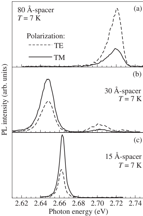
Fig. 3. Linearly polarized photoluminescence (PL) of structures with 80 Å, 30 Å and 15 Å spacers measured in edge geometry. The polarization changes from mostly TE for uncoupled islands (80 Å spacers) to mostly TM (accompanied by a red shift) for vertically coupled islands (15 Å spacers). The 30 Å spacer sample shows emission from both types of islands.
