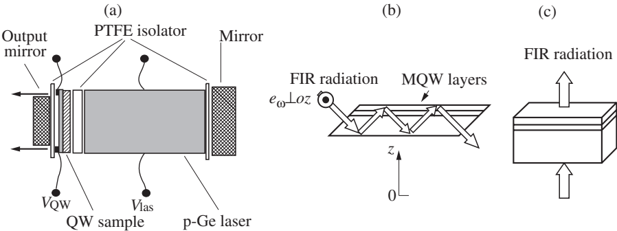
Fig. 1. Diagrams of experimental technique: intracavity measurements (a), total internal reflection geometry (b), traditional geometry (c).
