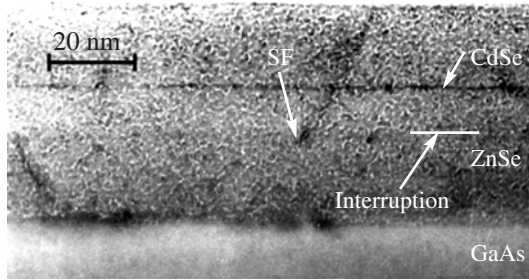
Fig. 1. TEM cross-sectional image of a ZnSe/CdSe/ZnSe structure.
