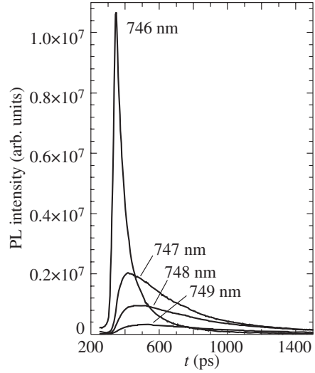
Fig. 2. Time-resolved PL spectra at different detection energies of excitonic band ( \lambda_{\text{exc}} = 746 \text{ nm} )
