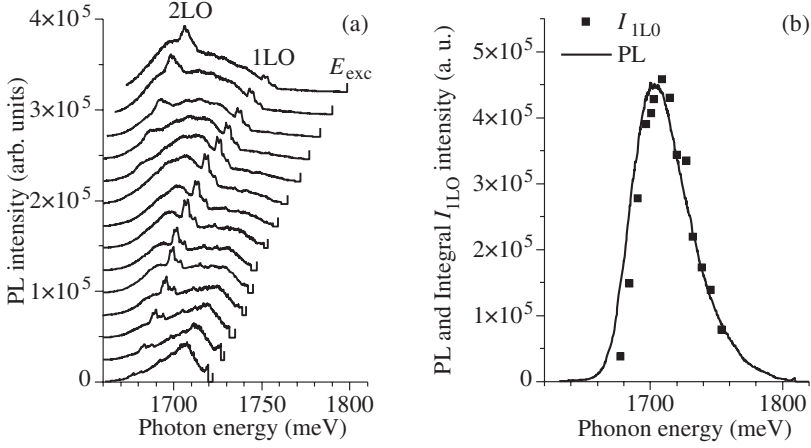
Fig. 2. (a) Dependence of the PL spectra on the excitation energy E_{\text{exc}} . U_{\text{bias}} = -0.8 V. (b) The spectral dependences of the QDs PL under high E_{\text{exc}} and zero bias (solid line) and the integral intensity I_{\text{LO}} of the 1LO resonance (solid squares).
