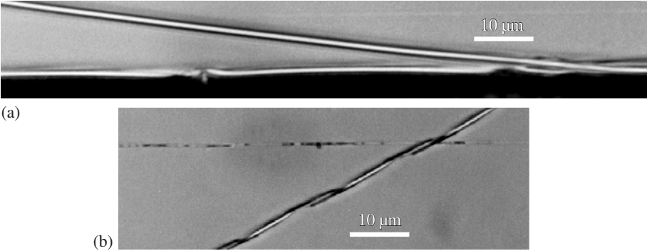
Fig. 2. Photographs of a tube (a) and a helical coil (b) of 1.5 μm in diameter made from a \text{Ge}_{0.4}\text{Si}_{0.6}/\text{Si} bilayer. Thicknesses of \text{Ge}_{0.4}\text{Si}_{0.6} and Si films were 10 and 20 nm, respectively.
