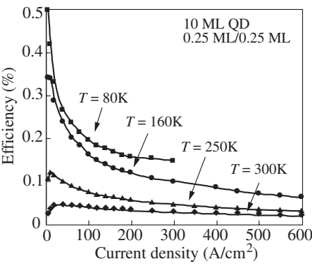
Fig. 1. Spontaneous efficiency versus current density measured for several temperatures. Two trends are observed. The ground state efficiency decreases with increasing temperature, and the efficiency at each temperature decreases with increasing current density.
