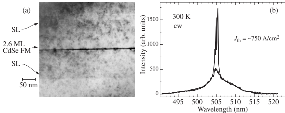
Fig. 4. Cross-section TEM image of the CdSe FM laser diode structure (a) and its cw RT electroluminescence spectra below and above threshold (b).
