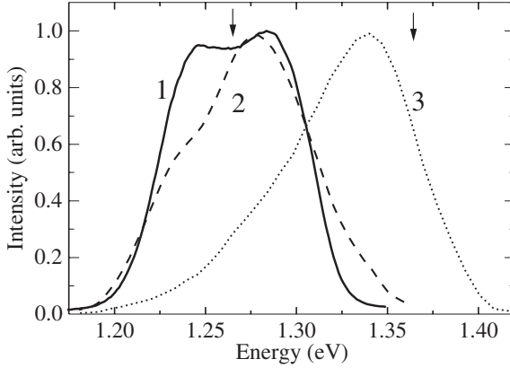
Fig. 1. Photoluminescence spectra of \text{In}_{0.5}\text{Ga}_{0.5}\text{As}/\text{GaAs} QDs at excitation energy E_{\text{exc}} = 1.531 eV, T = 10 K. 1—cw excitation with power density 0.1 \text{ W/cm}^2 ; 2 and 3—pulse pumping with power densities 0.1 and 3.0 \text{ MW/cm}^2 , time delay after excitation pulse equals 200 ps.
