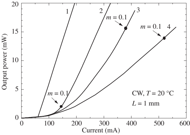
Fig. 1. CW light-current characteristics of SC DH InGaAsP/InP ( \lambda = 1.55 \mu\text{m} ) SLD of mesa construction with tilted stripe angle \alpha : 1— \alpha = 0^\circ (laser diode), 2— \alpha = 5^\circ , 3— \alpha = 10^\circ , 4— \alpha = 14^\circ .
