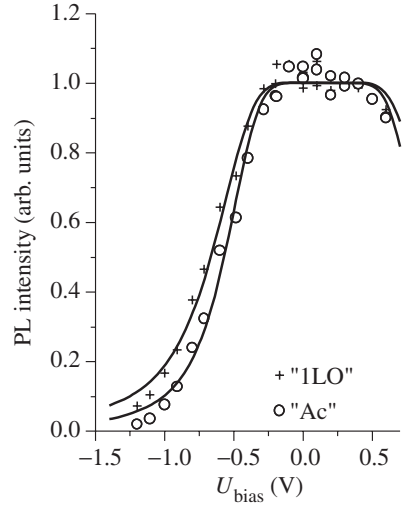
Fig. 4. The dependence of the normalized PL intensity I_{\text{PL}}^* on U_{\text{bias}} in the “1LO” and “Ac” spectral regions fitted by the expression (1).
