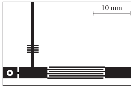
Fig. 4. Superlattice oscillator.
