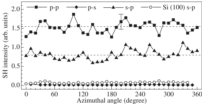
Fig. 2. The dependences of the SH signal of the sample A on the azimuthal angle at different polarizations of fundamental and SH intensities. For comparison the dependence for a single crystal silicon surface (100) is shown.
