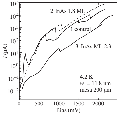
Fig. 1. I-V characteristics of the experimental devices at 4.2 K.
