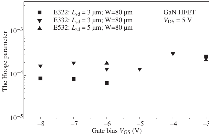
Fig. 1. Hooke parameter \alpha_H as a function of the gate bias. The results are shown for three devices biased at V_{DS} = 5 V. The gate dimensions are 0.25 \mu\text{m} \times 80 \mu\text{m} .
