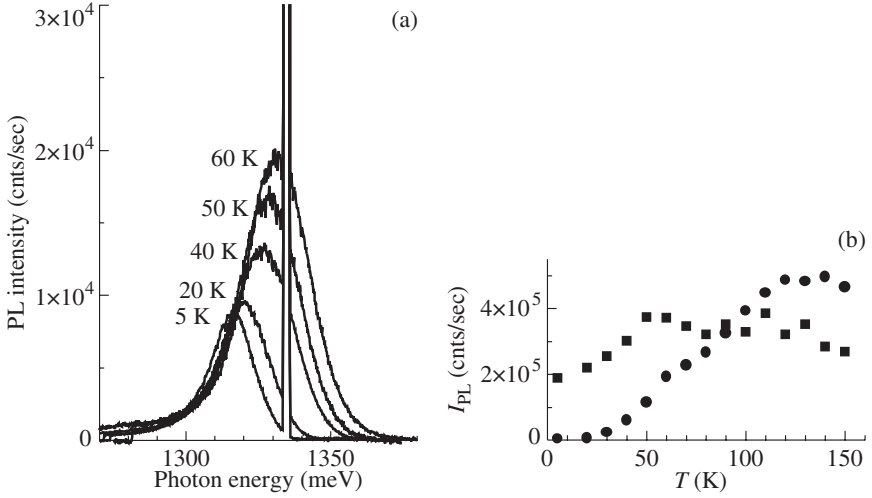
Fig. 2. General PL behavior with changing temperature for InGaAs QDs. (a) PL under resonant excitation E_{\text{exc}} = 1334 meV. (b) Dependence of integral Stokes and anti-Stokes PL intensity on temperature under resonance excitation ( E_{\text{exc}} = 1334 meV).
