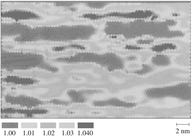
Fig. 1. The color-coded map of the local lattice parameter (LLP) in growth direction digitally processed from a HRTEM image of a stacked submonolayer-CdSe/ZnMgSSe structure.
