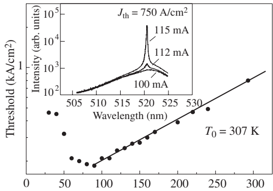
Fig. 2. Temperature dependence of threshold current density of BeMgZnSe SL QW laser diode. Inset shows its RT pulse lasing spectrum.
