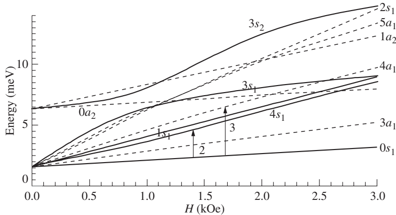
Fig. 2. Spectral positions of the absorption lines 1, 2, 3 versus magnetic field.
