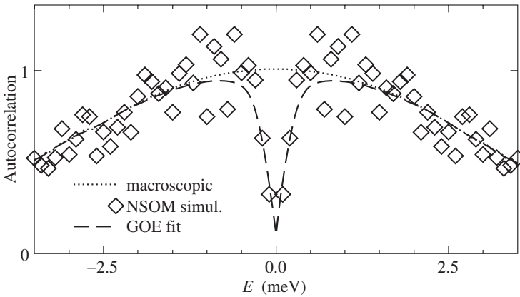
Fig. 1. Simulated spectral autocorrelation for luminescence from 250 NSOM quantum well spectra, each corresponding to an area 120 \times 120 \text{ nm} . Parameters of a 5 nm wide GaAs/ \text{Al}_{0.3}\text{Ga}_{0.7}\text{As} quantum well with disorder strength \langle v^2 \rangle^{1/2} = 8 \text{ meV} are used. GOE-fit (dashed) to the simulation data (diamonds) and corresponding fit to the autocorrelation of the sum of all spectra (macroscopic spectrum) (from Ref. [11]).
