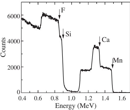
Fig. 2. RBS spectrum from Mn 0.4 Ca 0.6 F 2 film 300 nm thick in random scattering geometry. The energy of incident 4He + ions is 2 MeV.
