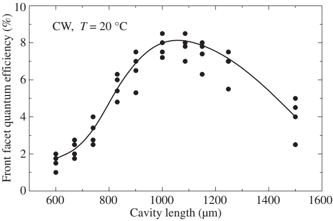
Fig. 2. The dependence of differential quantum efficiency per facet on cavity length of 10^\circ tilted mesastripe SC DH InGaAsP/InP ( \lambda = 1.55 \mu\text{m} ) SLD.
