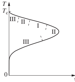
Fig. 2. The phase diagram of final composition-modulated structure near the onset of instability. I: 1D structure, II: 2D structure, III: no solutions in the weak segregation regime, the structure has a finite amplitude.
