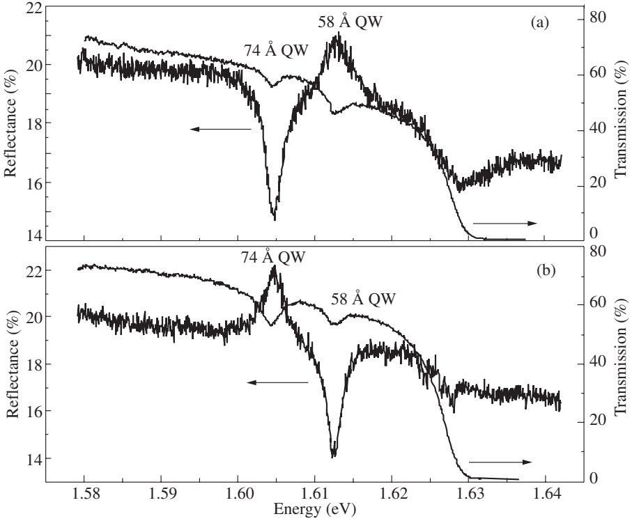
Fig. 1. Reflection and transmission spectra measured at 77 K at normal light incidence. (a) in this sample the 74 Å-thick QW is placed on the 3\lambda/4 distance from the surface and the 58 Å-thick QW is placed on a \lambda distance from the surface. (b) in this sample the 58 Å-thick QW is placed on the 3\lambda/4 distance from the surface and the 74 Å-thick QW is placed on a \lambda distance from the surface.
