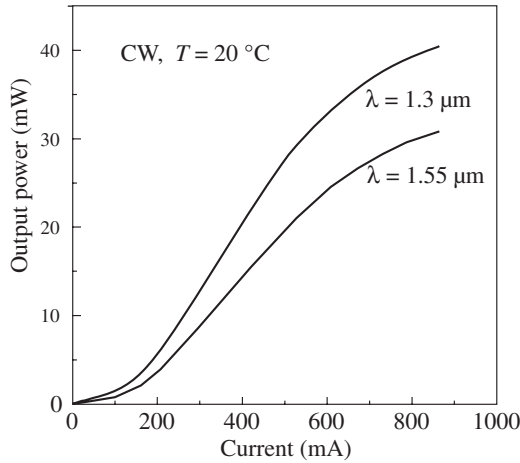
Fig. 3. Room temperature cw light-current characteristics of SC DH InGaAsP/InP ( \lambda = 1.3\text{--}1.55\ \mu\text{m} ) SLDs with 10^\circ tilted mesa stripe ( L = 1\ \text{mm} ) and back absorbing section ( L = 300\ \mu\text{m} ).
