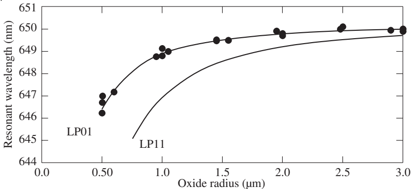
Fig. 9. Calculated (solid lines) and measured (dots) room temperature resonant emission wavelength as a function of oxide aperture radius for selectively oxidized red VCSELs designed for large area emission at 650 nm. The fundamental (LP01) and first higher order mode (LP11) are shown.
