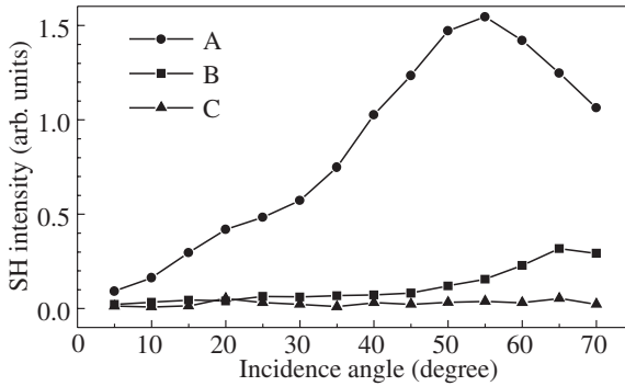
Fig. 3. The dependence of the SH intensity on the angle of pumping radiation incidence for samples A, B, and C.
