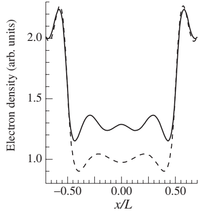
Fig. 3. The electron density distribution calculated with account of the exchange interaction (solid line) and ignoring it (dashed line).
