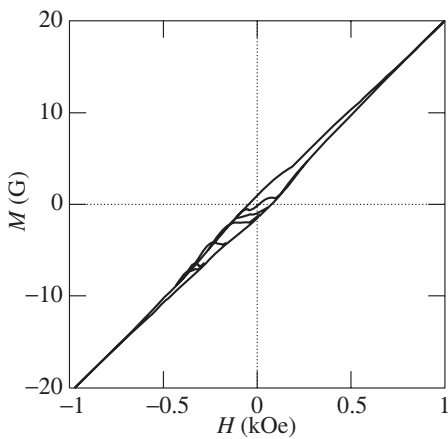
Fig. 5. The dependence of M_z on the magnetic field with \theta = 90^\circ , \phi = 0^\circ .
