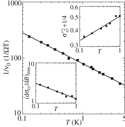
Fig. 3. 1/\nu_0 vs T for the PI transition (full squares, \kappa' = 0.55 ). Upper inset: \ln(\sigma_{xx}^{*2} + 1/4) vs T . The slope of the straight line equals 0.15. Lower inset: (d\sigma_{xy}/dB)_{\min} vs T . The slope of the straight line equals 0.43.
