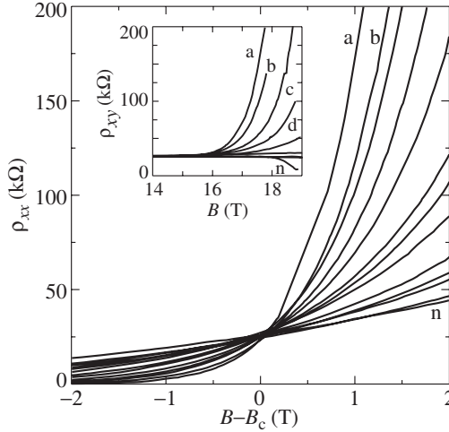
Fig. 1. Resistivity \rho_{xx} and Hall resistance \rho_{xy} (inset) versus magnetic field. B_c is the critical magnetic field defined in the text. The curves are labelled a, b, ..., n and the corresponding temperatures are 0.13, 0.21, 0.26, 0.35, 0.47, 0.59, 0.83, 1.04, 1.4, 1.5, 1.9, 2.2, 3.1 and 4.2 K.
