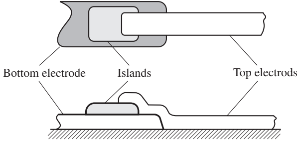
Fig. 1. A geometry of the transistor.
