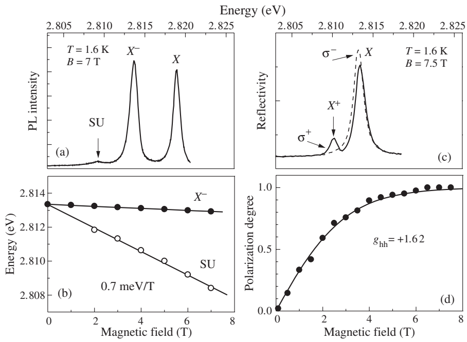
Fig. 4. A shake-up (SU) process in PL spectrum of a 100 Å thick ZnSe/Zn 0.89 Mg 0.11 Se 0.18 SQW with n_e \approx 10^{10} \text{ cm}^{-2} (a) and magnetic-field dependence of the SU line (b). A positively charged exciton in reflectivity spectra of a 130 Å ZnSe/Zn 0.89 Mg 0.11 Se 0.18 QW with n_h \approx 3 \times 10^{10} \text{ cm}^{-2} (c) and polarization dependence of X^+ line in magnetic fields: experiment (circles) and calculation for T = 1.6 K (line).
