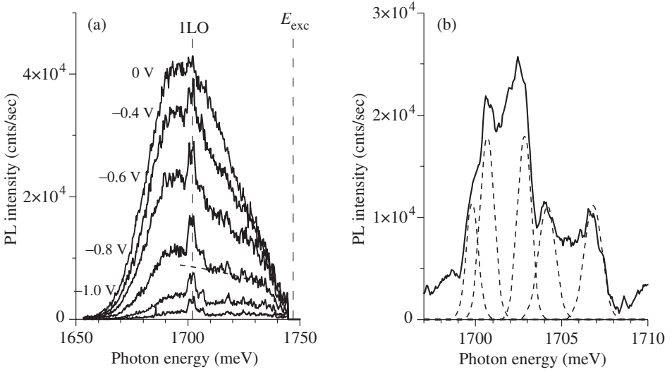
Fig. 1. (a) Dependence of the PL spectrum on the applied electric field. The excitation energy is 1747 meV. The positions of the excitation photon energy and the 1LO resonances are marked by the vertical dashed lines. (b) Part of the PL spectra around the 1LO resonance ( E_{\text{exc}} = 1747 meV, U_{\text{bias}} = -0.8 V). A decomposition of the resonance into Gaussians is shown by the dotted lines. The signal was accumulated by the detection of the PL from the large illuminates sample area of about 0.03 \text{ mm}^2 . A background signal is substrated according the dashed line shown in the Fig. 1(a).
