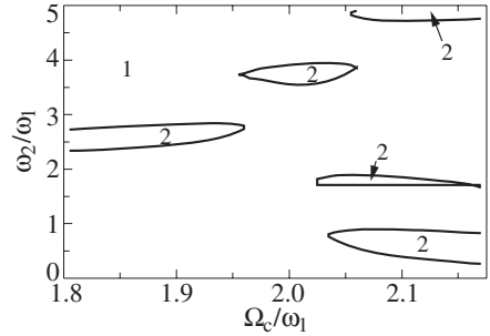
Fig. 3. The regions of negative conductivity (2) on the “step” LN. (1) is the stable region.
