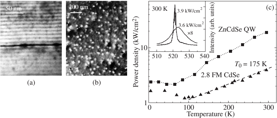
Fig. 3. Cross-sectional (a) and plan-view (b) TEM images of laser structures with 2.8 ML CdSe/ZnSe FM active region. (c) Temperature dependence of threshold power density for FM (triangle) and QW (square) laser structures. RT FM laser generation spectra are presented in the inset.
