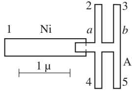
Fig. 1. Sample geometry. 1—Nickel electrode; 2–5—Aluminium electrodes. The voltage U_{23} is measured as a function of current I_{45} or I_{15} applied to part ab .
