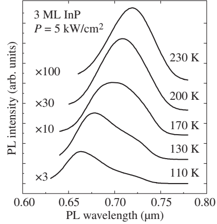
Fig. 4. PL spectra of 3 ML InP NSIs at high excitation level ( 5 \text{ kW/cm}^2 ) for different measuring temperatures.
