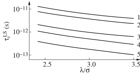
Fig. 3. Calculated parametrical dependences of the transport relaxation time \tau_t^{LS}(N_D, \sigma\lambda, T) . T = 4.2 K. \lambda , nm: 1, 2—53, 3—45, 4, 5—40. N_D , \text{cm}^{-2} : 1— 1 \times 10^{12} , 2, 3, 4— 1.4 \times 10^{12} , 5— 3 \times 10^{12} .
