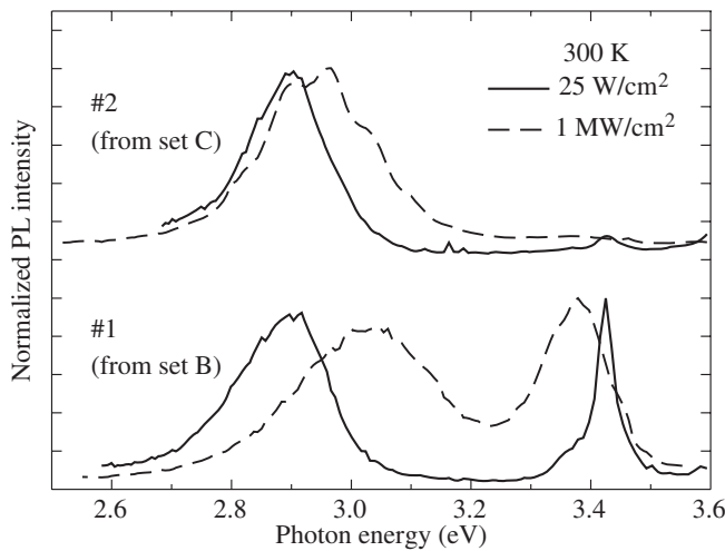
Fig. 2. Room temperature PL spectra at low and high excitation density for samples from sets B and C grown under the same TMI/(TMI + TMG) mole flow ratio of 0.415.
