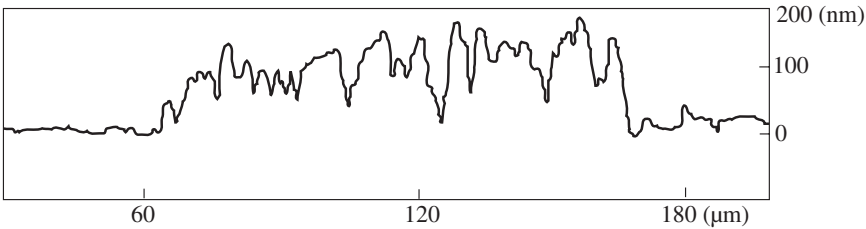
Fig. 3. Profile of chemically nitridized stripe on (100) GaAs after etching.
