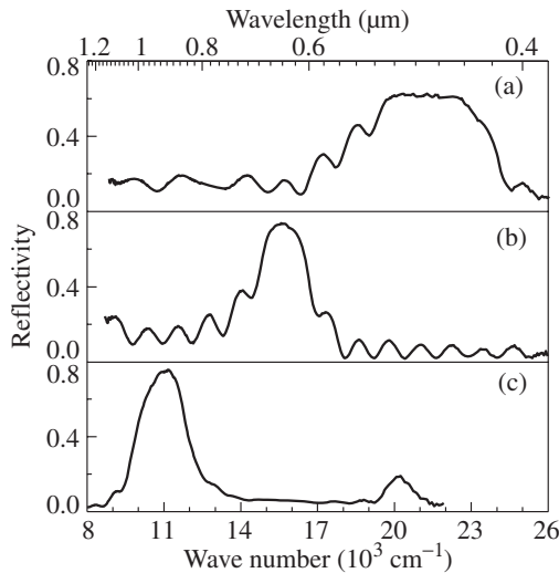
Fig. 1. Reflection spectra of structures A (a), B (b) and C (c) at normal light incidence.
