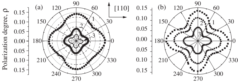
Fig. 2. Polar diagrams of the PL polarization in oxidized Si NCs under non-resonant (a) and resonant (b) conditions; (a) \lambda_{\text{ex}} = 442 nm (2.8 eV), \lambda_{\text{det}} : 1—550 nm (2.25 eV); 2—700 nm (1.77 eV); 3—750 nm (1.65 eV); (b) \lambda_{\text{ex}} = 633 nm (2.8 eV), \lambda_{\text{det}} : 1—670 nm (1.85 eV); 2—700 nm (1.77 eV); 3—750 nm (1.65 eV).
