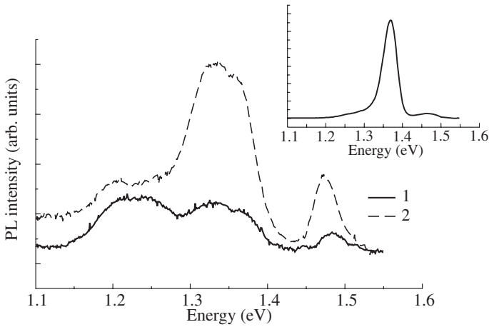
Fig. 2. Dependence of PL spectra of InAs/GaAs sample ( 7^\circ , [001]) on excitation intensity (1—100 mW, 2—400 mW) at T = 170 K. Insert—this sample PL spectrum at T = 10 K and excitation intensity 100 mW.
