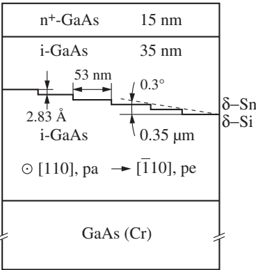
Fig. 1. The overall view of the structure with \delta -Sn layer on i-GaAs vicinal plane.
