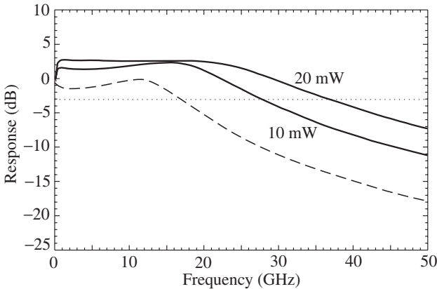
Fig. 4. Simulated small signal responses of a stepped-mesa structure under modulation by the side voltage (solid) at different output power levels. Direct modulation response at 10 mW (dash) is shown for comparison.
