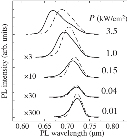
Fig. 3. 77 K PL spectra of 3 ML (solid line) and 5 ML (dash line) InP NSIs at different excitation level.
