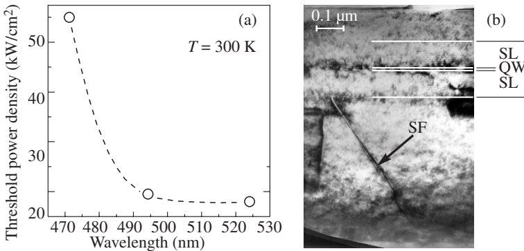
Fig. 1. (a) Room temperature threshold power density as a function of lasing wavelength for three SL QW laser structures with different compositions of (Zn,Cd)Se QW. (b) Cross-sectional TEM image of one of the structures, SF is a stacking fault.
