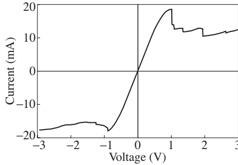
Fig. 3. Current-voltage characteristic.
