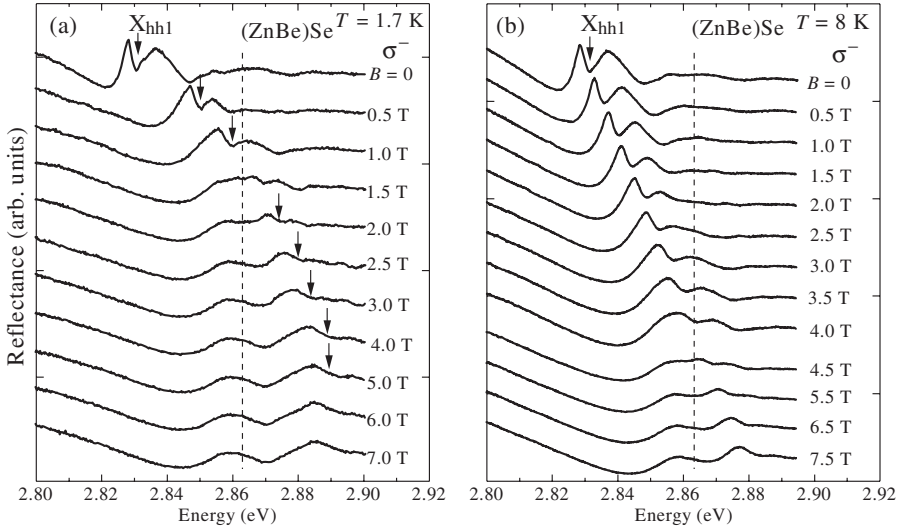
Fig. 2. \sigma^- -polarized reflectance spectra of a \text{Zn}_{0.91}\text{Mn}_{0.09}\text{Se}/\text{Zn}_{0.972}\text{Be}_{0.028}\text{Se} MQW taken at temperatures of 1.7 K (a) and 8 K (b). Arrows indicate X_{\text{hh}1} -energies determined from PLE spectra.
