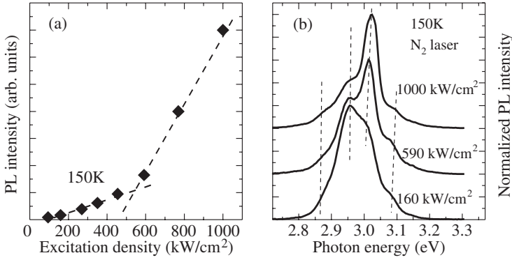
Fig. 2. Photoluminescence intensity versus excitation density (a) and PL spectra (b) taken at 150 K.
