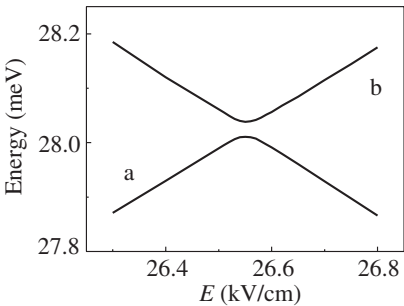
Fig. 1. The behaviour of energy position of the asymmetric ground heavy hole state (a) and the symmetric first excited heavy hole state (b) in the region of anticrossing.
