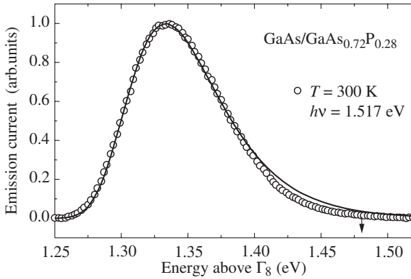
Fig. 3. Experimental electron energy distribution curve T = 300\text{ K} , together with results of the calculation (solid line) using the localized states model. Band gap value is shown by arrow.
