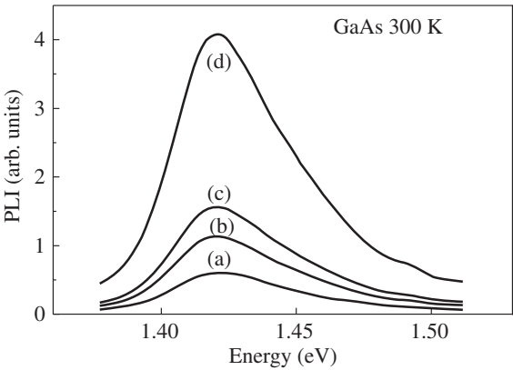
Fig. 4. Photoluminescence spectra of GaAs for untreated (100) surface (a), treated with \text{Na}_2\text{S} (b), with (\text{NH}_4)_2\text{S} (c), with hydrazine-based solution (d).
