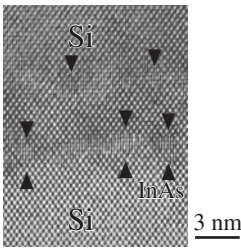
Fig. 3. Cross section image of the sample A taken at high resolution. InAs clusters are marked by arrows.
