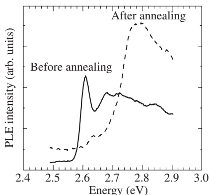
Fig. 2. PLE spectra measured at 77 K in unannealed (solid curve) and annealed (dashed curve) samples. The detection energy is 2.0 eV.
