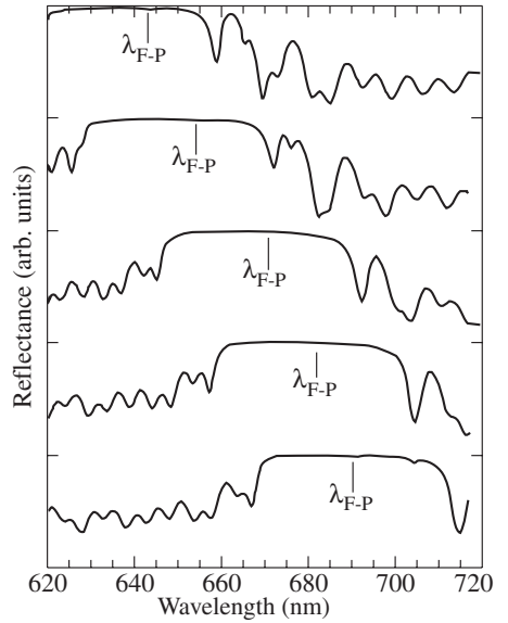
Fig. 5. Measured reflectance spectra (at normal incidence) at five approximately equally spaced points across a nonrotated red VCSEL wafer.
