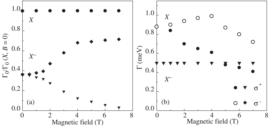
Fig. 3. Magnetic-field dependences of radiative ( \Gamma_0 ) and nonradiative ( \Gamma ) dampings for exciton and trion transitions in a 100 Å thick \text{ZnSe}/\text{Zn}_{0.89}\text{Mg}_{0.11}\text{S}_{0.18}\text{Se}_{0.82} SQW with n_e \approx 9 \times 10^{10} \text{ cm}^{-2} . Results for two circular polarized components of reflectivity spectra are presented at T = 1.6 \text{ K} .
