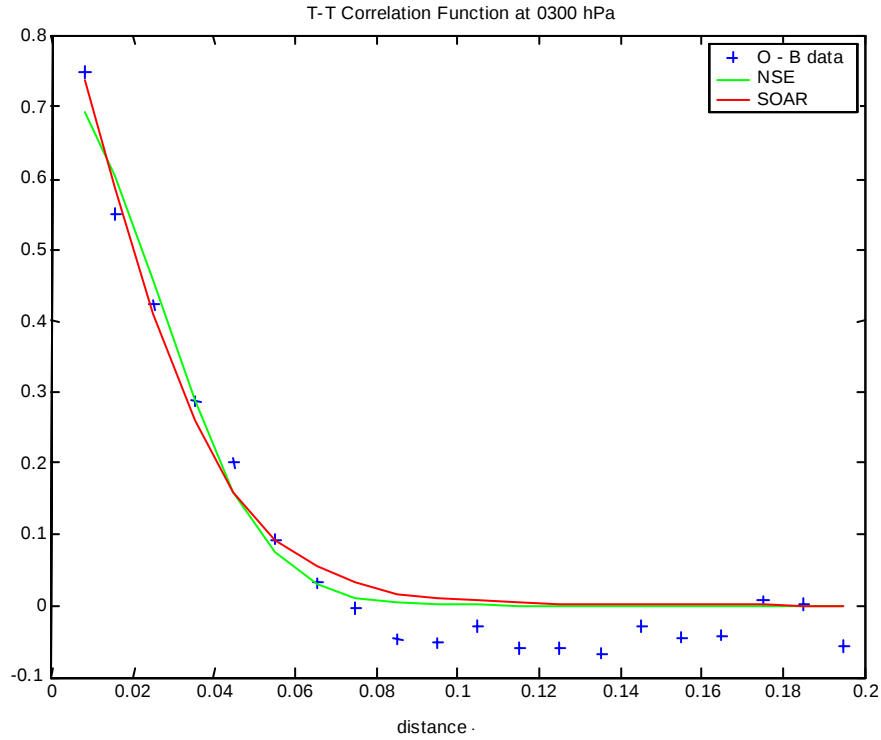
Figure 3.2 Correlation fit for isobaric (300 hPa) Temperature Observation increments.
