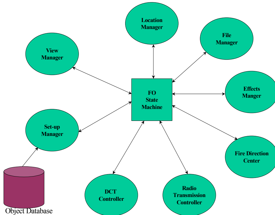
Figure 14. Diagram of the modules that interface with the FO state machine
