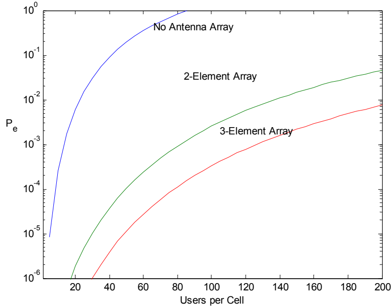
Figure 5.7 Probability of Bit Error for DS-CDMA System with a SNR per Bit of 15 dB (\sigma_{dB}=7, R_{cc}=1/2, v=8) .
