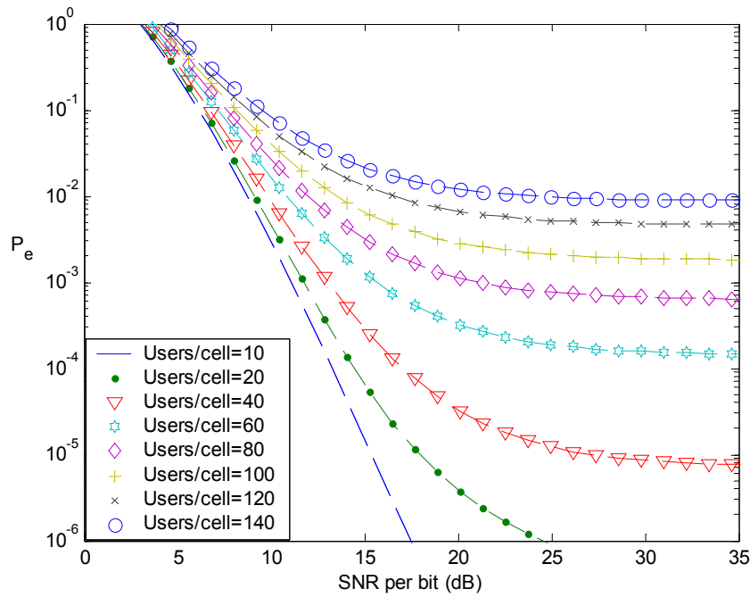
Figure 5.4 WB Performance Boundaries for Our DS-CDMA System with a 2-Element Linear Adaptive Array System ( \sigma_{dB}=7 , R_{cc}=\frac{1}{2} , v=8 )
