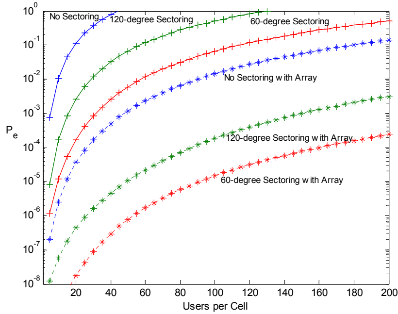
Figure 5.11 Probability of Bit Error for a 3-Element Linear Adaptive Array DS-CDMA System Using Sectoring for \sigma_{dB} = 9 dB with a SNR per Bit of 15 dB ( R_{cc} = 1/2 and v = 8 ).
