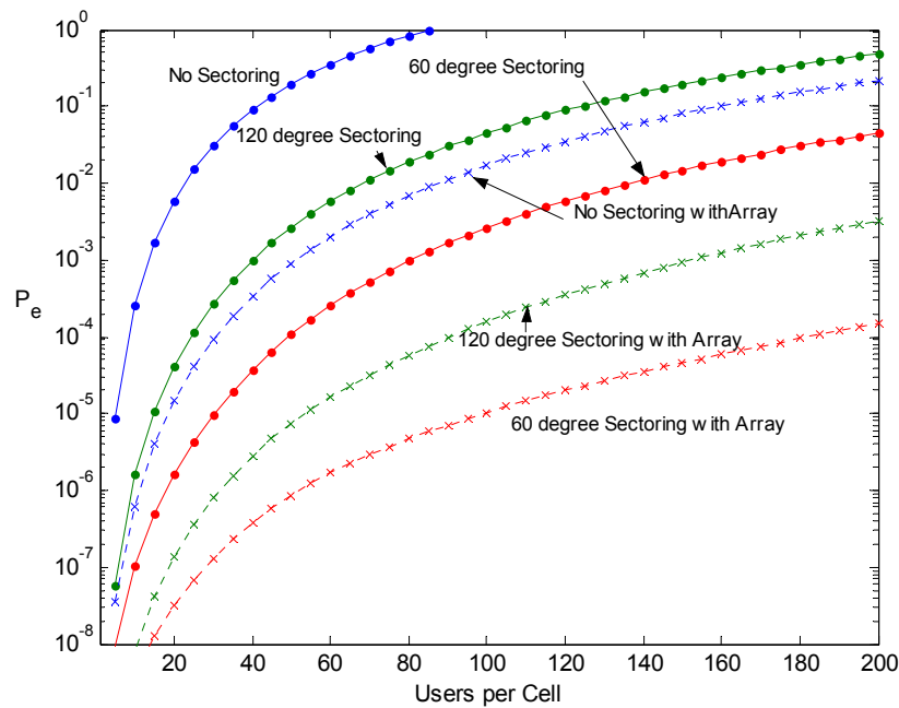
Figure 5.17 System Enhancement with \pm 3 Degree of Orientation Offset at Worst-Worst Case for a 2-Element Array ( \sigma_{dB} = 7 , R_{cc} = 1/2 , v = 8 )
