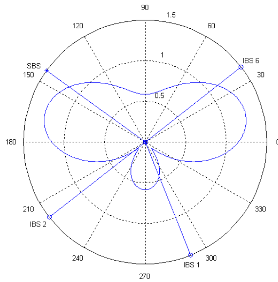
Figure 5.15 Antenna Factor of the WW Case for a 4-Element Array Antenna at +1 Degree Offset with a Path-Loss Ratio of 0.7950
