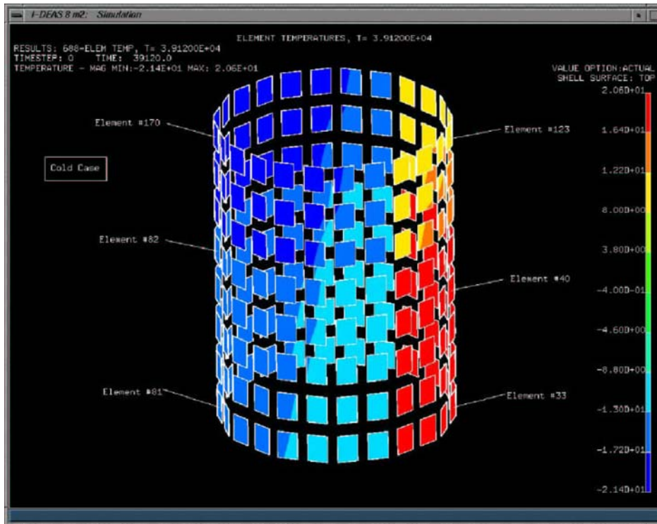
Figure 15 Element Temperatures Simulation [From Ref. 10].
