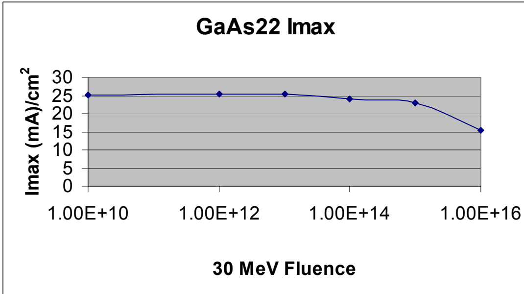
Figure 43 GaAs LINAC Testing Imax Curve [From Ref. 15].
