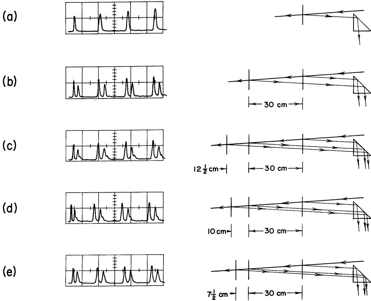
(*) Fig. 2. Multiple reflections of ultrashort laser pulses observed with photodiode and displayed on an oscilloscope. Oscillograms are shown on the left: horizontal time scale is 5 nsec/cm; vertical deflection is intensity in relative units. Corresponding experimental setup is shown on the right.
