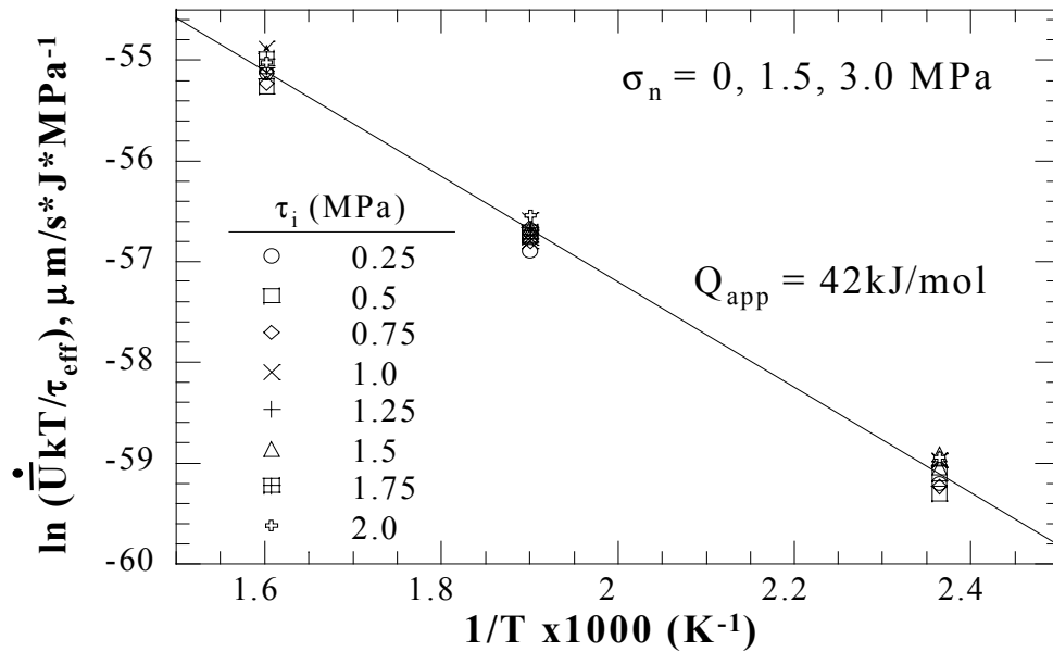
Figure 32. Interfacial Shear Stress and Temperature Normalized Interface Displacement Rate Showing Arrhenius Temperature Dependence with an Apparent Activation Energy of \sim 42 \text{ kJ/mol} with Applied Interfacial Normal Stress.
