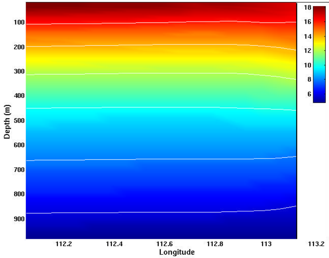
Figure 12d. Cross-section of temperature ( ^{\circ}\text{C} ) at 25.7^{\circ}\text{S} for Experiment 2 day 60, with a contour interval of two degrees.
