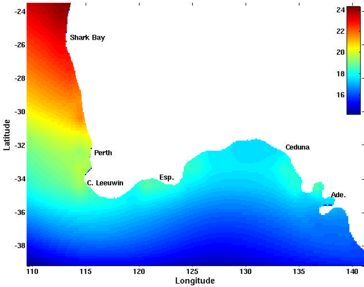
Figure 8. Annual climatological surface temperature ( ^{\circ}\text{C} ) obtained from Levitus and Boyer (1994).
