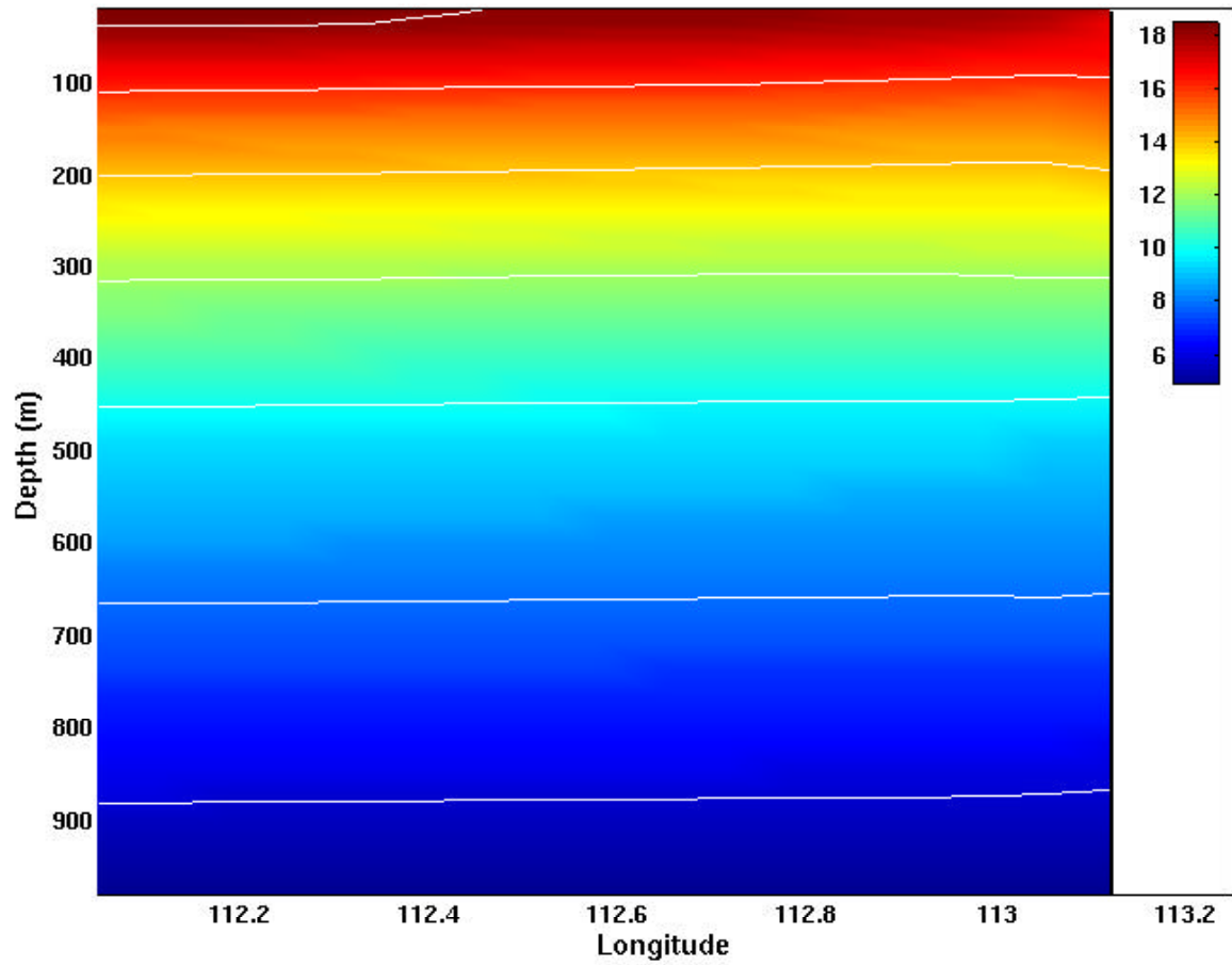
Figure 12b. Cross-section of temperature ( ^{\circ}\text{C} ) at 25.7^{\circ}\text{S} for Experiment 2 day 39, with a contour interval of two degrees.
