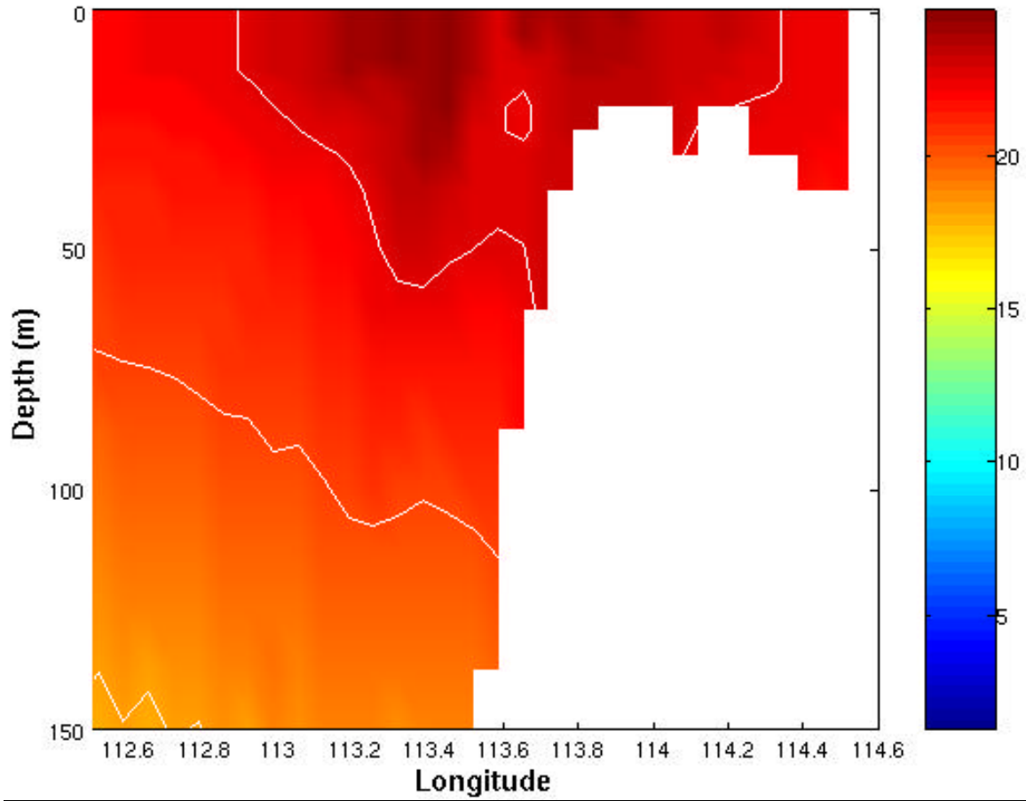
Figure 17e. Cross-section of temperature ( ^{\circ}\text{C} ) at 28.9^{\circ}\text{S} for Experiment 7 day 60, with a contour interval of 2.5 degrees.
