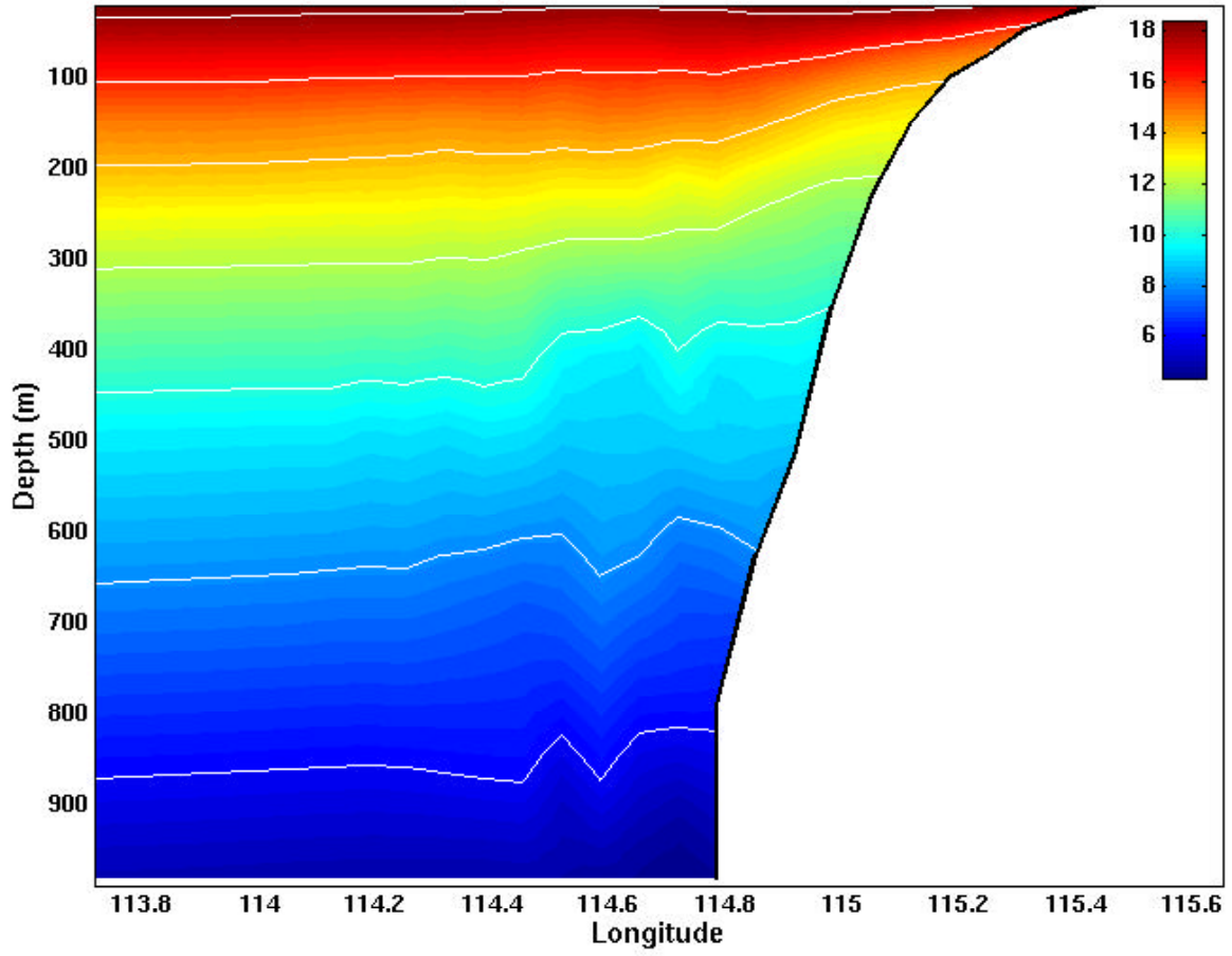
Figure 13d. Cross-section of temperature ( ^{\circ}\text{C} ) at 32^{\circ}\text{S} for Experiment 3 day 60, with a contour interval of two degrees.
