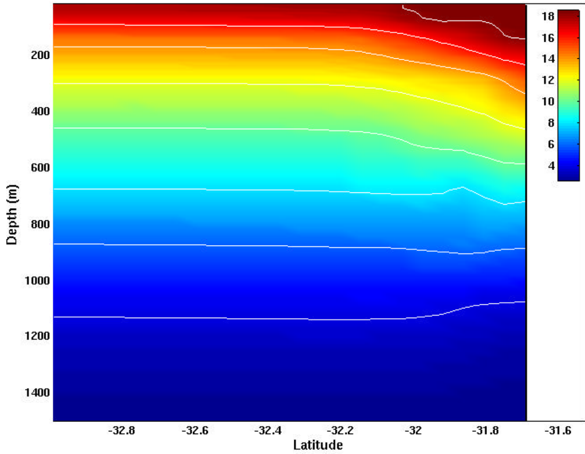
Figure 14d. Cross-section of temperature ( ^{\circ}\text{C} ) at 130.1^{\circ}\text{E} for Experiment 4 day 42, with a contour interval of two degrees.
