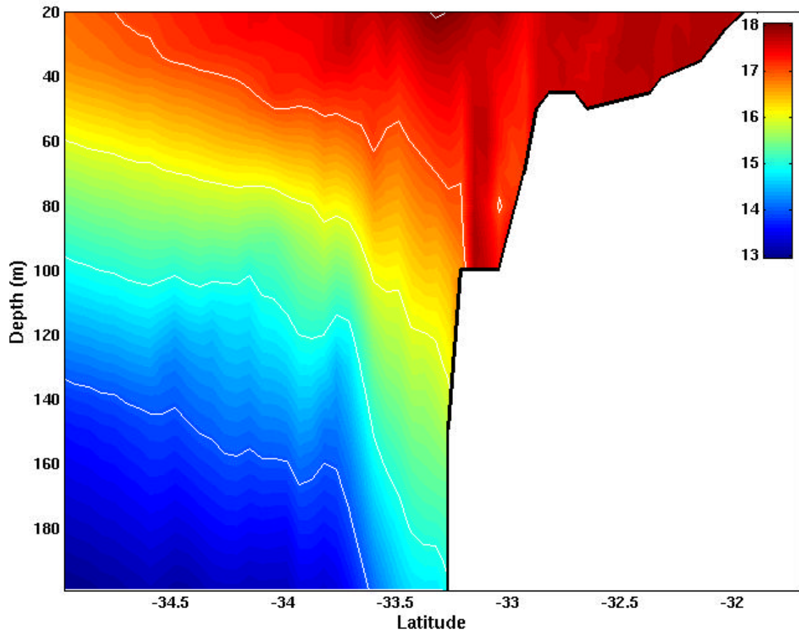
Figure 17h. Cross-section of temperature ( ^{\circ}\text{C} ) at 130.1^{\circ}\text{E} for Experiment 7 day 60, with a contour interval of one degree.
