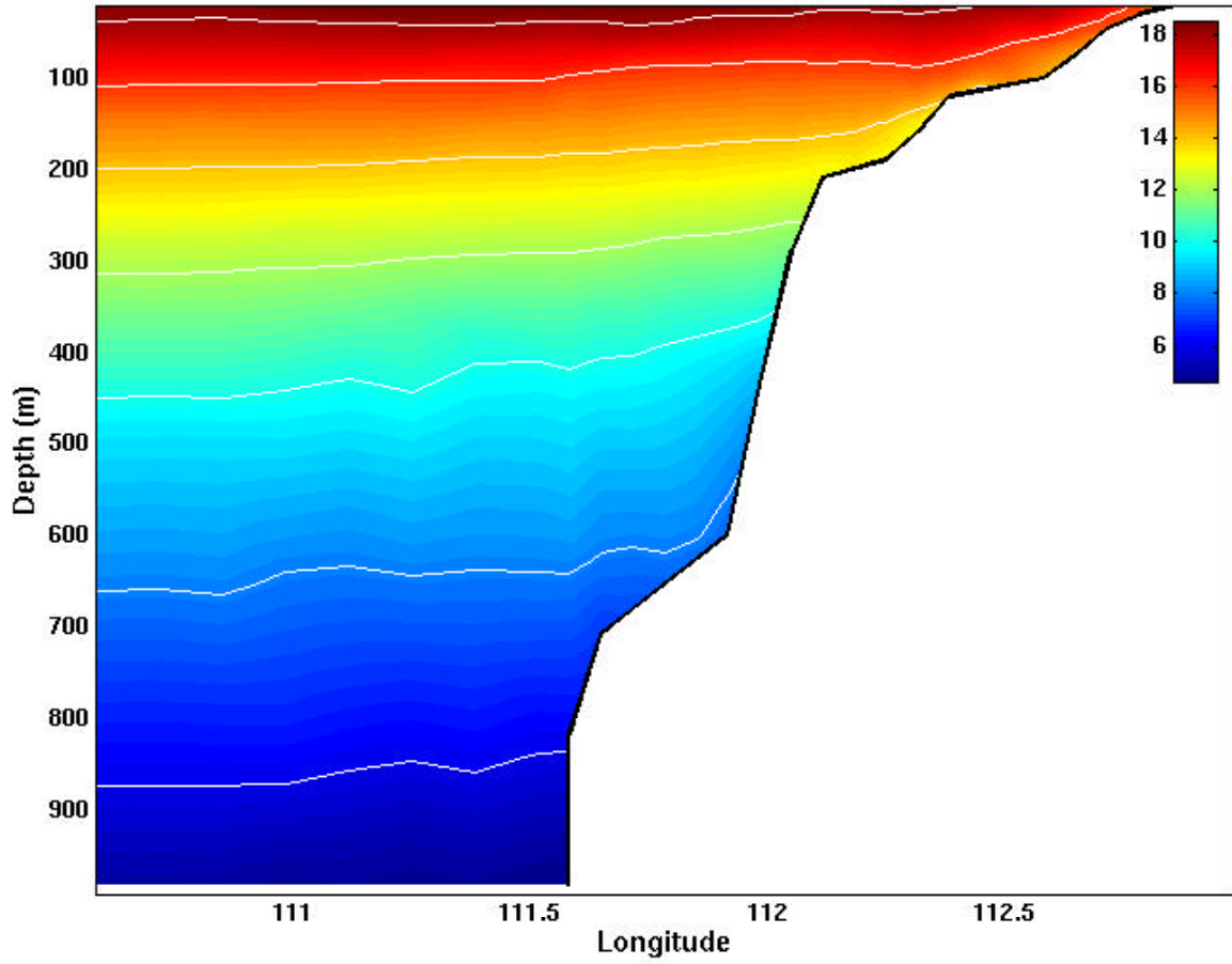
Figure 13b. Cross-section of temperature ( ^{\circ}\text{C} ) at 25.7^{\circ}\text{S} for Experiment 3 day 60, with a contour interval of two degrees.
