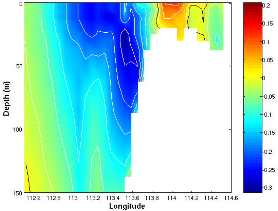
Figure 17d. Cross-section of north-south velocities (m/s) at 28.9^{\circ}\text{S} for Experiment 7 day 60, with a contour interval of 5 cm/s. Red is equatorward (north).
