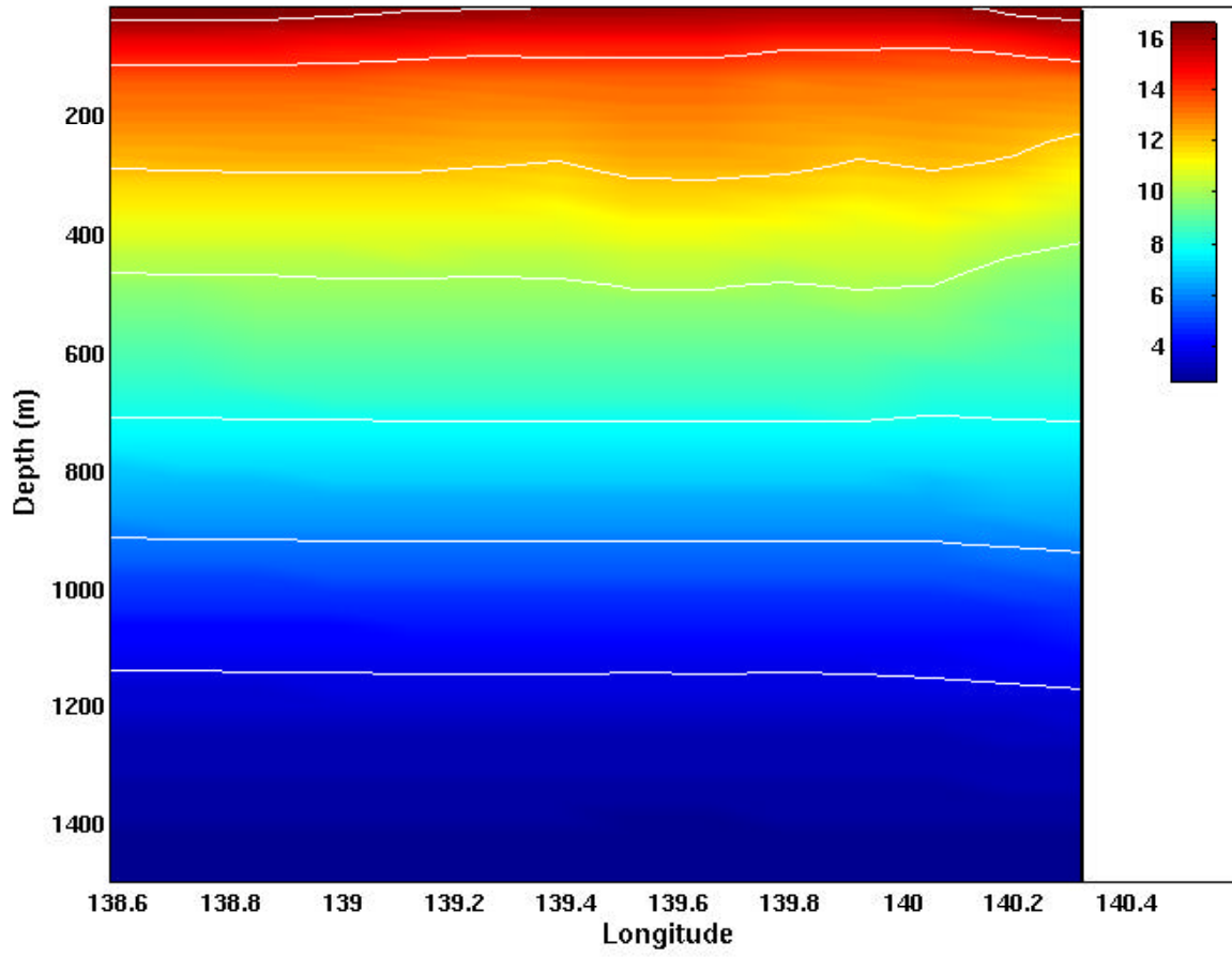
Figure 14f. Cross-section of temperature ( ^{\circ}\text{C} ) at 38^{\circ}\text{S} for Experiment 4 day 42, with a contour interval of two degrees.
