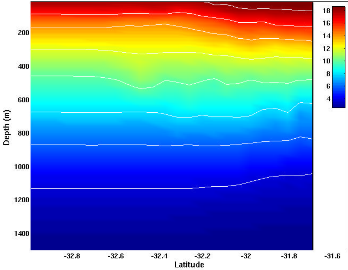
Figure 14h. Cross-section of temperature ( ^{\circ}\text{C} ) at 130.1^{\circ}\text{E} for Experiment 4 day 60, with a contour interval of two degrees.
