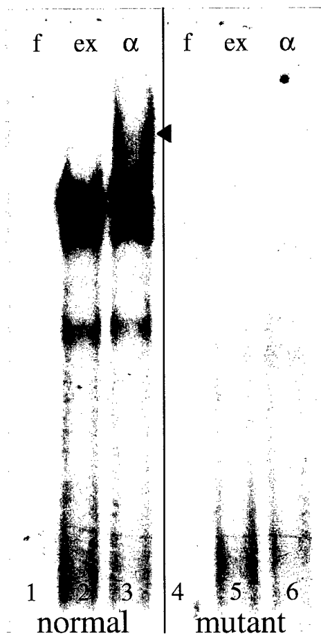
Figure 5. Gelshift assays using oligos specific to (a) SP1 and (b) CRE. In each experiment, oligos possessing altered (mutant) binding motifs were also used. These CG to TG alterations dramatically changed the protein binding profiles seen binding to the SP1 and the CRE sequences. The arrowhead indicates the supershift seen in the presence of the anti-SP1 antibody (Santa Cruz). F: free probe, no protein; ex: probe and cell extract; \alpha : probe, cell extract and antibody.
