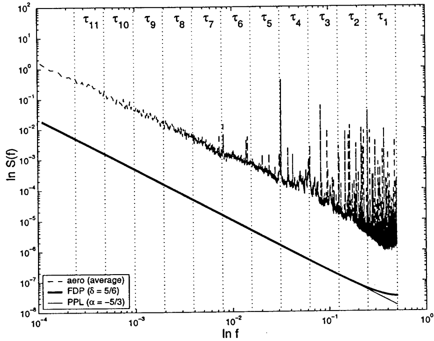
FIGURE 5.7. Averaged estimated SDF for aero series and the theoretical SDFs for an FDP process and pure power law (PPL) model of fully developed Kolmogorov turbulence with an infinite inertial range. The FDP and PPL curves are purposefully offset from the average SDF of aero series so that their \ln - \ln SDF slopes may be easily compared over a broad range of scale. The vertical divisions represent the octaves over which the wavelet coefficients at scale \tau_j are nominally associated.
