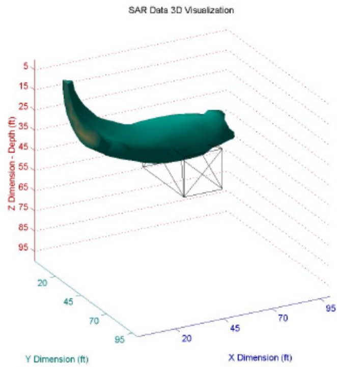
Figure 6.16b. Data Set 16 GPR Processed Image
