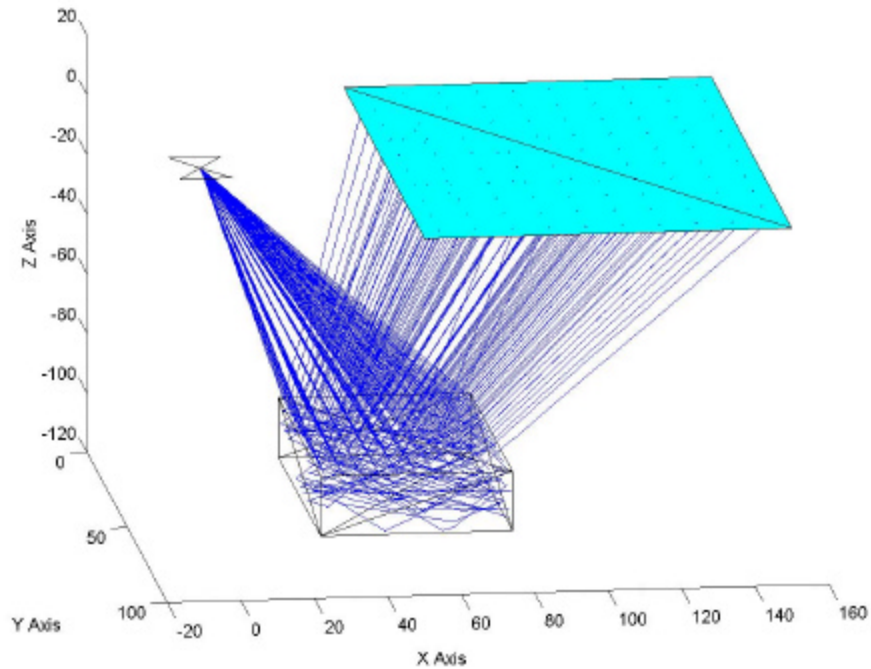
Figure 6.13a. Data Set 13 Scene Configuration Image
