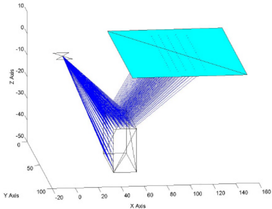
Figure 6.14a. Data Set 14 Scene Configuration Image
