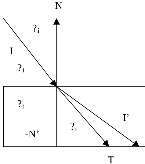
Figure 4.7 Transmitted Ray Calculation Diagram
