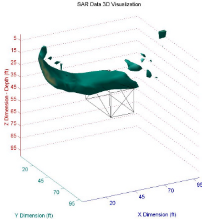
Figure 6.17b Data Set 17 GPR Processed Image
