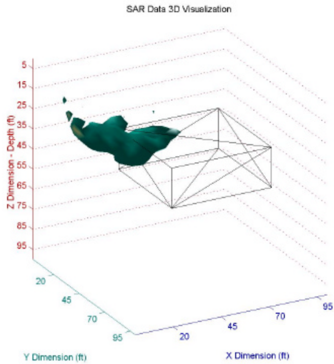
Figure 6.5b. Data Set 5 GPR Processed Image
