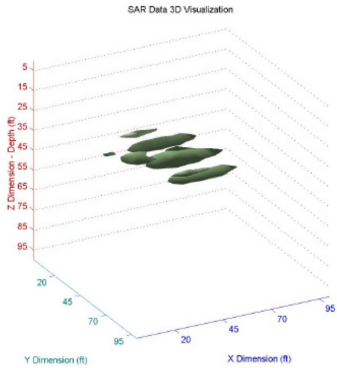
Figure 6.20. Data Set 20 GPR Processed Image
