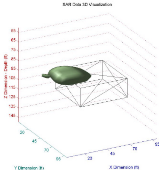
Figure 6.13b. Data Set 13 GPR Processed Image
