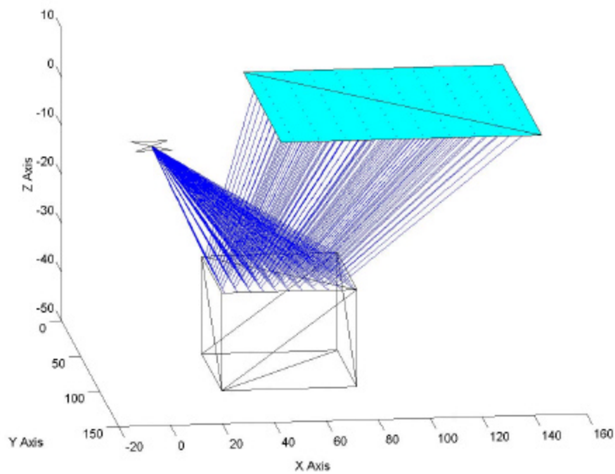
Figure 6.3a. Data Set 3 Scene Configuration Image
