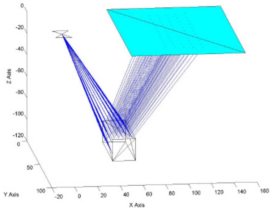
Figure 6.12a. Data Set 12 Scene Configuration Image
