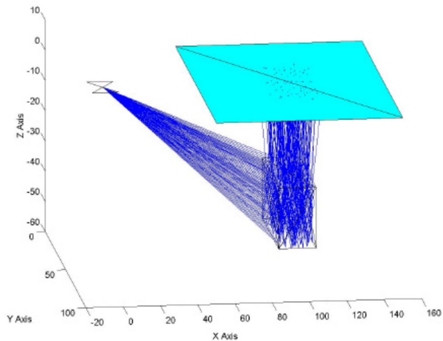
Figure 6.11a. Data Set 11 Scene Configuration Image
