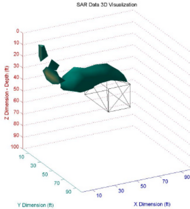
Figure 6.14b. Data Set 14 GPR Processed Image
