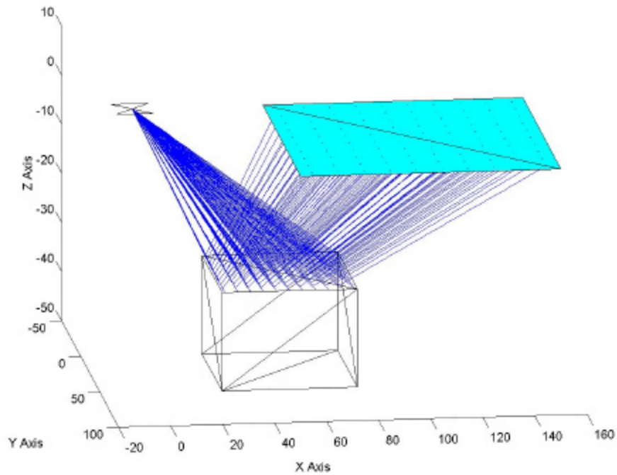
Figure 6.2a. Data Set 2 Scene Configuration Image
