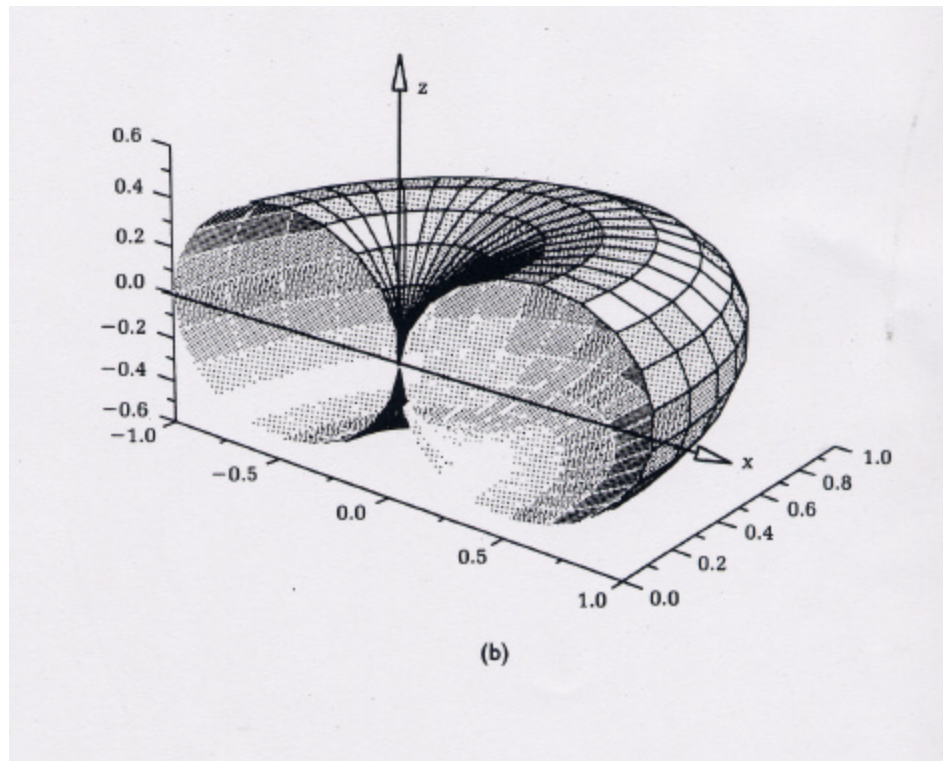
Figure 3.4. Antenna Gain Pattern of A Hertzian Dipole Antenna 1
