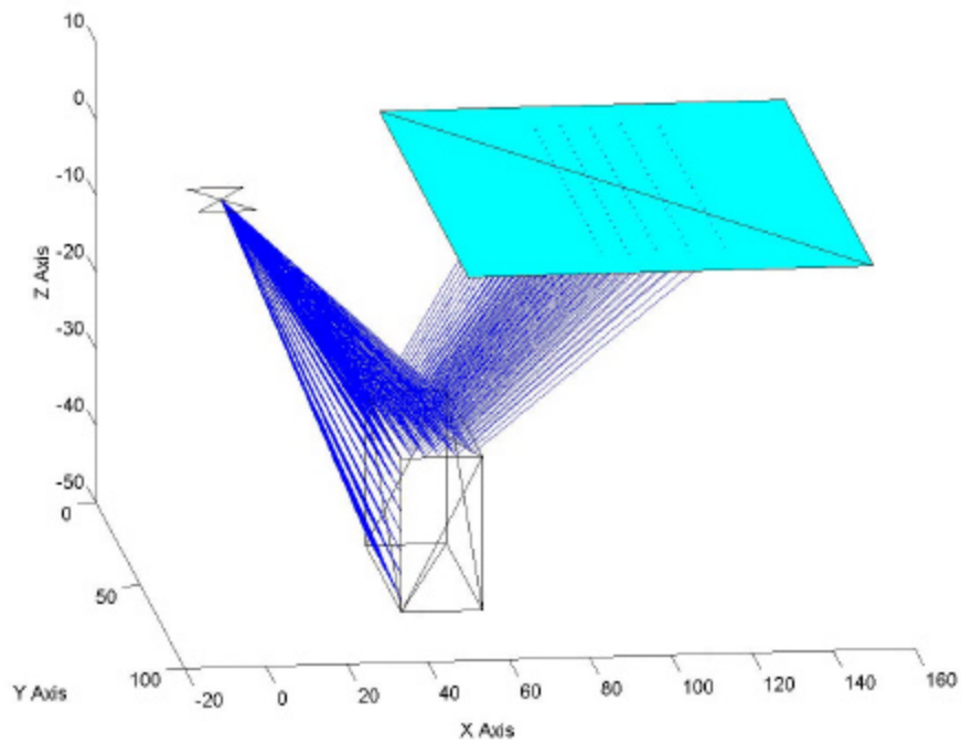
Figure 6.15a Data Set 15 Scene Configuration Image
