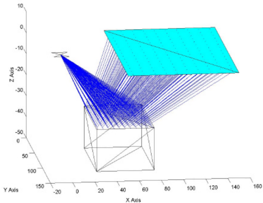
Figure 6.6a. Data Set 6 Scene Configuration Image
