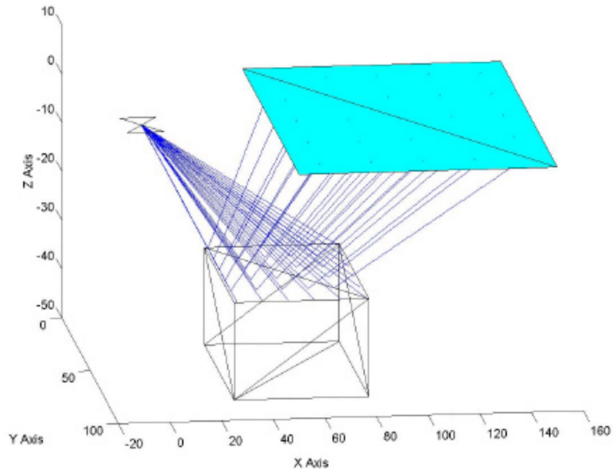
Figure 6.5a. Data Set 5 Scene Configuration Image
