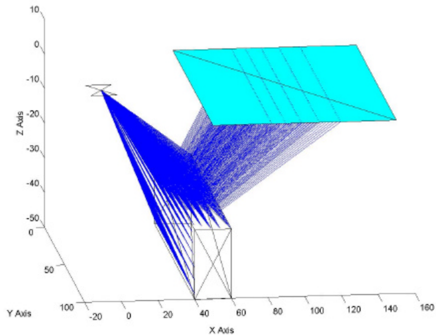
Figure 6.10a. Data Set 10 Scene Configuration Image
