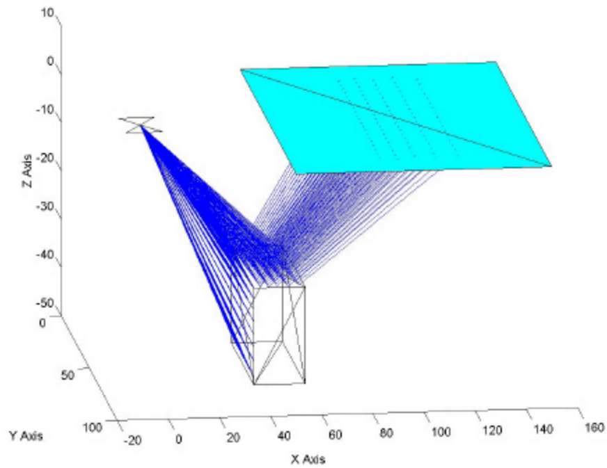
Figure 6.8a Data Set 8 Scene Configuration Image
