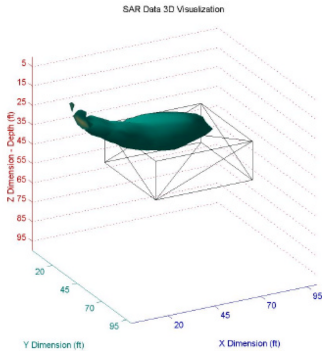
Figure 6.4b. Data Set 4 GPR Processed Image
