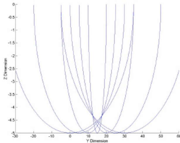
Figure 7.3 Two Dimensional Representation of GPR Processed Image in Y Dimension
