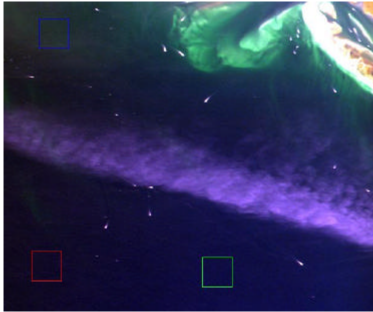
Figure 9. AVIRIS data collected at the LEO site on July 12, 1998. This is scene 4 of the complete data set.
