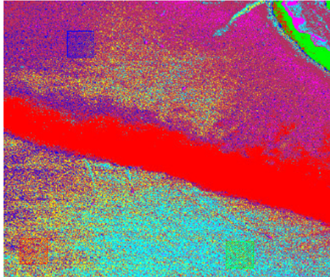
Figure 13. Representation of the models chosen for Scene 4 of the 1998 data set. Red is clouds, Green is the land, Blue is Maritime, Yellow is coastal, Cyan is Coastal-a, Magenta is Tropospheric, and Maroon is Urban.
