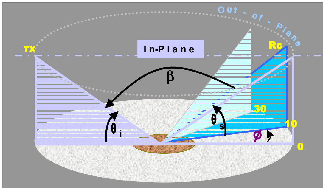
Figure 1. Illustration of Bistatic Signal Geometry
