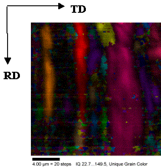
Figure 11. An image quality grayscale unique grain color map of a 20 \mu\text{m} x 20 \mu\text{m} area of AR16 material in the as-received condition utilizing a 0.2 \mu\text{m} step size. This structure is essentially the same as described in Figure 9, however, the elongated coarser grains appear to be larger in size and better defined.
