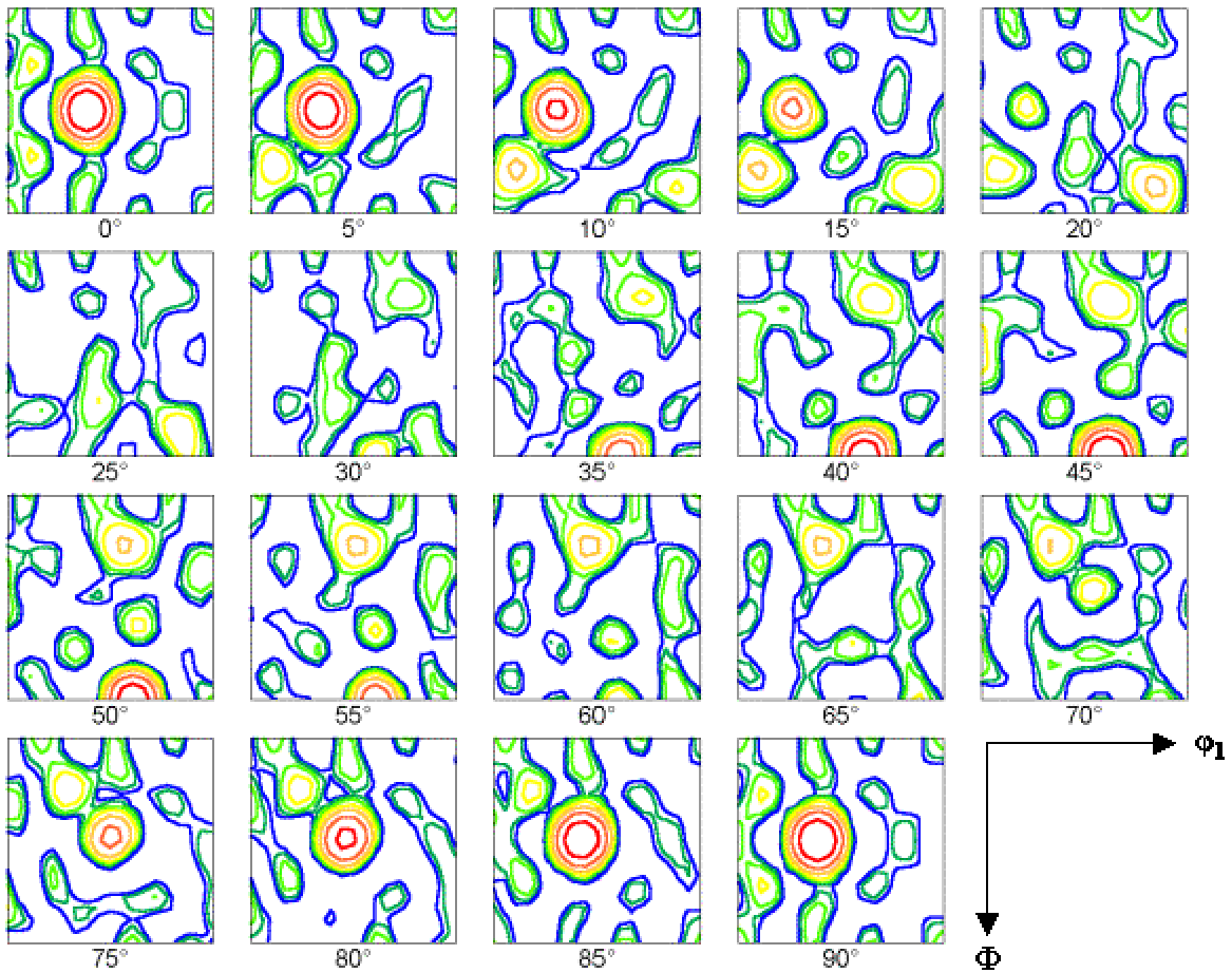
Figure 12. Euler space contour map for the AR16 material revealing distinct B1 and B2 texture components at (\varphi_1=35^\circ, \Phi=45^\circ, \varphi_2=0^\circ) and (\varphi_1=55^\circ, \Phi=90^\circ, \varphi_2=45^\circ) respectively. The red lines indicate an increased local intensity at that point described by the Euler angles. The contour plot was constructed by ranging \varphi_1 and \Phi from 0^\circ - 90^\circ , with 5^\circ increments, holding \varphi_2 constant.
