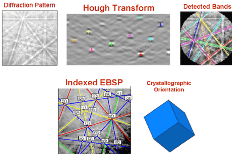
Figure 6. Schematic illustrating the raw diffraction pattern, Hough Transform, the resulting detected bands and the final indexed EBSP based on the crystallographic orientation shown. (From: TSL-OIM.com)
