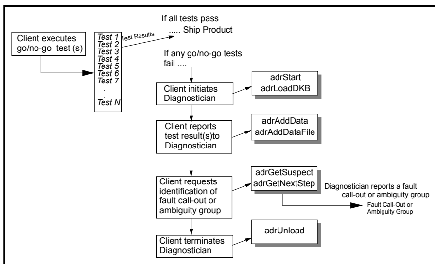
Figure 8 – Go/No-Go Control Mode
