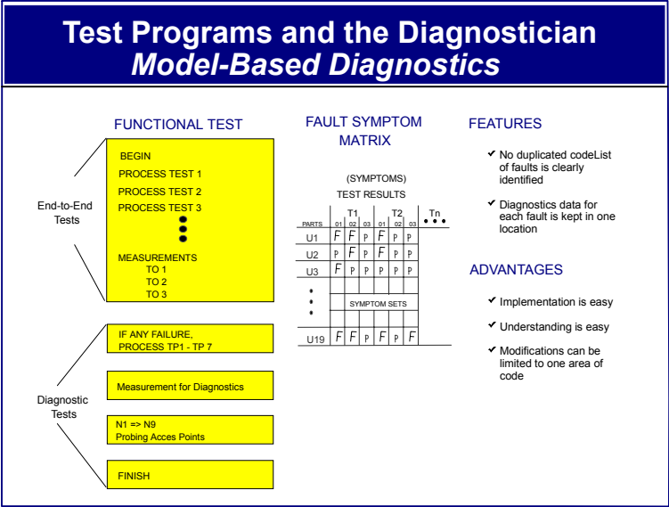
Figure 6 – Model Based Test Program Structure
