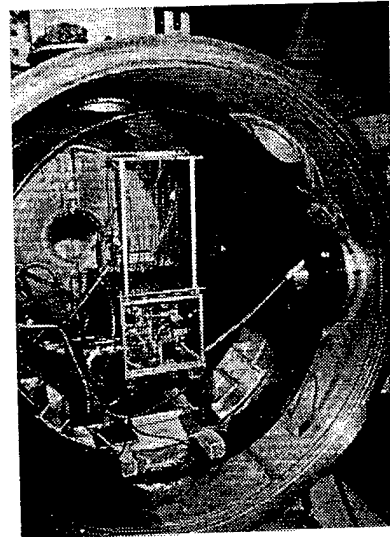
Figure 6: JPL Inverted Pendulum Thrust Stand
