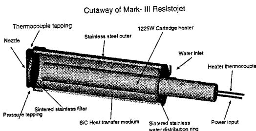
Figure 12: Cutaway of Mk-III Resistojet
