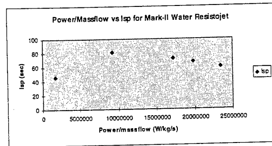
Figure 10: Isp vs. Input Power/Mass Flow for Mark-II Resistojet (H 2 O)
