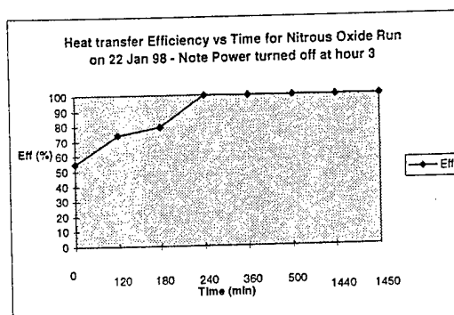
Figure 15: Heat transfer efficiency vs.time for the Mark-III ( N_2O )
