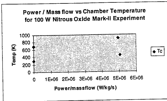
Figure 8: Chamber Temperature vs. Input Power /Mass Flow for Mk-II Resistojet (N 2 O)
