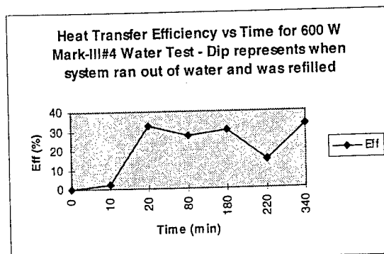
Figure 16: Heat transfer efficiency vs.time for the Mark-III ( H_2O @ 600 W)
