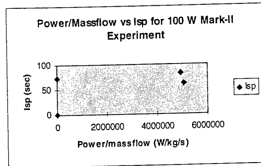
Figure 11: Isp vs. Input Power/Mass Flow for Mark-II Resistojet (N 2 O)
