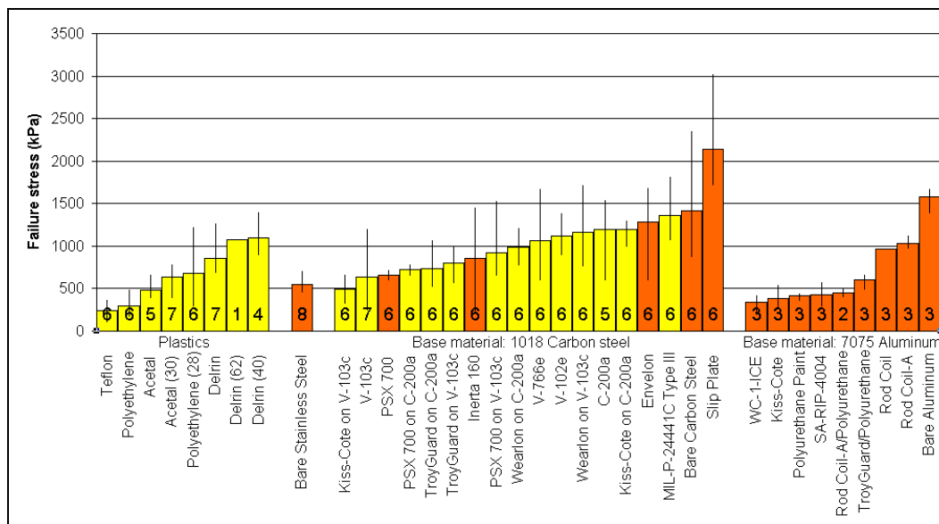
Figure 2. Shear adhesion strength of ice bonded to various materials and coatings. Yellow bars indicate new tests done under this study. Numbers in bars indicate sample size. Numbers in parentheses indicate number of days samples were weathered atop Mount Washington.
