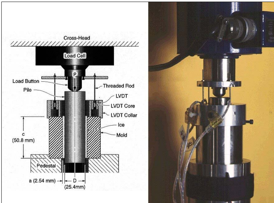
Figure 1. 0° cone test apparatus.
