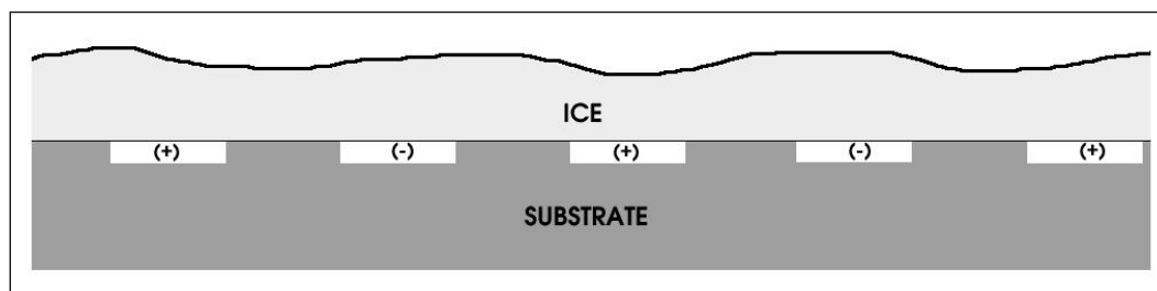
Figure 2. Electrode configuration used for removing ice from a flat surface by electrolysis.
