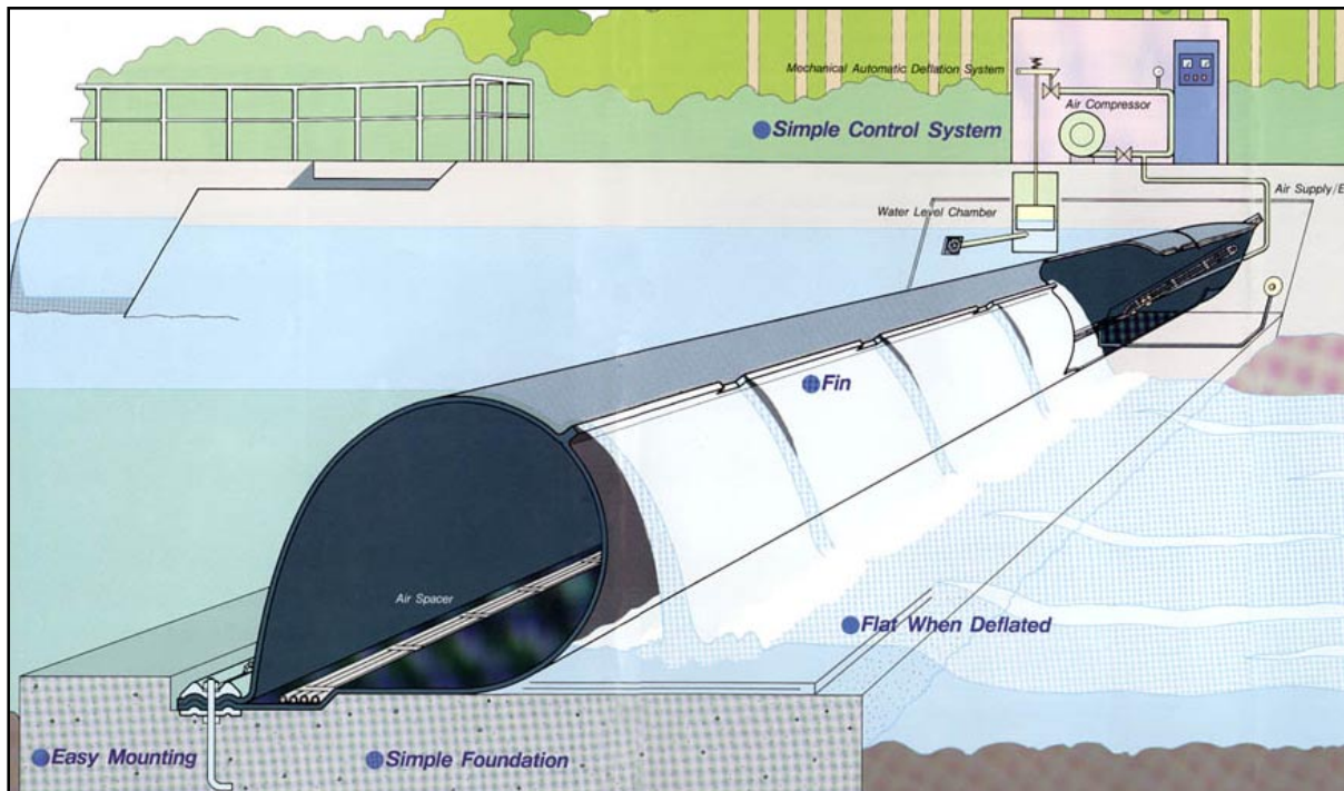
Figure 1. Cross section of an inflatable dam.
