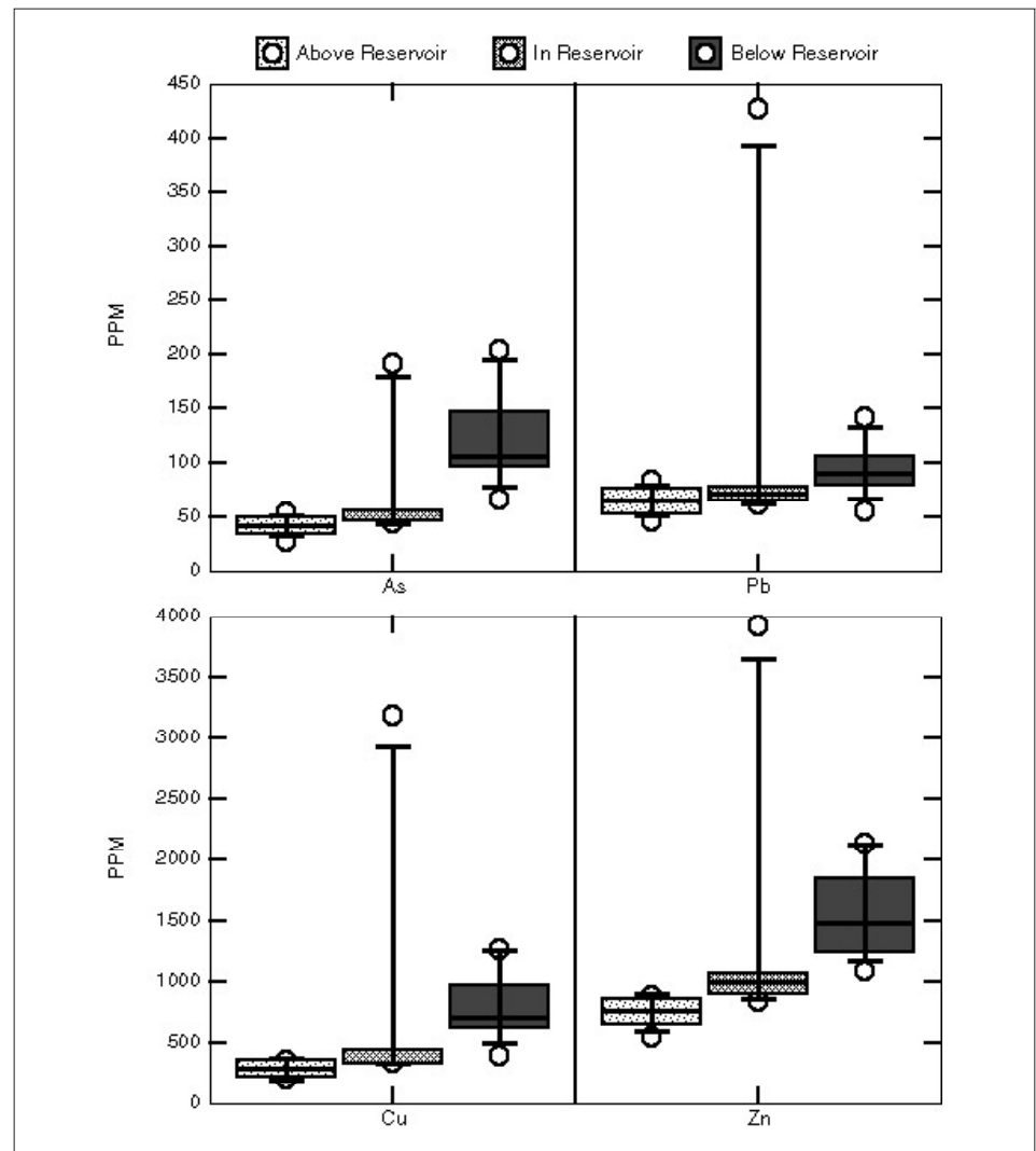
Figure 3. The erosion and scour of fluvial tailings can be dramatic during ice events. Here, metals concentrations measured in the Clark Fork River upstream and downstream from the Milltown Dam reservoir are shown following the ice jam event of February 1996. (After Moore and Landrigan 1999.)
