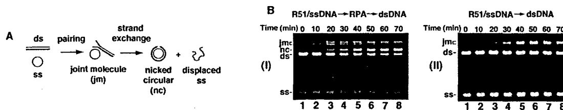
Figure 4. RPA dependence of human Rad51-mediated homologous DNA pairing and strand exchange. (A) Schematic of the homologous DNA pairing and strand exchange reaction. (B) Rad51-mediated DNA pairing and strand exchange reaction in the presence of RPA (panel I) and in the absence of RPA (panel II). In panel I RPA is added after Rad51 and ssDNA have been preincubated together.
