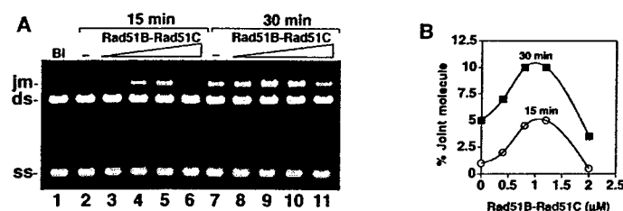
Figure 6. Rad51B-Rad51C complex stimulates DNA joint formation but does not replace RPA in DNA strand exchange reaction. (A) Rad51B-Rad51C complex and Rad51 were used in the strand exchange reaction in the absence of RPA. (B) Graphic representation of the results from the experiments in A.
