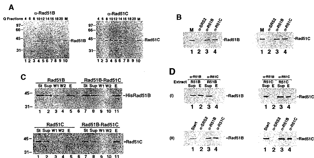
Figure 1. Rad51B and Rad51C form a complex in human cells. (A) HeLa cell extract was fractionated on a Q-Sepharose column and the fractions were run on a 11% gel and immunoblotted with the Rad51B and Rad51C antibodies. (B) Co-immunoprecipitation of Rad51B and Rad51C from the Q-Sepharose column fractions. The fractions were pooled and immunoprecipitated with protein A beads containing anti-Srs2, anti-Rad51B or anti-Rad51C antibodies. Proteins bound to the protein A beads were eluted by SDS treatment and analyzed. (C) Immunoprecipitation of Rad51B and Rad51C from yeast extracts. Rad51B and Rad51C were expressed individually and subjected to immunoprecipitation with protein A beads containing anti-Rad51B or anti-Rad51C antibodies. Unbound proteins (sup) and protein eluted of the beads (E) were analyzed on 11% gels (Panel I). In panel II, the yeast extracts expressing both the proteins were mixed and then immunoprecipitated. (D) Complex formation between 6-histidine tagged Rad51B and Rad51C. Extracts from insect cells expressing 6-Histidine tagged Rad51B, Rad51C or a mixture of the two were incubated with nickel-NTA agarose, followed by washing with imidazole. The starting material (st), unbound proteins (sup), washes (W1, W2) and eluates (E) were blotted with Rad51B antibody (upper panel) and Rad51C antibody (lower panel).
