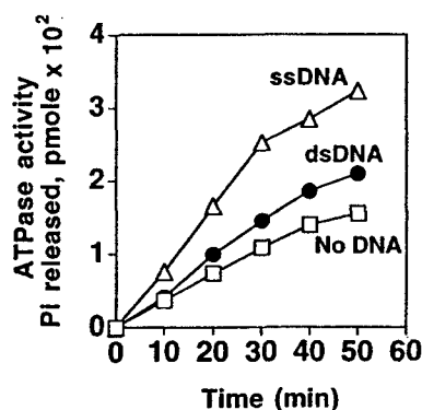
Figure 3. The ATPase activity of Rad51B-Rad51C complex was studied with ssDNA, dsDNA and without the addition of DNA.
