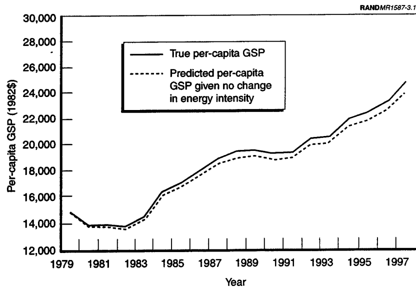
Figure 3.1—Actual GSP Per Capita and GSP Per Capita in the Case of Constant Energy Intensity
