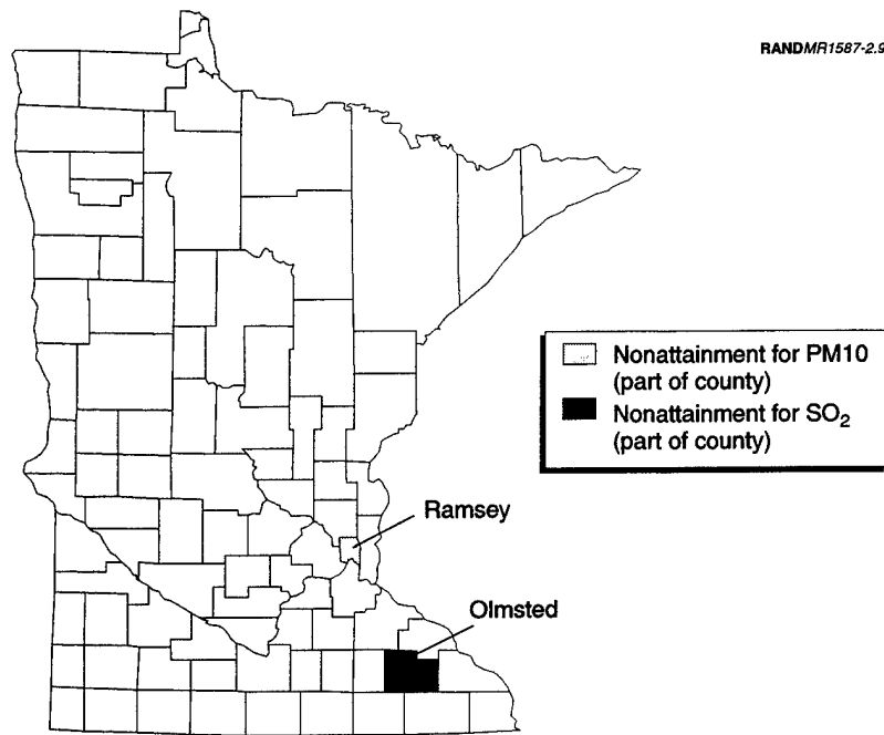
Figure 2.9—Minnesota Nonattainment Areas for PM10 and SO 2 by County in 2001
