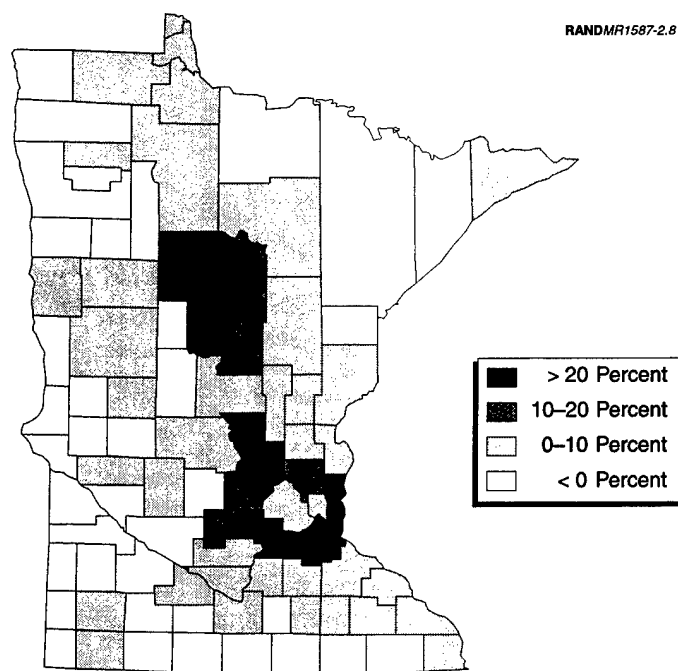
Figure 2.8—Forecasted Minnesota Population Growth by County, 2000–2015
