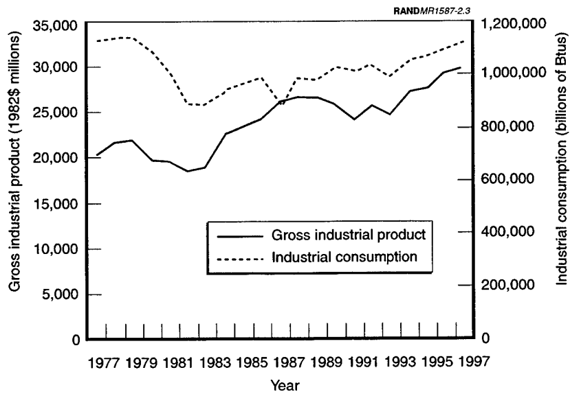
Figure 2.3—Total Industrial Consumption and Gross Industrial Product, Minnesota
