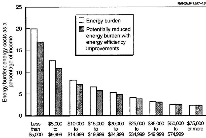
Figure 4.6—Minnesota Household Energy Expenditure as a Percentage of Income and Potential Reduction of Energy Burden with Energy Efficiency Improvements
