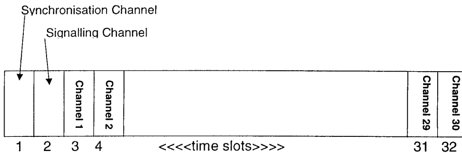
Figure 5: Sub-Structure of the Eurocom Loop Group
