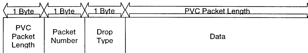
Figure 6: Structure of PVC Ethernet Packet Payload
