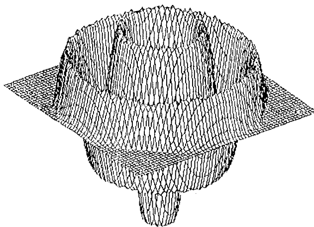
Fig. 4 — Results of a sinusoidal point source input to the central node of a two-dimensional TLM mesh. ©P.A. Willison, 1992, used by permission.
