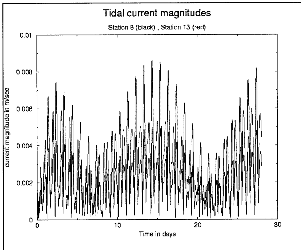
Figure 15. Tidal current magnitude reconstruction time series for 28 days, stas 8 and 13
