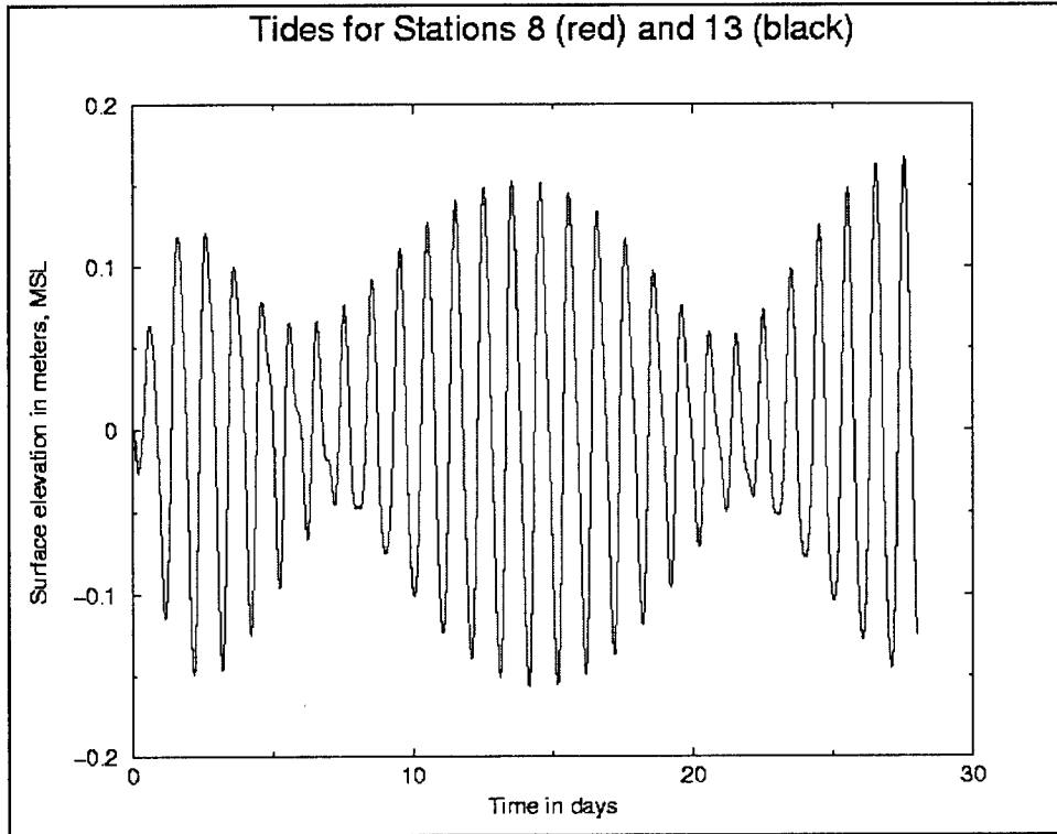
Figure 14. Tidal elevation reconstruction time series for 28 days, stas 8 and 13
