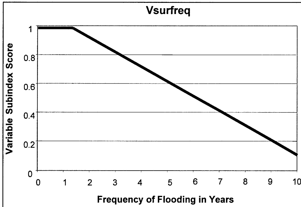
Figure 37. Function 7: Relationship of surface flood recurrence and the corresponding V_{SURFREQ} Variable Subindex Score
