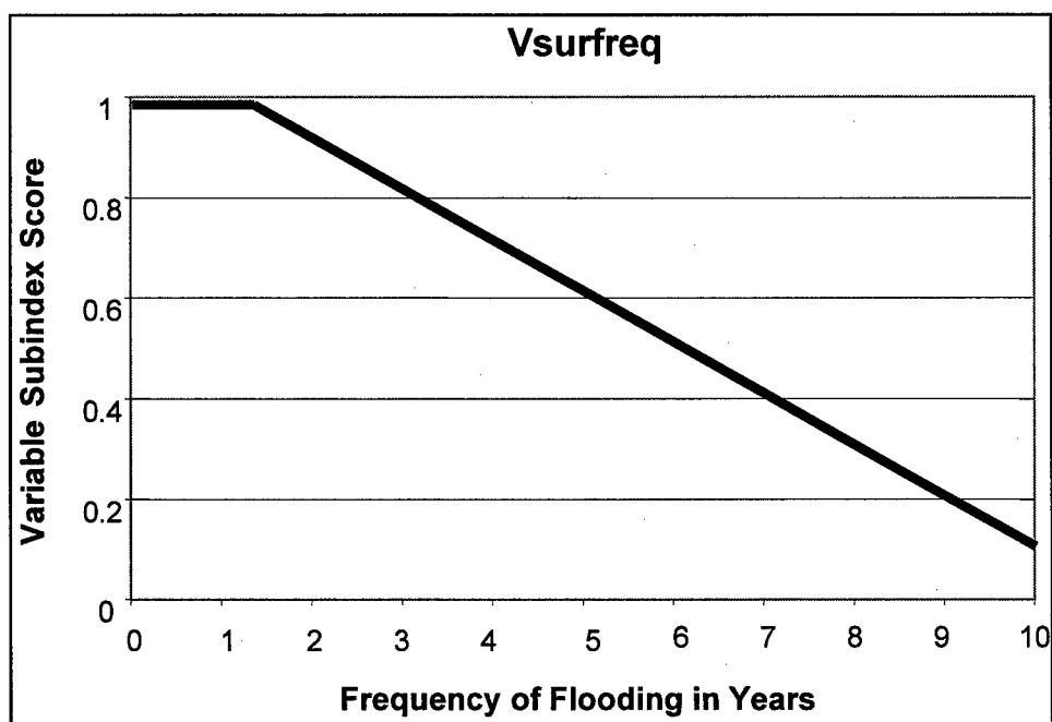
Figure 21. Function 3: Relationship of surface flood recurrence and the corresponding V_{SURFREQ} Variable Subindex Score
