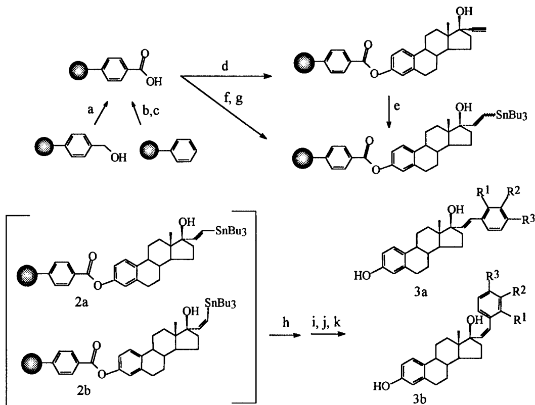
Scheme 1. Reagent: (a) Jones reagent ( \text{H}_2\text{Cr}_2\text{O}_4 , \text{H}_2\text{SO}_4 , acetone); (b) n -BuLi, TMEDA, cyclohexane, 50^\circ\text{C} ; (c) Dry ice, THF; (d) 17 \alpha -Ethynyl estradiol, DCC, DMAP, \text{CH}_2\text{Cl}_2 ; (e) \text{HSnBu}_3 , \text{Et}_3\text{B} , THF, 50 – 60^\circ\text{C} ; (f) 17 \alpha -Ethynyl estradiol, \text{HSnBu}_3 , \text{Et}_3\text{B} , THF, 50 – 60^\circ\text{C} ; (g) DCC, DMAP, \text{CH}_2\text{Cl}_2 ; (h) R-Aryl-X, Pd ( \text{PPh}_3 ) _4 , BHT, toluene, \text{N}_2 , reflux; (i) 5 N-NaOH in \text{CH}_3\text{OH} -Dioxane (1:3); (j) 5%- \text{CH}_3\text{COOH} ; (k) 10%- \text{NaHCO}_3 .
