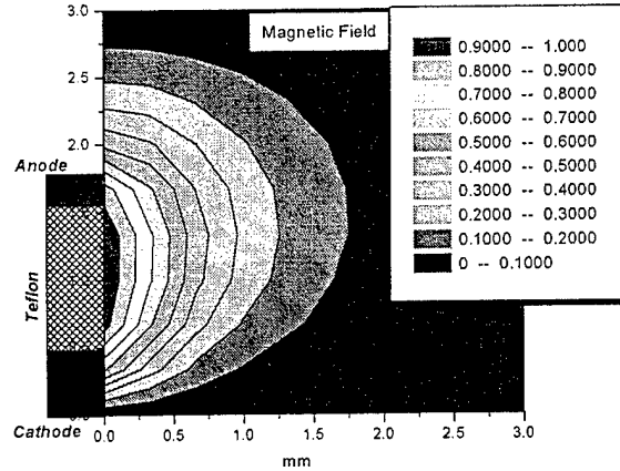
Figure 7. Magnetic field distribution in the near field of a 3.6 mm diameter micro-PPT
