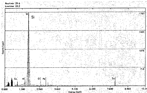
Figure 3. Image and XEDS results for the Area 2. The main peak corresponds to Silicon
