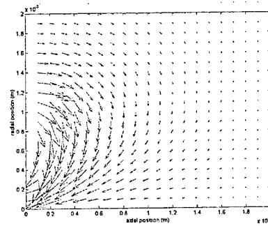
Figure 8. Current distribution in the near field of a 3.6 mm diameter micro-PPT
