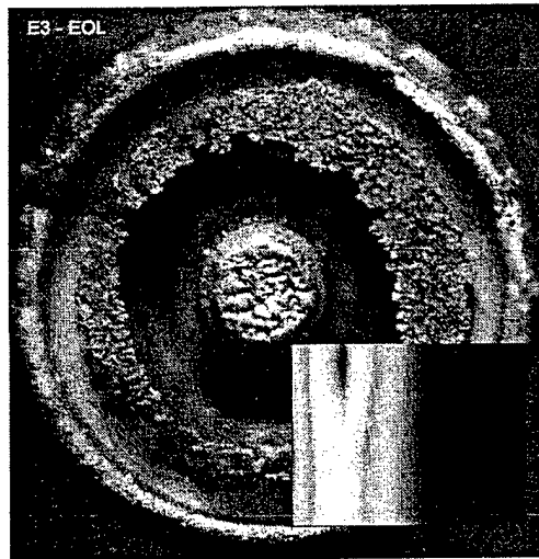
Figure 12. Teflon™ surface photo (Ref. 6) and the Teflon™ surface temperature field and the ablation rate in the case of 3.6 mm diameter micro-PPT
