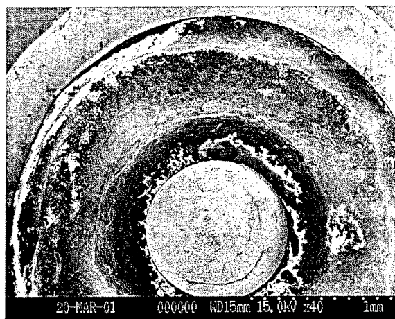
Figure 4. Propellant surface of 3.6 mm diameter micro-PPT
