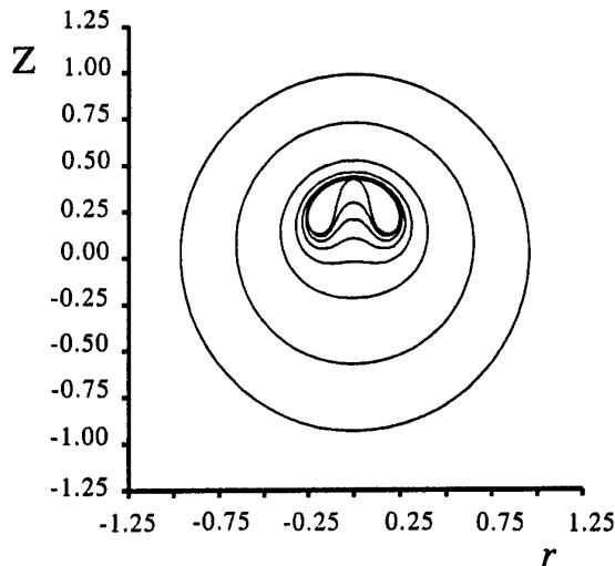
Figure 6: The collapse of the bubble created by detonating 343 kg TNT at a depth of 154.2 m. The distance scale is non-dimensional with respect to the maximum bubble radius, equal to 4.13 m. The times, in milliseconds, corresponding to the bubble shapes are: 136.6, 188.0, 204.7, 208.5, 210.1, 211.1, 211.9, 213.1.
