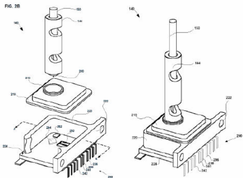
Figure 6. Outline drawing of the package assembly.
