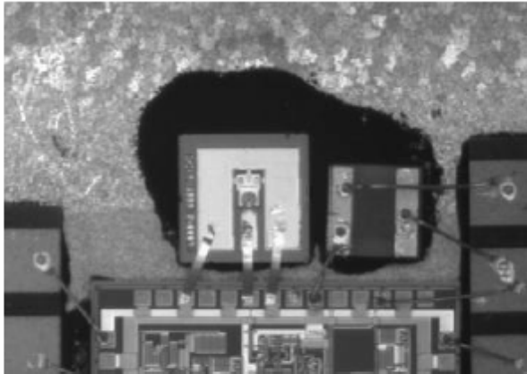
GaAs PIN structure 750 \mu\text{m} square die 65 \mu\text{m} active area
