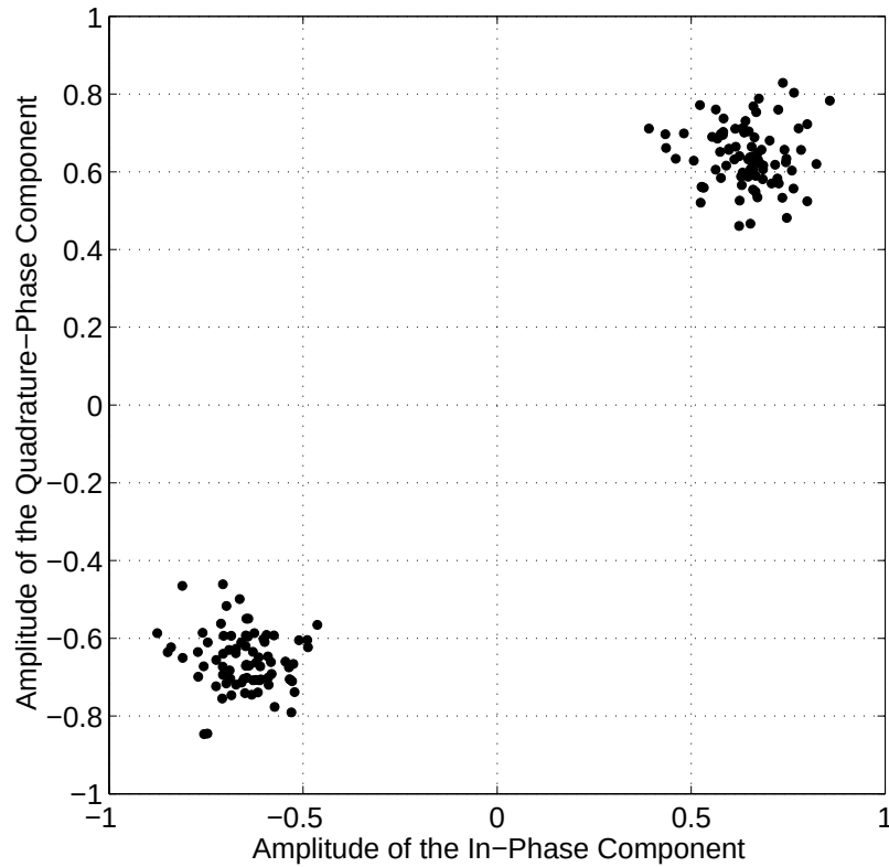
Figure 36. Typical received signal constellation, after despreading and before differential decoding, in the ideal AWGN channel (this example is for an E_b / N_0 = 18 \text{ dB} ( SNR \approx -10 \text{ dB} )).
