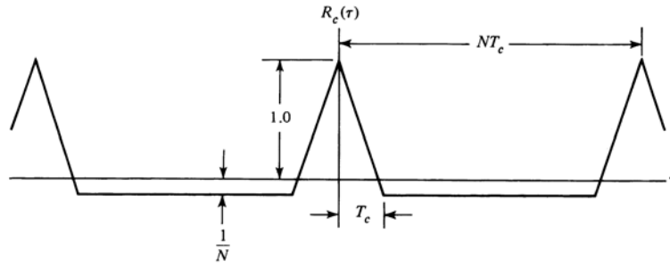
Figure 14. The autocorrelation function for an arbitrary m-sequence [From Ref. 14].
