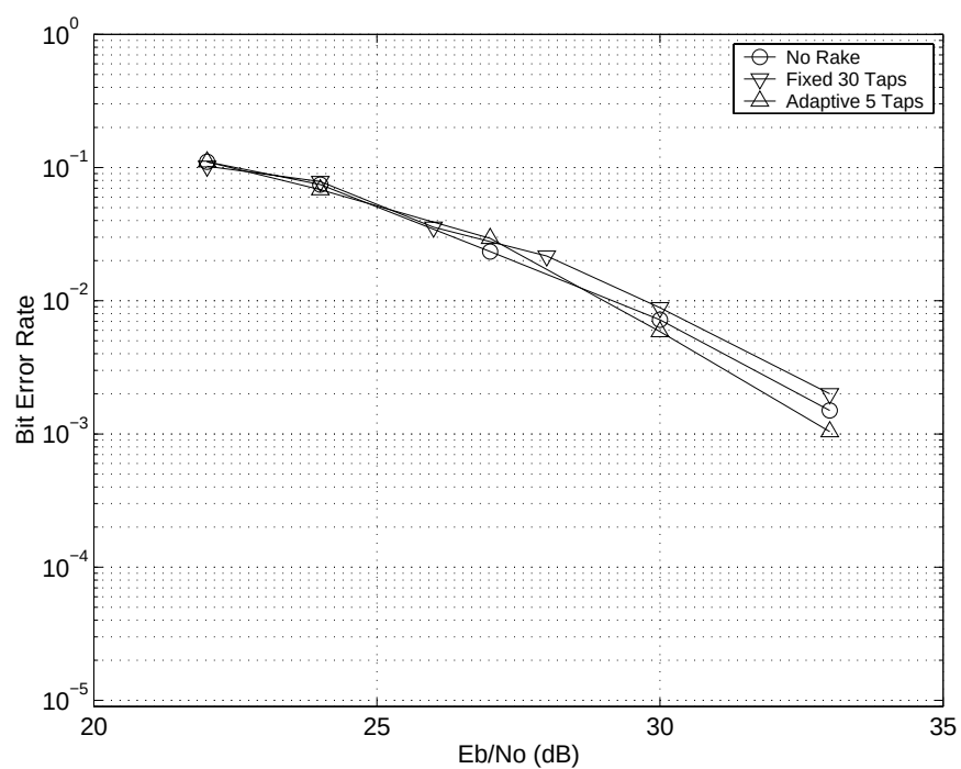
Figure 55. Bit error rate for the RAKE receiver using SDD and 5 adaptively spaced taps located at the dominant multipath arrivals, in the modeled channel.
