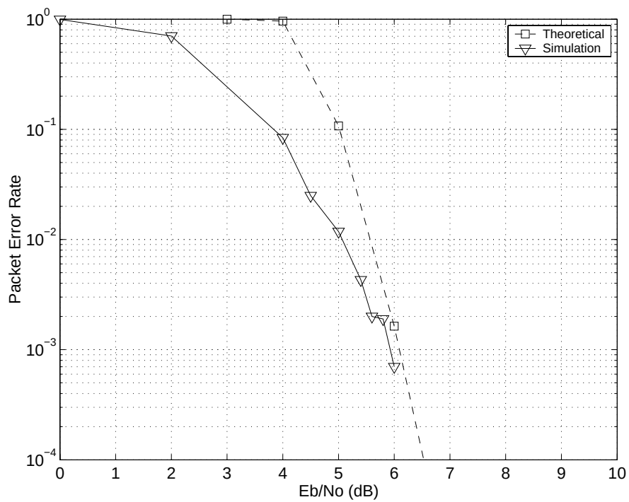
Figure 45. Packet error rate in an AWGN channel with SDD.
