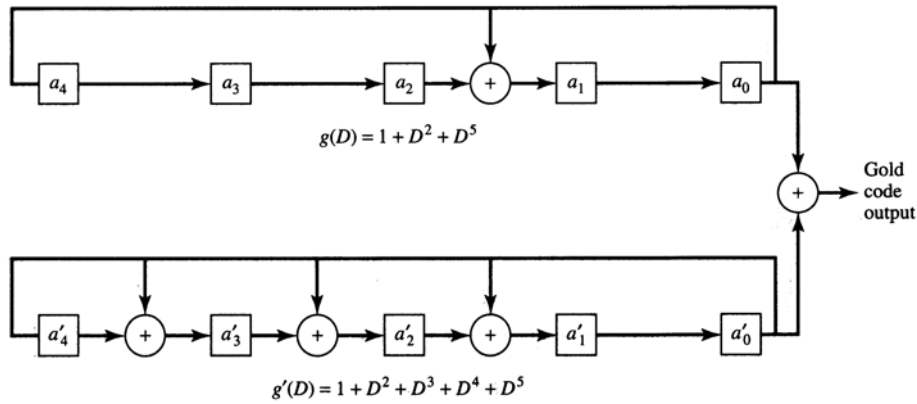
Figure 15. A typical Gold code generator [From Ref. 14].
