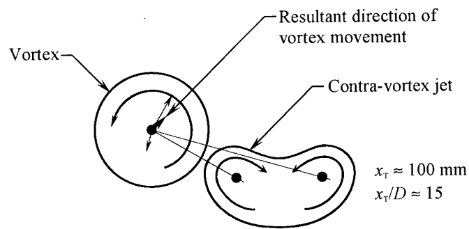
Figure 23. Cross sections of a vortex and a jet showing the direction of vortex movement. Circular jet, U_j = 1.2 \text{ m/s} , contra-vortex jet, \theta = -90^\circ .
