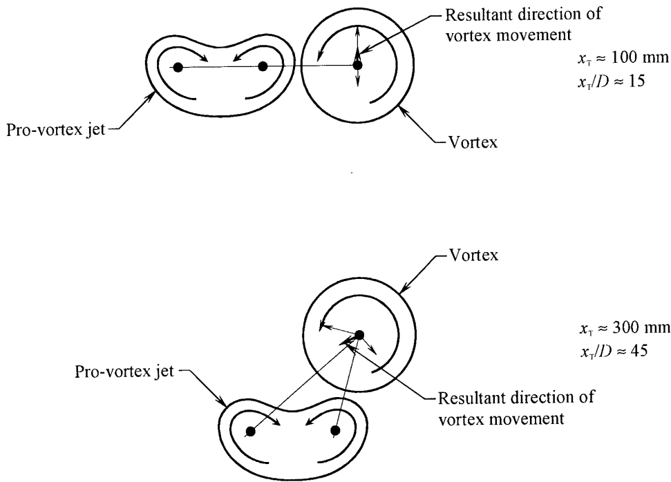
Figure 18. Cross sections of a vortex and a jet showing the direction of vortex movement. Circular jet, U_j = 0.4 \text{ m/s} , pro-vortex jet, \theta = -90^\circ .
