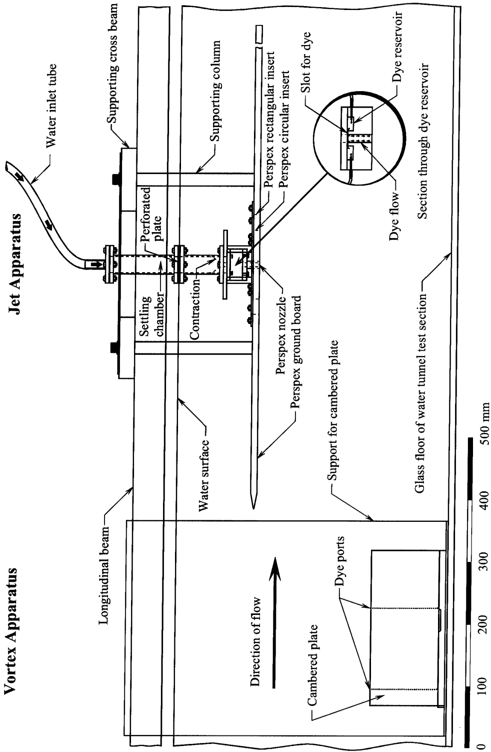
Figure 4. Diagrammatic representation of the vortex apparatus and the jet apparatus; (a) side view.
