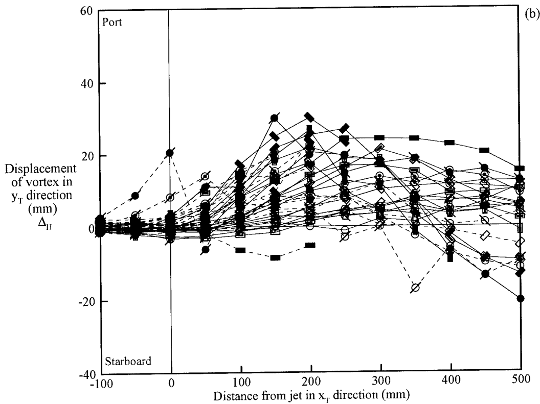
Figure 9. Effect of different jets on vortex displacement: (a) side view; (b) plan view. See Table 1 for an explanation of the symbols used for the different jets.
