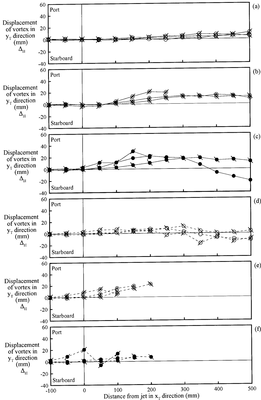
Figure 31. Effect of jet pitch angle on vortex displacement –plan views:
