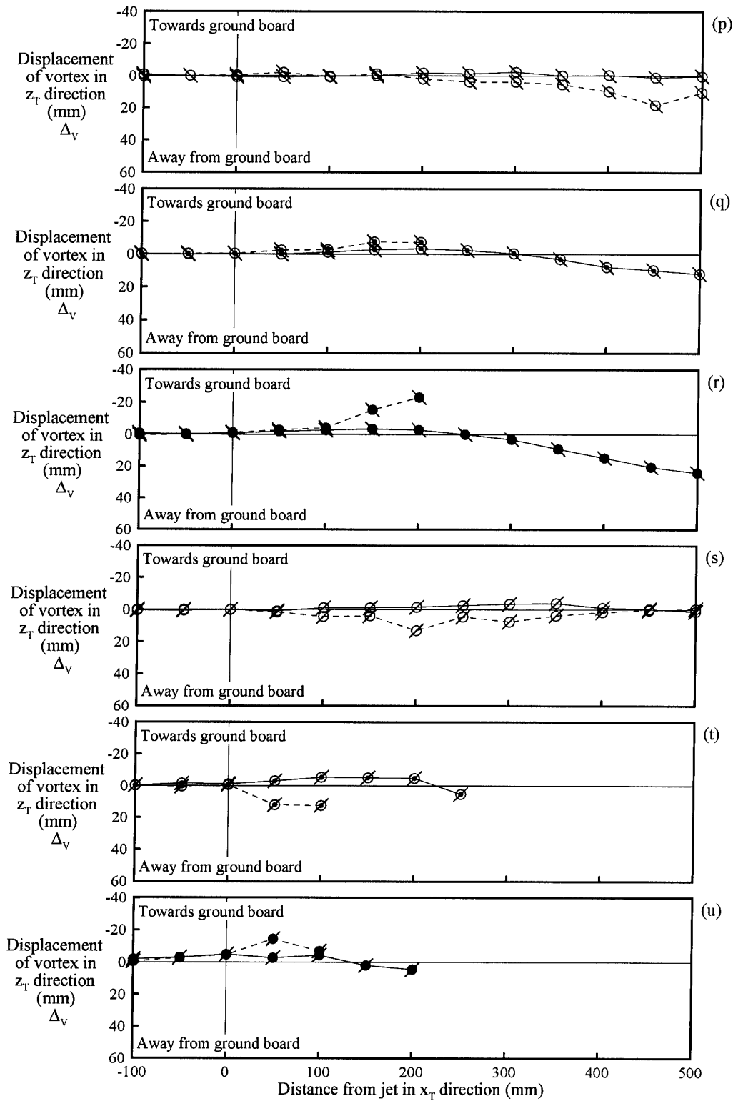
Figure 28 cont'd. Effect of jet location on vortex displacement –side views: (p) circular jet, U_j = 0.4 \text{ m/s} , \theta = -45^\circ ; (q) circular jet, U_j = 0.8 \text{ m/s} , \theta = -45^\circ ; (r) circular jet, U_j = 1.2 \text{ m/s} , \theta = -45^\circ ; (s) circular jet, U_j = 0.4 \text{ m/s} , \theta = -135^\circ ; (t) circular jet, U_j = 0.8 \text{ m/s} , \theta = -135^\circ ; (u) circular jet, U_j = 1.2 \text{ m/s} , \theta = -135^\circ See Table 1 for an explanation of the symbols used for the different jets.
