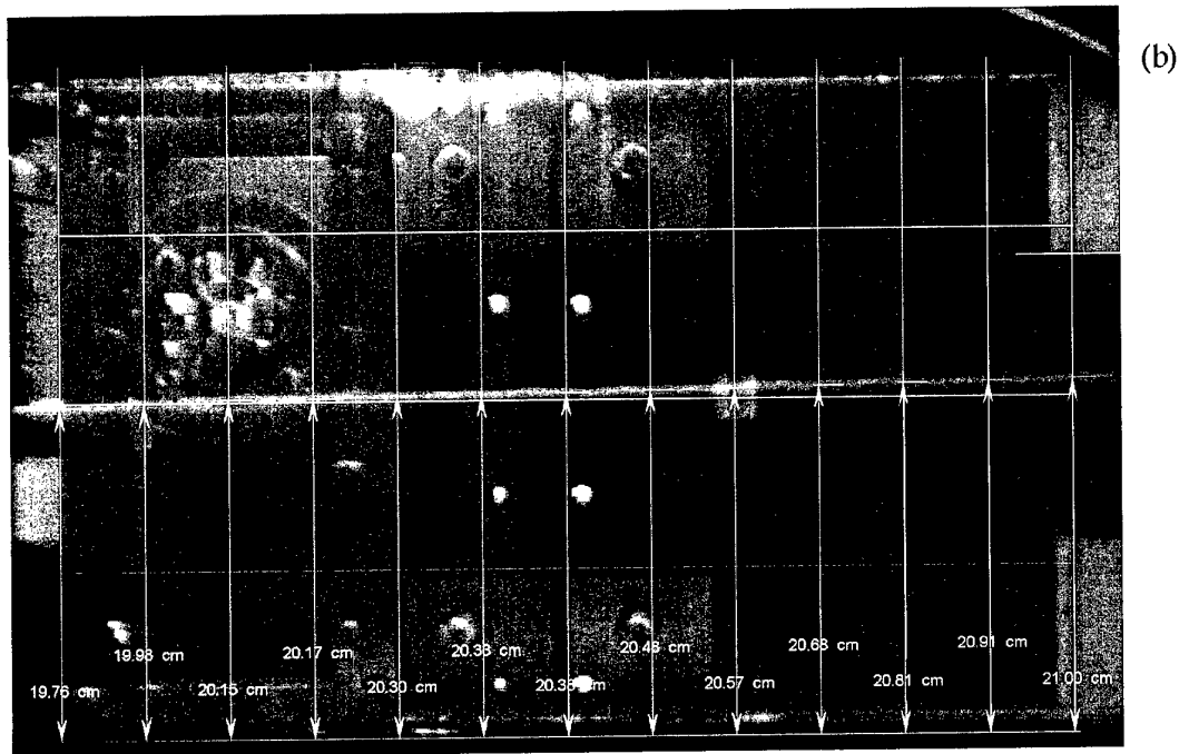
Figure 6. Typical images of cores of unperturbed vortices: (a) side view; (b) plan view.
