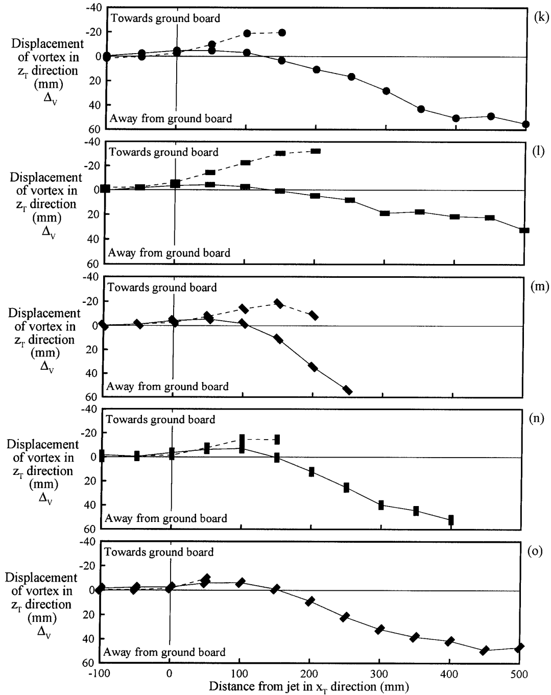
Figure 28 cont'd. Effect of jet location on vortex displacement –side views: (k) circular jet, U_J = 1.2 \text{ m/s} , \theta = -90^\circ ; (l) rectangular jet \phi = 0^\circ , U_J = 1.2 \text{ m/s} , \theta = -90^\circ ; (m) rectangular jet \phi = 45^\circ , U_J = 1.2 \text{ m/s} , \theta = -90^\circ ; (n) rectangular jet \phi = 90^\circ , U_J = 1.2 \text{ m/s} , \theta = -90^\circ ; (o) rectangular jet \phi = 135^\circ , U_J = 1.2 \text{ m/s} , \theta = -90^\circ . See Table 1 for an explanation of the symbols used for the different jets.
