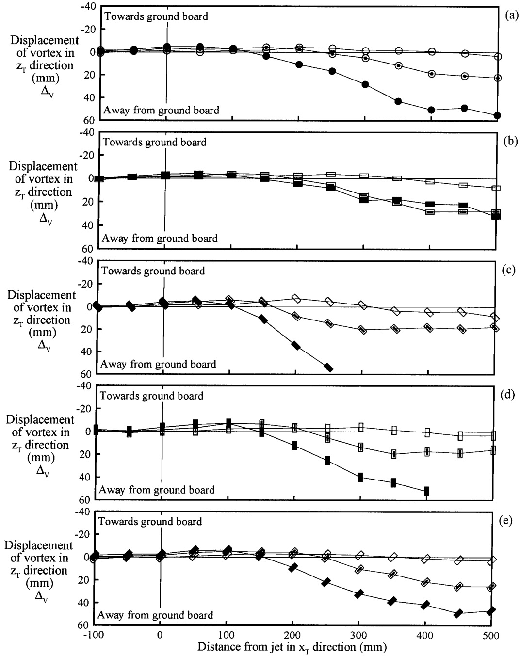
Figure 26. Effect of jet velocity on vortex displacement –side views: (a) circular jet, pvj, \theta = -90^\circ ; (b) rectangular jet \phi = 0^\circ, pvj, \theta = -90^\circ ; (c) rectangular jet \phi = 45^\circ, pvj, \theta = -90^\circ ; (d) rectangular jet \phi = 90^\circ, pvj, \theta = -90^\circ ; (e) rectangular jet \phi = 135^\circ, pvj, \theta = -90^\circ .
