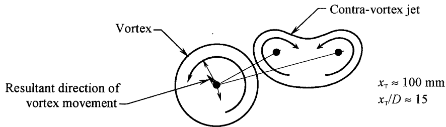
Figure 21. Cross sections of a vortex and a jet showing the direction of vortex movement. Circular jet, U_j = 0.8 m/s, contra-vortex jet, \theta = -90^\circ .
