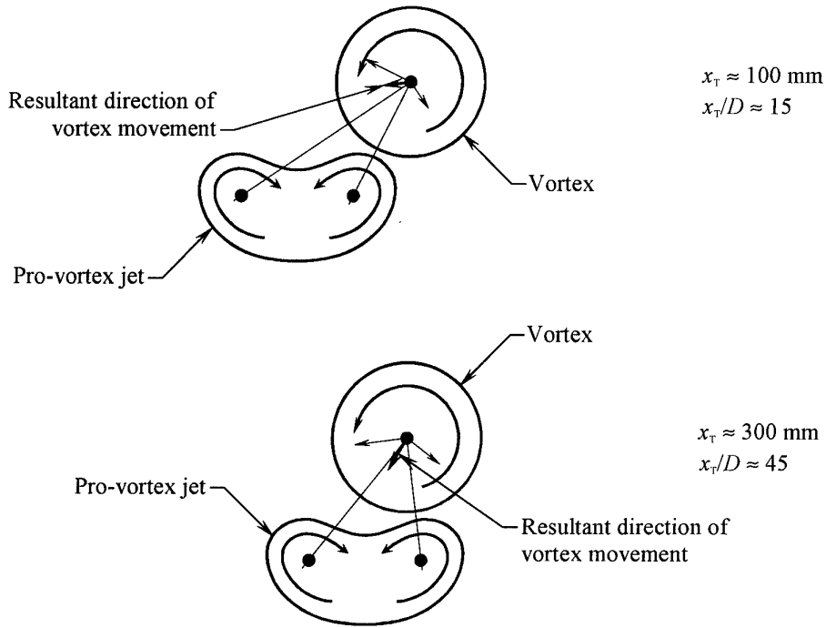
Figure 20. Cross sections of a vortex and a jet showing the direction of vortex movement. Circular jet, U_j = 0.8 m/s, pro-vortex jet, \theta = -90^\circ .
