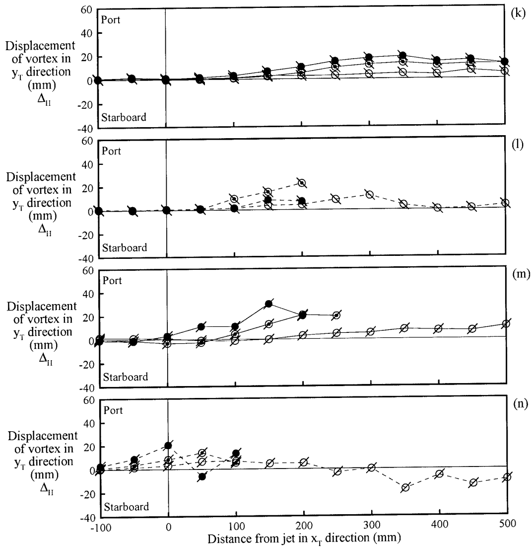
Figure 27 cont'd. Effect of jet velocity on vortex displacement: -plan views.
