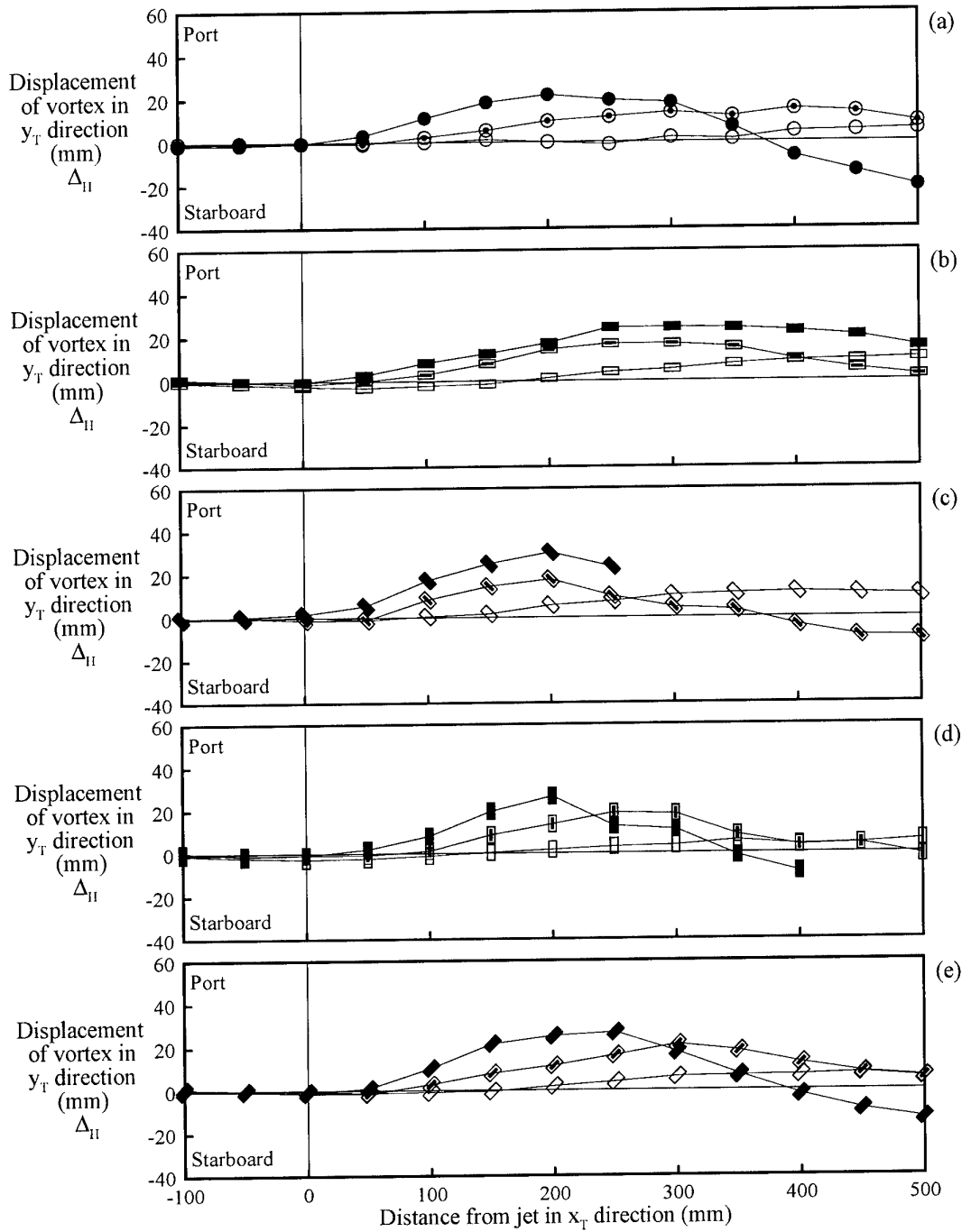
Figure 27. Effect of jet velocity on vortex displacement – plan views: (a) circular jet, pvj, \theta = -90^\circ ; (b) rectangular jet \phi = 0^\circ, pvj, \theta = -90^\circ ; (c) rectangular jet \phi = 45^\circ, pvj, \theta = -90^\circ ; (d) rectangular jet \phi = 90^\circ, pvj, \theta = -90^\circ ; (e) rectangular jet \phi = 135^\circ, pvj, \theta = -90^\circ .
