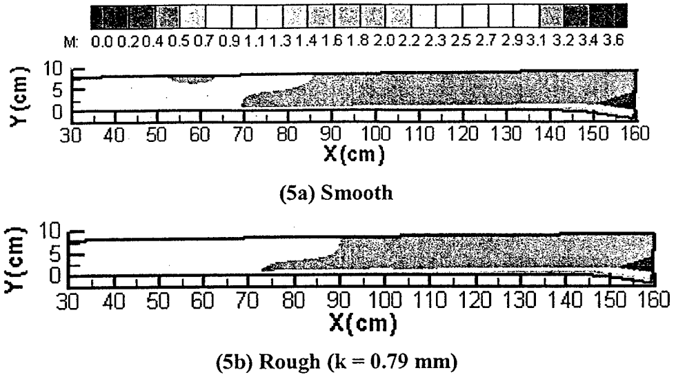
Figure 5 Mach Distributions within the FPG Test Sections
