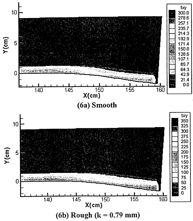
Figure 6 Shear Stress Distributions (Algebraic Models)
