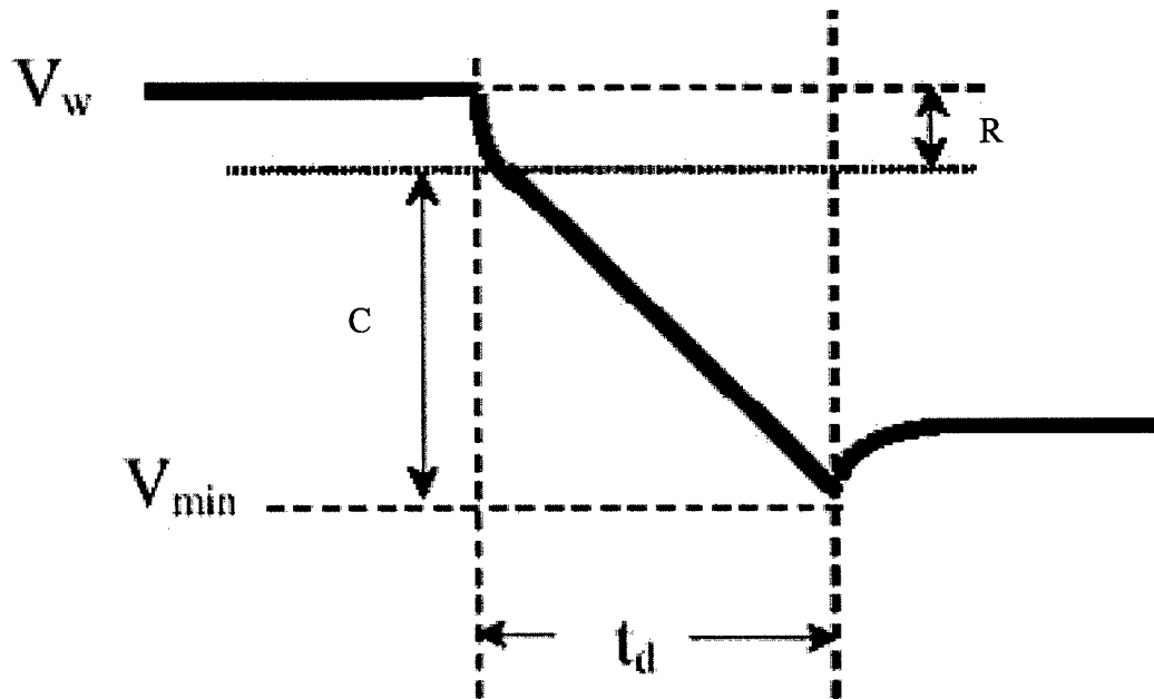
Discharge Profile
