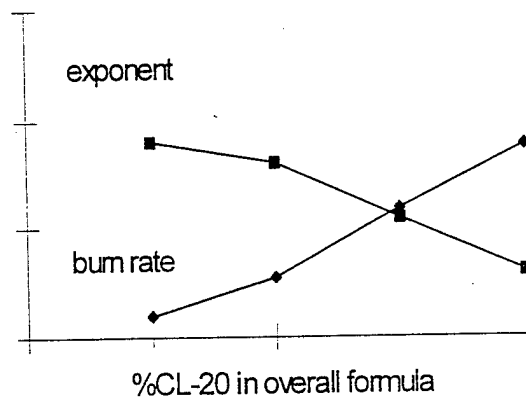
Figure 1. Ballistic Properties of High Energy CL-20 Propellants
