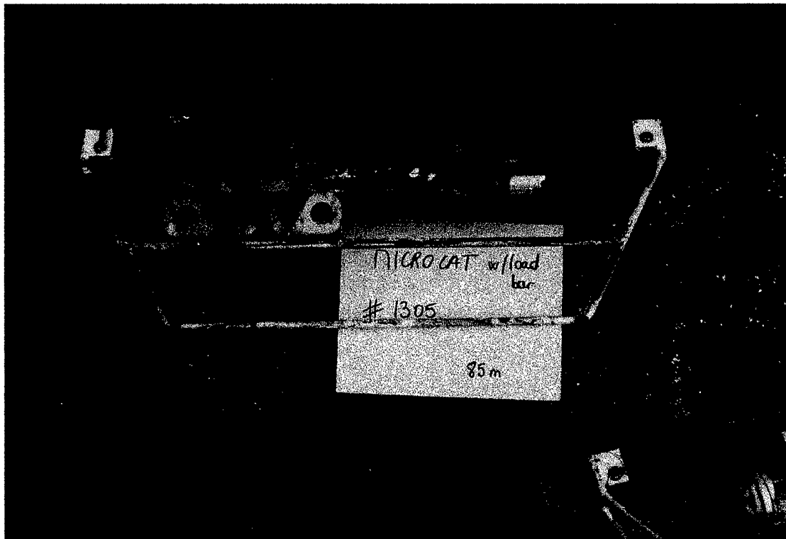
Figure 35: MICROCAT instrument at 85 m depth.
