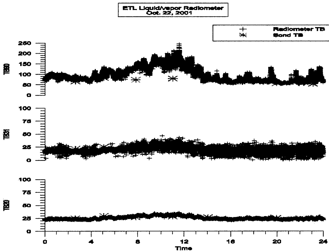
Figure 30: Raw brightness temperatures from the three channels of the microwave radiometer.
