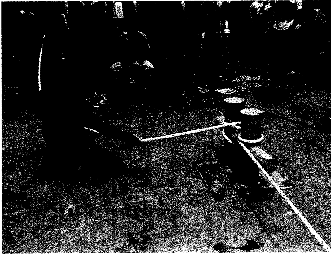
Figure 73: Position of the line handler and assistant.
