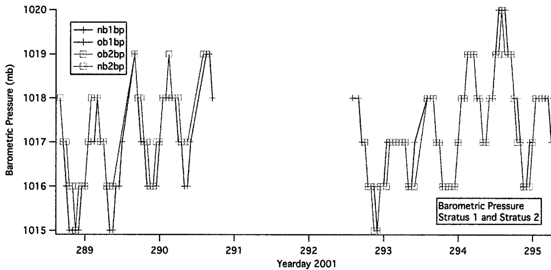
Figure 43: Comparison of barometric pressure (mb) data from the two IMET systems on the Stratus 1 (left) and 2 (right) buoys.
