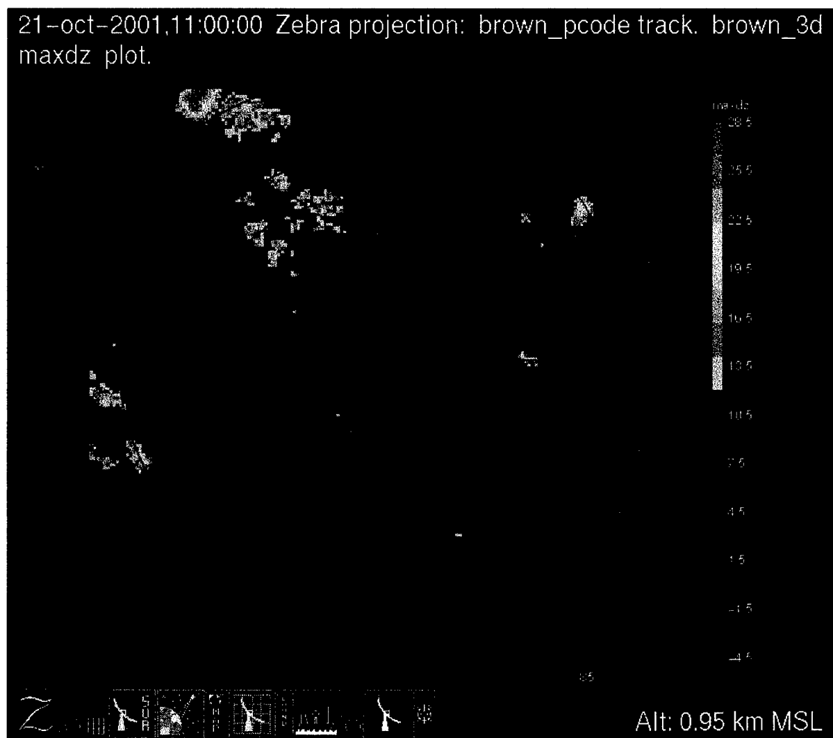
Figure 22: Horizontal cross-section of C-band radar data from 11 UTC October 21 (Day 294).
