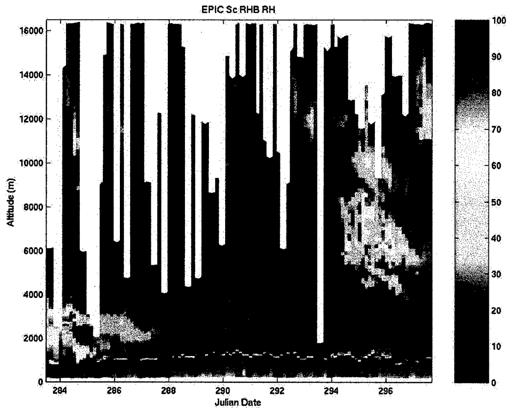
Figure 24: Relative humidity time-height plot from upper-air soundings every three hours throughout Leg 2.
