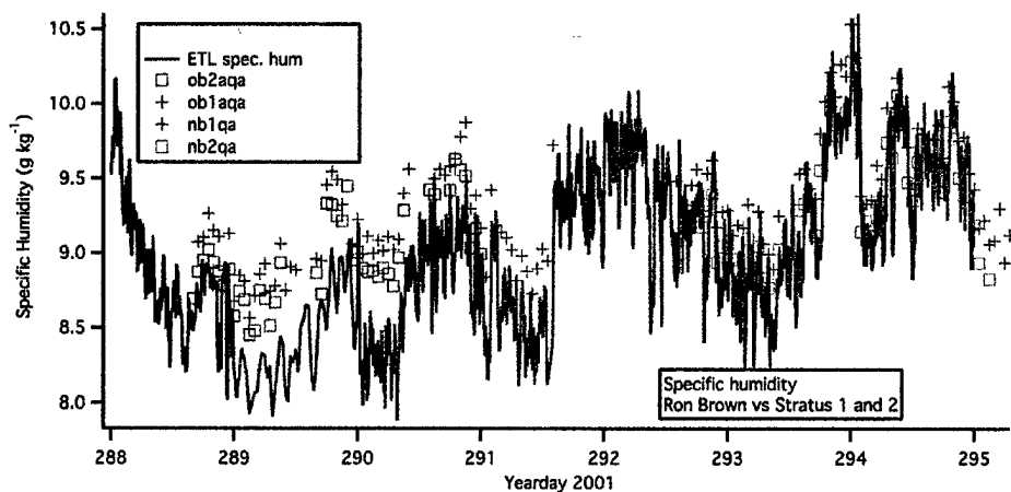
Figure 51: Comparison of specific humidity (g/kg) from the two IMET systems on the Stratus 1 (left) and 2 (right) buoys with ETL data.
