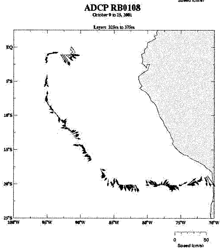
Figure 68: ADCP vectors for vertical layers of 275m to 375m.
