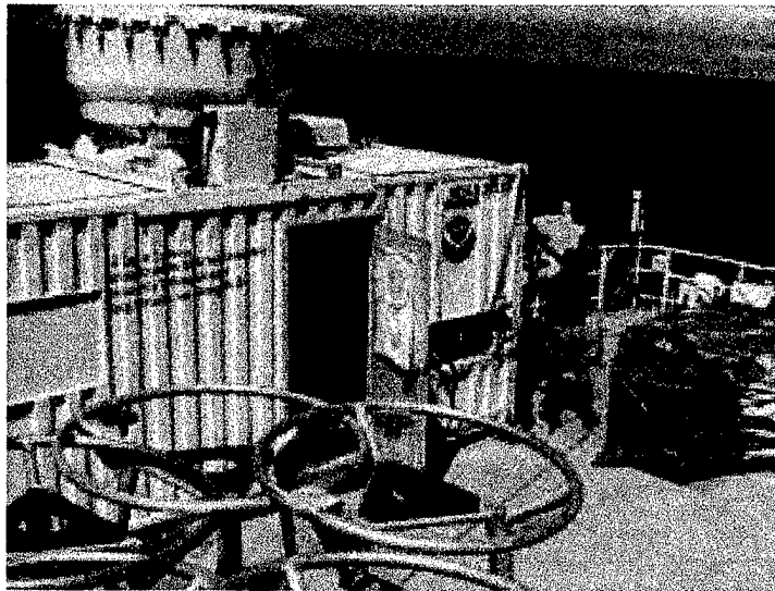
Figure 26: Photo of the MMCR Package showing the radar antenna (roof) and MWR reflector (right side).
