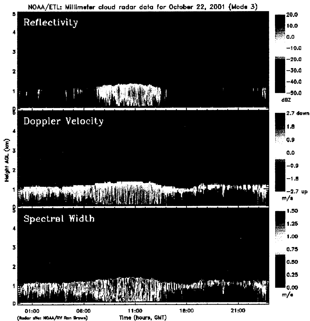
Figure 27: Example of radar reflectivity (upper panel), Doppler velocity (middle panel) and the spectral width (bottom panel) of the Doppler spectrum for a 24 hour period.
