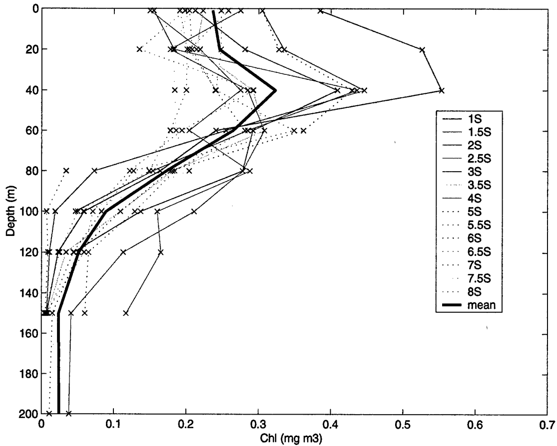
Figure 8: Chlorophyll profiles in the upper 200 m at the stations from 1° to 8° S.
