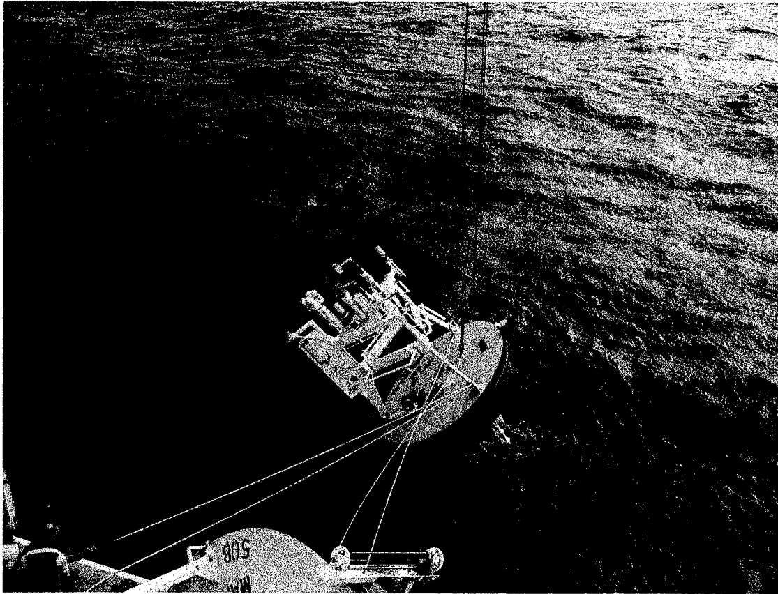
Figure 70: Three slip lines rigged on the discus to maintain constant swing control during the lift.
