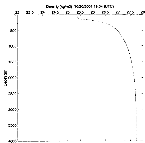
Figure 56: CTD Station 24, cast # 68.
