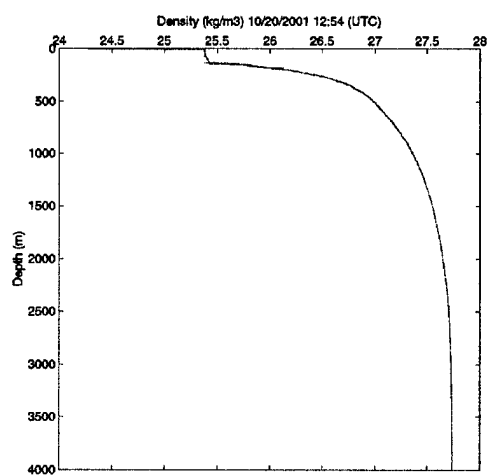
Figure 55: CTD Station 21, cast # 67.
