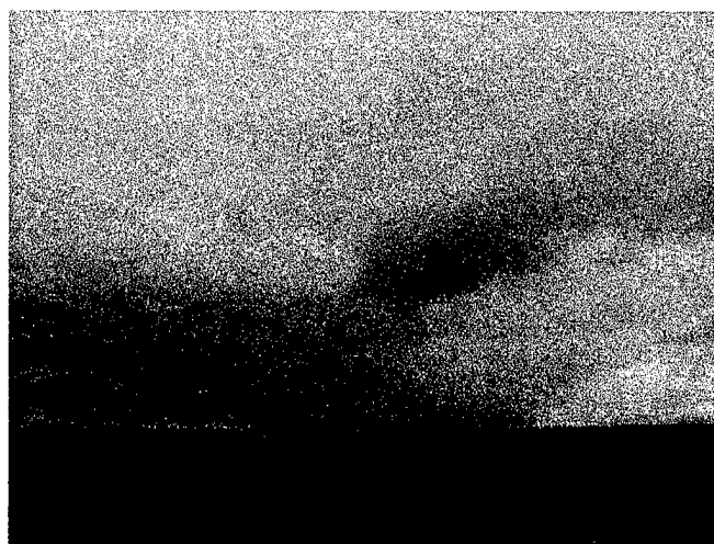
Figure 25: Cloud photo looking eastward at about 11:15 UTC on October 21 (Day 294).
