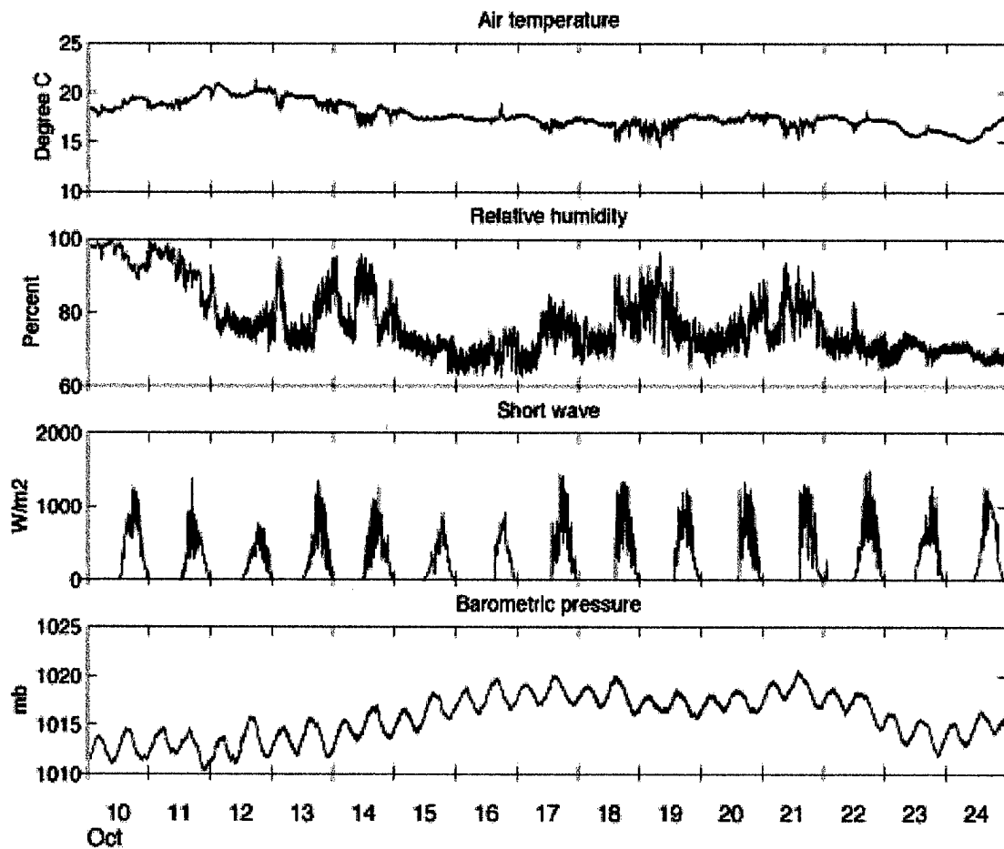
Figure 59: Air Temperature, Relative Humidity, Short-wave and Barometric pressure from Shipboard IMET sensors.
