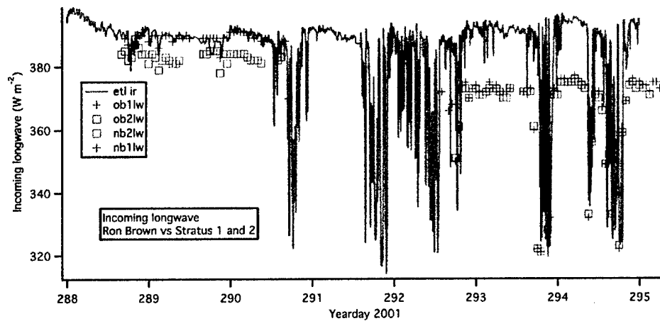
Figure 50: Comparison of incoming long-wave ( \text{W/m}^2 ) from the two IMET systems on the Stratus 1 (left) and 2 (right) buoys with ETL data.
