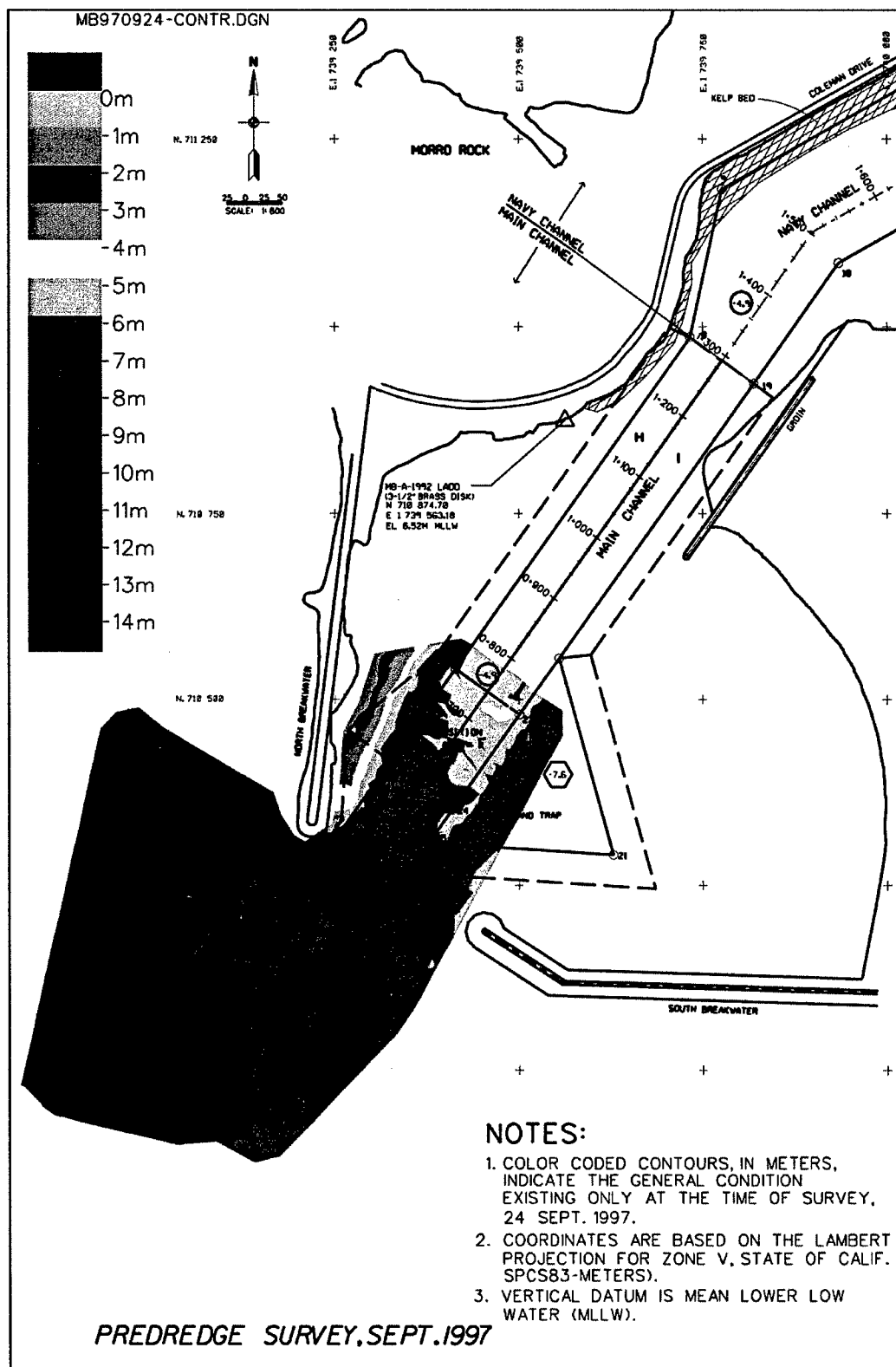
Figure A6. Bathymetry at Morro Bay entrance, 24 September 1997
