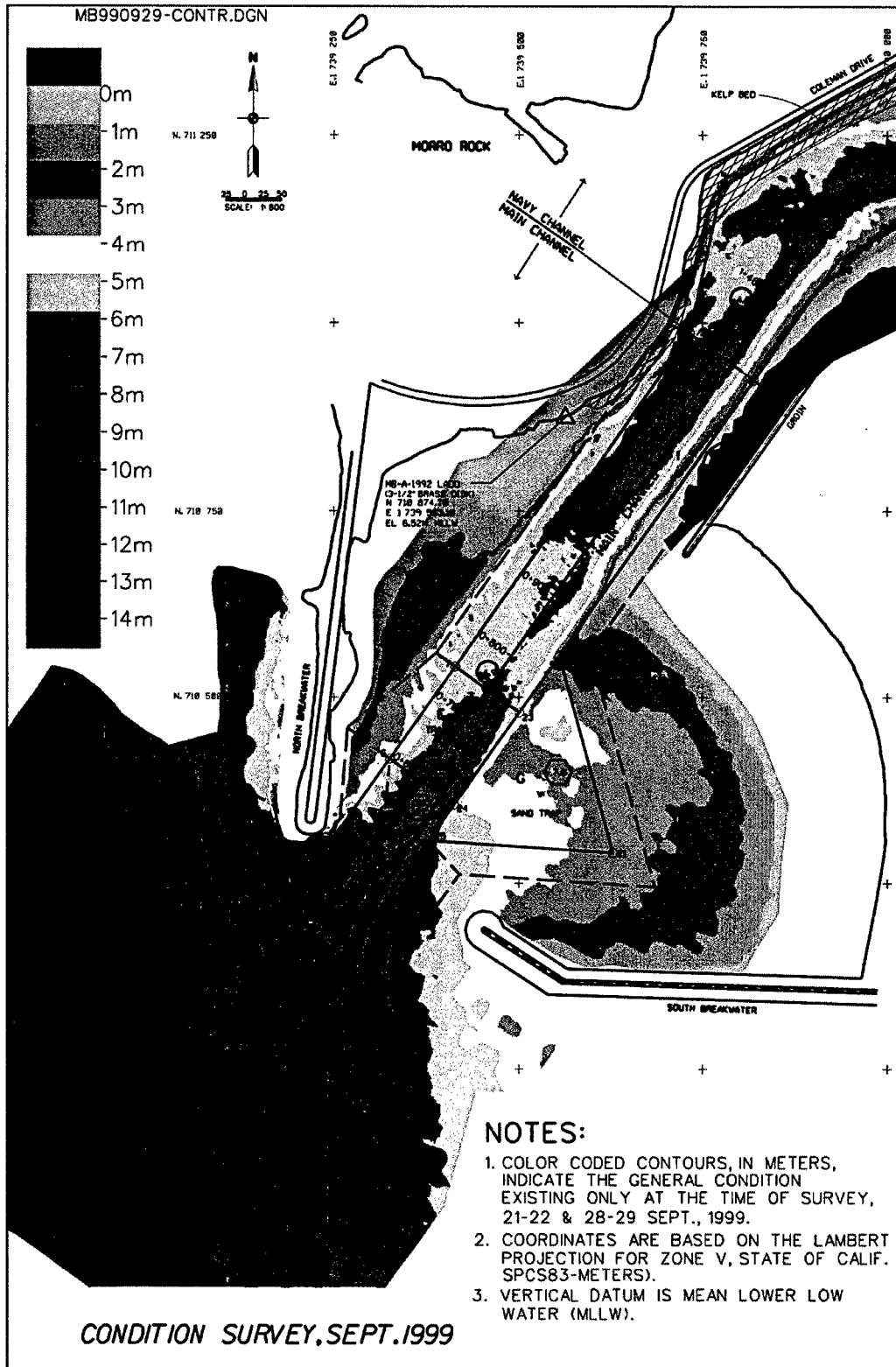
Figure A16. Bathymetry at Morro Bay entrance, 21-22 and 28-29 September 1999
