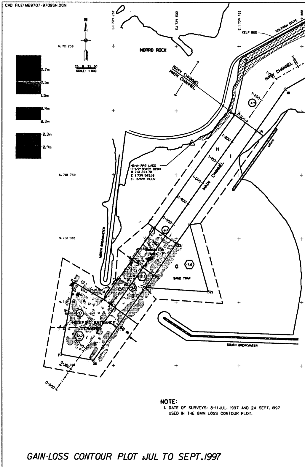
Figure C2. Bathymetry changes at Morro Bay entrance between 8-11 July 1997 and 24 September 1997
