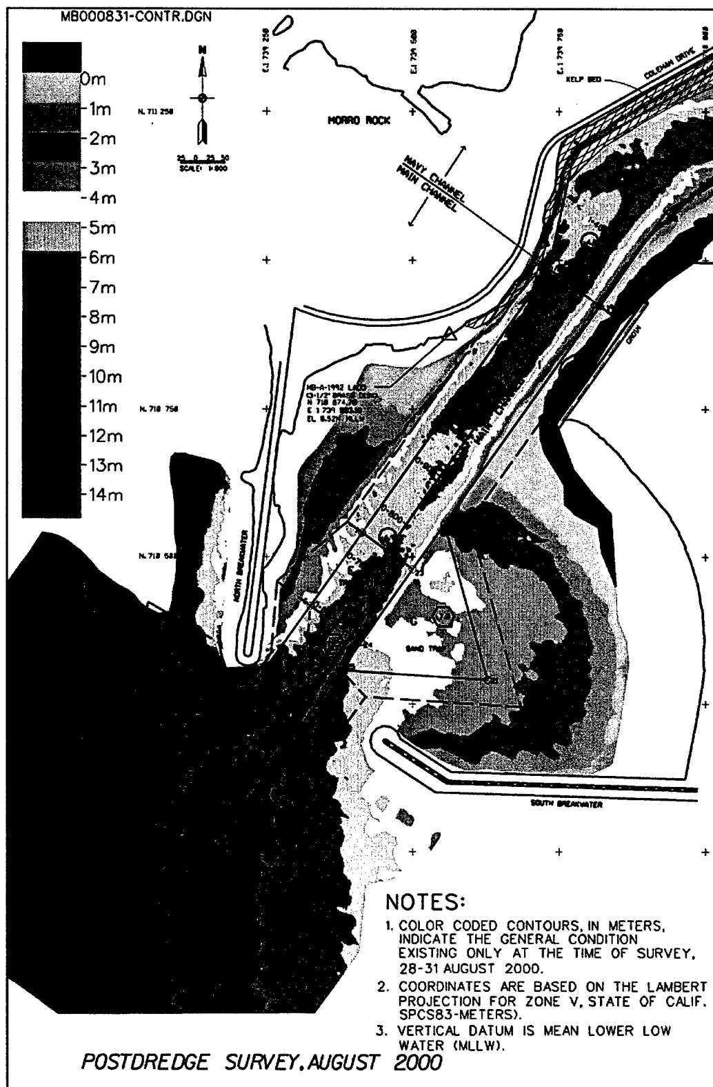
Figure A18. Bathymetry at Morro Bay entrance, 28-31 August 2000
