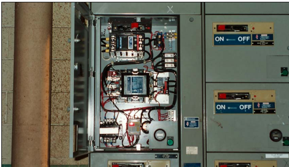
Figure 21. MCC starter bucket for chromic acid pump, with power monitor installed.
