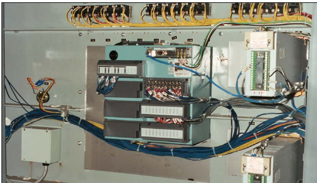
Figure 13. DX200 Back Panel Wiring.
