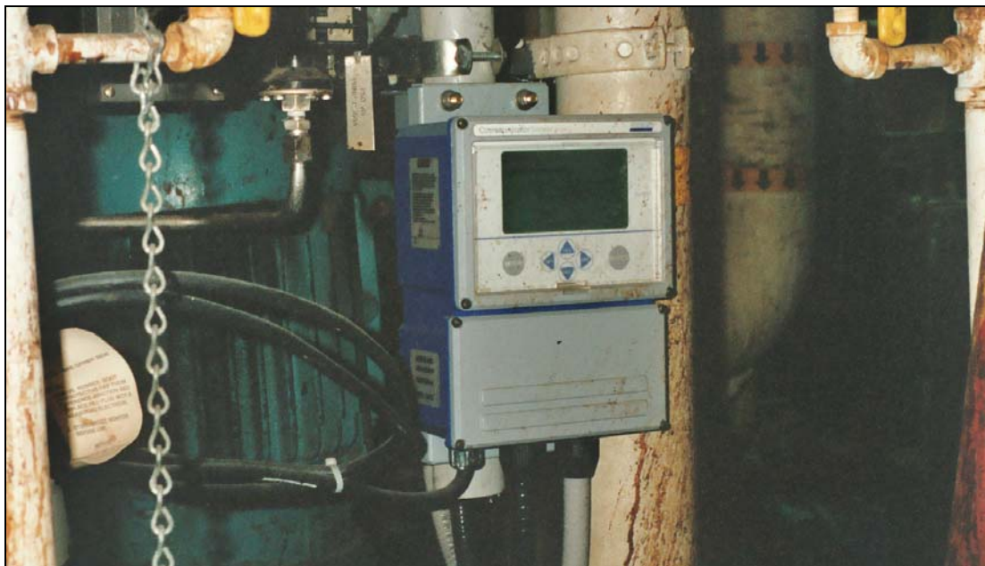
Figure 18. pH analyzer with high/low alarm outputs, Foxboro Model 875PH.
