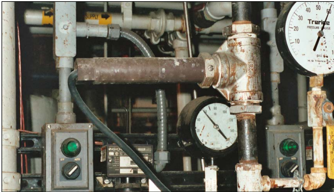
Figure 17. pH probe and cable in heat exchanger cooling line, Foxboro 871 series.
