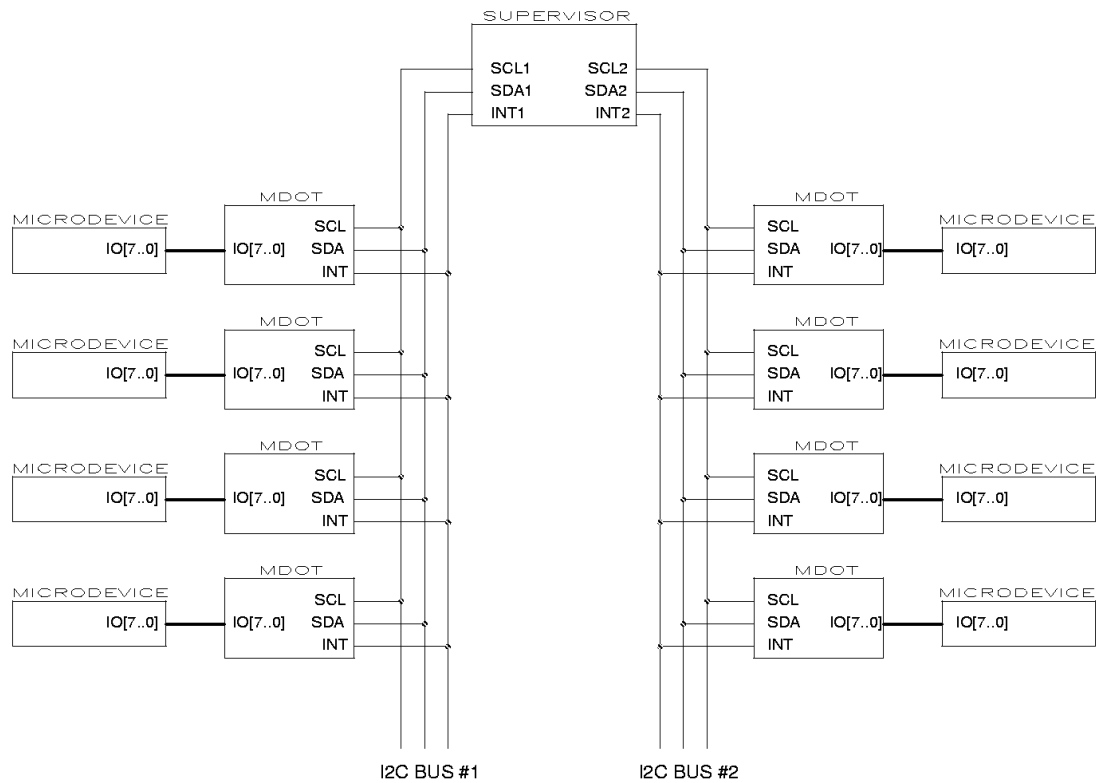
Figure 3-1. Microdot Distributed Computing Concept. Microdots are connected to the supervisor processor with the I 2 C bus. Each I 2 C bus can connect up to 128 Microdots.
