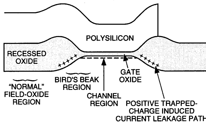
Figure 2-13. Bird's Beak Diagram. Positive charge buildup in the bird's beak region causes parasitic edge leakage [18]
