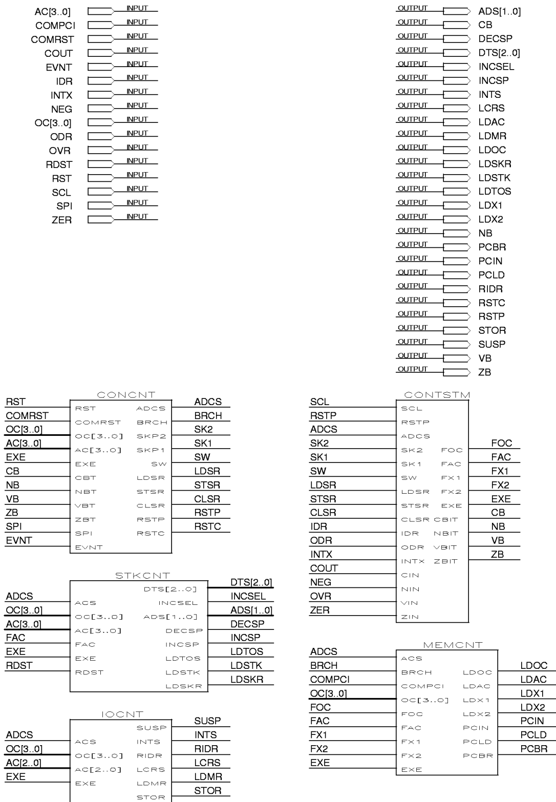
Figure 4-2. Control Unit Interconnect Diagram
