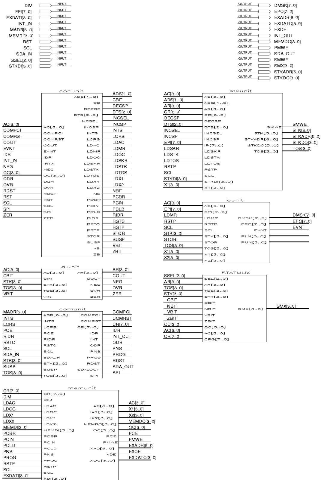
Figure 4-19. Microdot Interconnection Diagram
