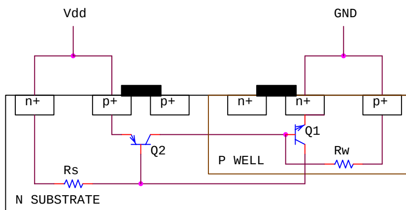
Figure 2-12. CMOS PNP Structure [10]
