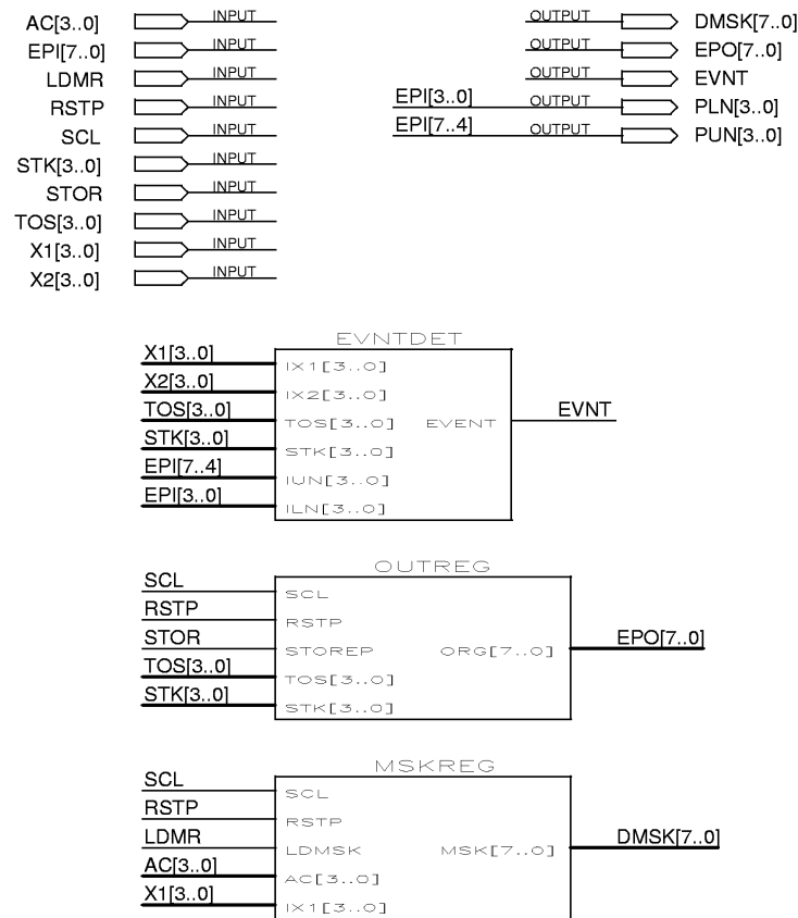
Figure 4-7. Input/Output Unit Interconnection Diagram
