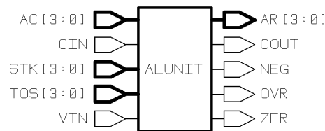
Figure 3-5. ALU Interface
