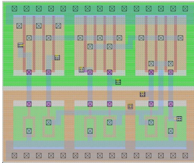
Figure 2-15. AOI222 (AND-OR-INVERT) gate in RHBD Gate Array
