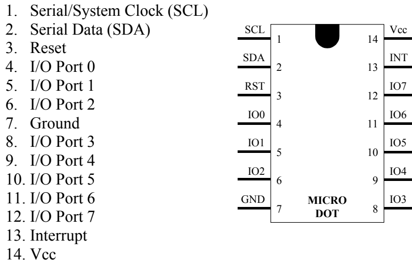
Figure 4-20. Microdot Production Version Pinout
