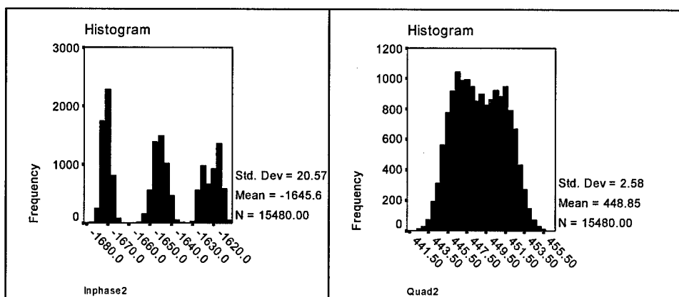
Figure 45. In-phase and quadrature histograms for 57-mm mortar at 150 Hz
