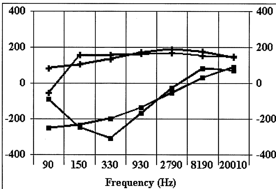
Figure 67. Calibration match with all frequencies for target 1-132 (57-mm mortar)
