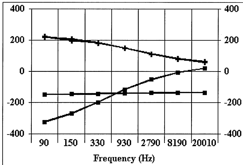
Figure 62. Best matching point for target 3-84 (81-mm mortar)
