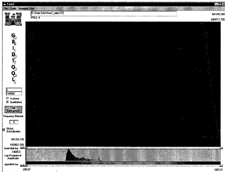
Figure A13. Area 1 quadrature coverage map for 8,190 Hz
