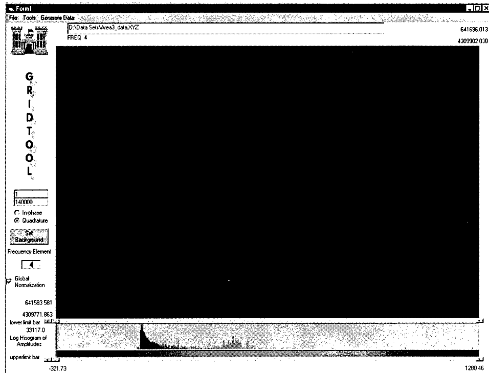
Figure A39. Area 3 quadrature coverage map for 930 Hz
